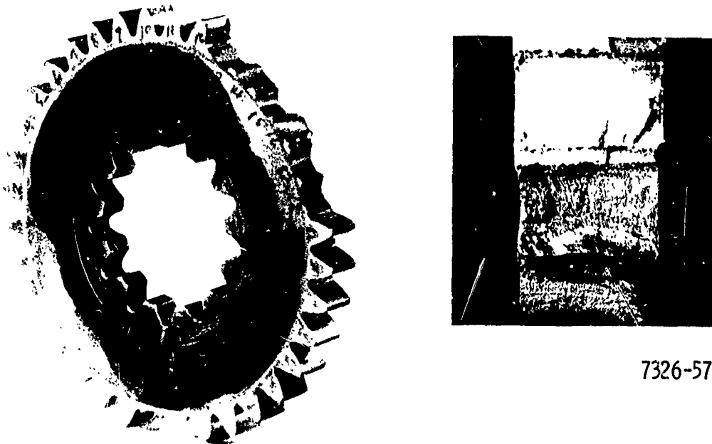
Figure 57. Fractured gear teeth induced by fatigue failure.
