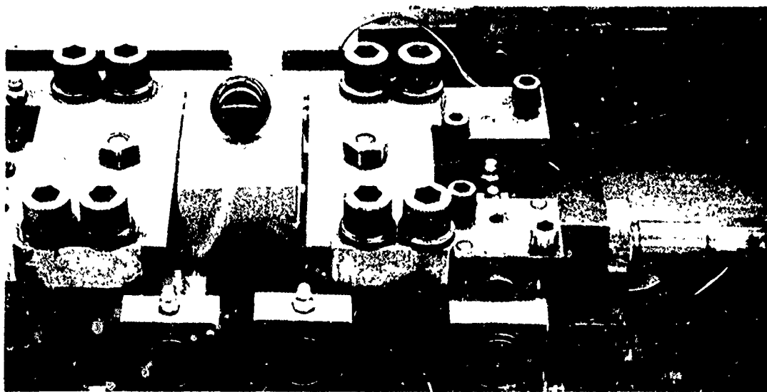
Figure 25. View of the Fretting Fatigue Fixture Showing the Assembly for 400° F Testing. Heated Air from a Tube Furnace is Blown into the Chamber (Lower Photograph) which Contains the Instrumented Specimen, Exposed in the Upper Photograph.
