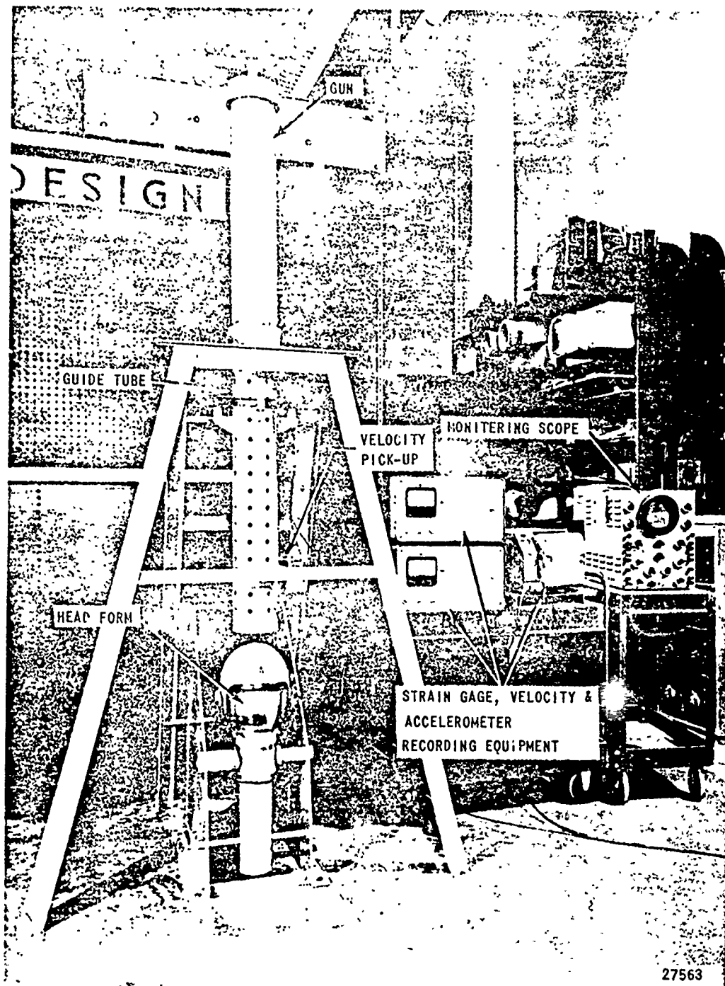
HELMET IMPACTOR
