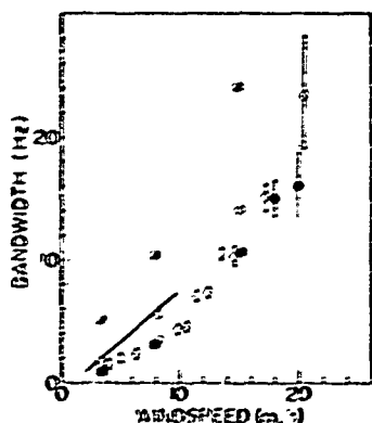
Fig. 12 — Dependence of bandwidth on windspeed at 9.375 GHz, 30° VV. The solid line is taken from Ref. 2, Fig. 8. The square data points are from Fig. 4. O, ● — fetch = 1 m; □ fetch = 1 m, □ fetch = 3.1 m, ■ fetch = 12 m.
