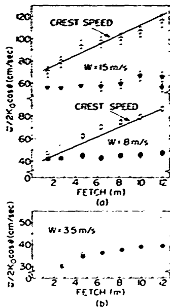
Fig. 8 — Fetch and windspeed dependence of mean wave speeds. (a) \nabla 9.375 GHz, 80° VV; \nabla 23.9 GHz, 50° VV; \square 23.9 GHz, 70° VV; \blacksquare 9.375 GHz, 30° VV. The solid lines are least mean squares linear fits to the measured crest speeds, (a) \circ 23.9 GHz, 70° VV; \bullet 9.375 GHz, 30° VV.
