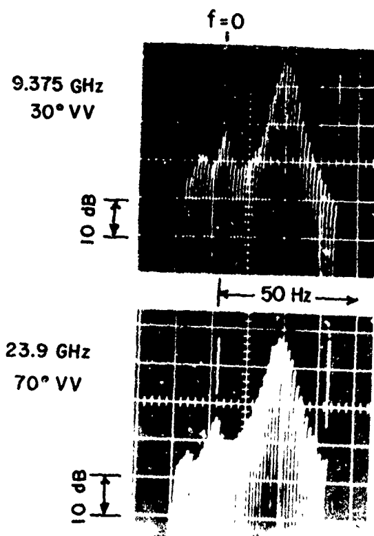
Fig. 4 — Doppler spectra in Bragg scattering. Windspeed = 3.5 m/s, fetch = 2.75 m, 2k_0 \cos\theta = 3.4 \text{ cm}^{-1} .
