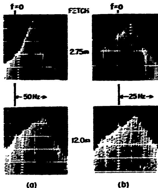
Fig. 7 — Doppler spectra at high angles. (a) 23.9 GHz, 70° VV, windspeed = 8 m/s, (b) 9.375 GHz, 90° VV, windspeed = 15 m/s
