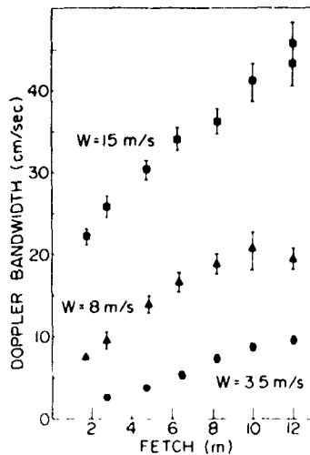
Fig. 6 -- Doppler bandwidth in velocity units, \Delta \omega / 2k_0 \cos \theta , as a function of fetch. ■ 23.9 GHz, 50° VV; ▲ 9.375 GHz, 30° VV; ● 9.375 GHz, 30° VV.
