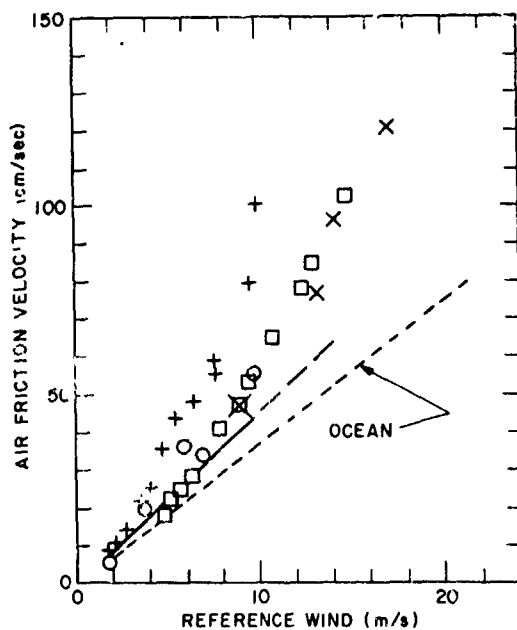
Fig. 2 — Air friction velocities as a function of reference wind for several wave tanks and the ocean. \circ — Shemdin (6); + — Kunishi (7); \square — Hidy and Plate (8); \times — this report.
