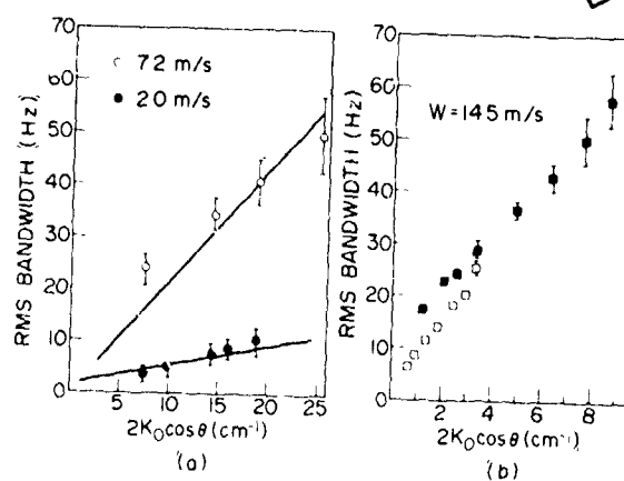
Fig. 5 — Doppler bandwidth on vertical polarization (a) 70.1 GHz, fetch = 3m, small tank. The solid lines are from Ref. 2, Fig. 7 (b) ■ 23.9 GHz, □ 9.375 GHz, fetch = 12 m, large tank.
