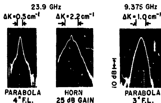
Fig. 3 — Fourier transforms of antenna patterns. The vertical scale is 10 dB/large division in each case. The horizontal scales vary. The width of the pattern 12 dB below the peak, \Delta K , is given in each case. The abbreviation F.L. means focal length.
