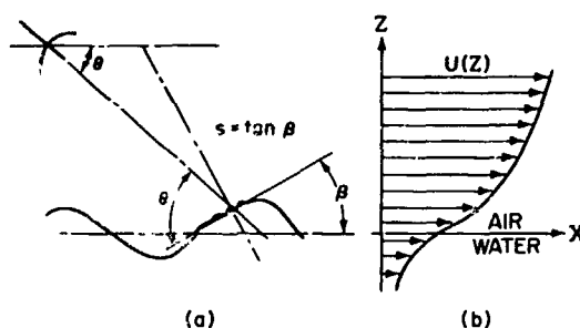
Fig. 1 — (a) Scattering geometry (b) Shear flow profile
