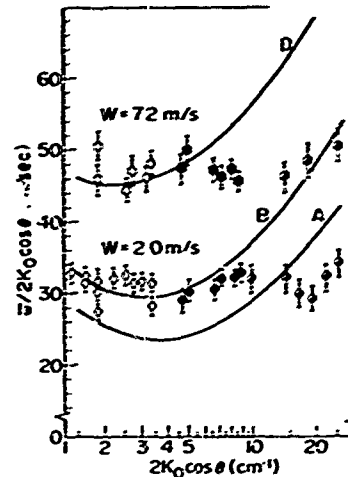
Fig. 13 — Dependence of mean wave speeds on Bragg wavenumber at fetch = 3.1 m. Open points, 9.375 GHz; solid points, 23.9 GHz; half-solid points, 70.1 GHz. Curve A is C_0(k) ; curve B is C(k) for U_s = 10 cm/sec, z_0^w = 0.01 cm, \alpha = 0 . Curve D is C(k) for U_s = 33 cm/sec, z_0^w = 0.01 cm, \alpha = 0 .
