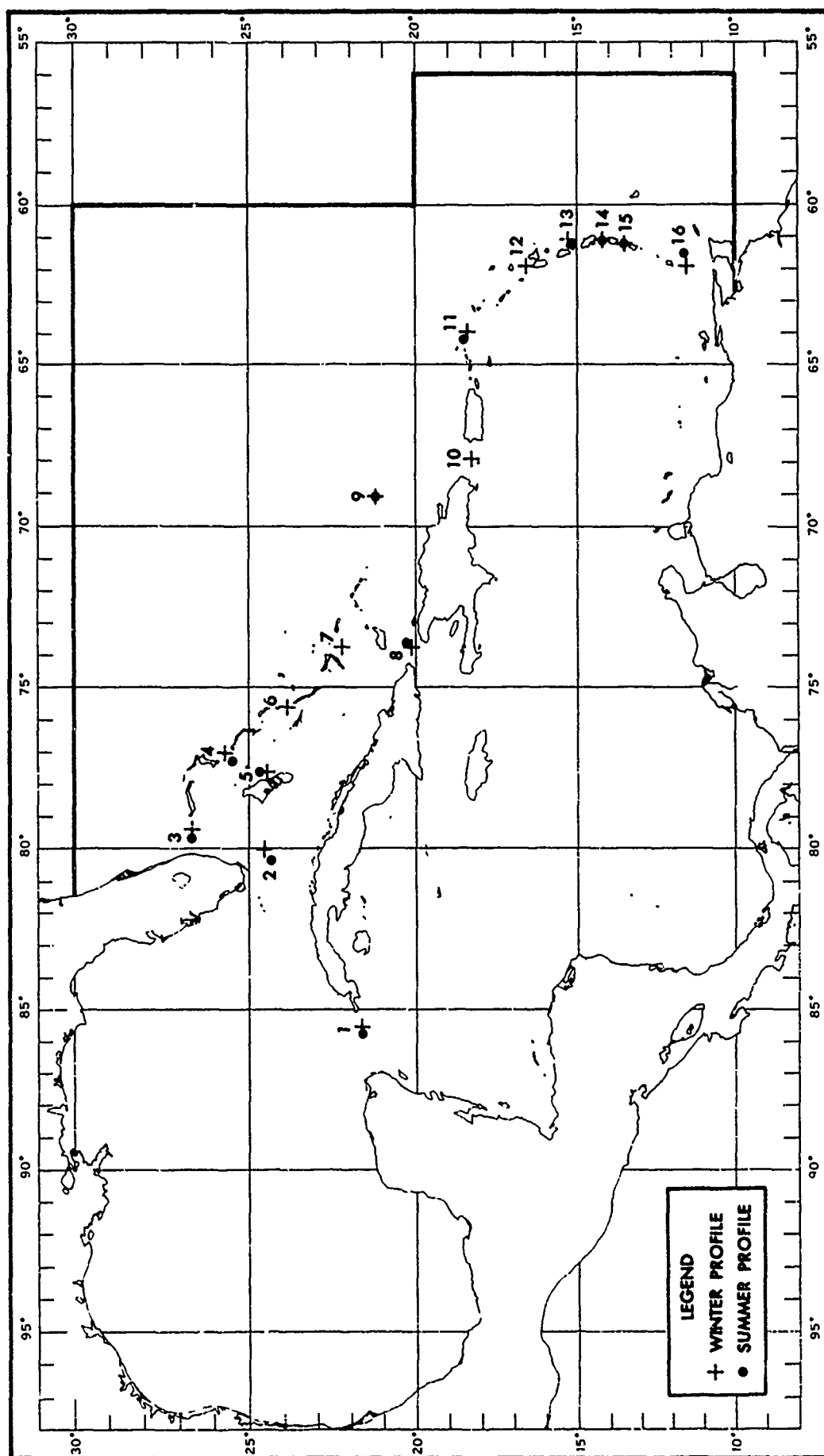
FIGURE 4-23 LOCATIONS OF SOUND VELOCITY PROFILES IN PRINCIPAL STRAITS
