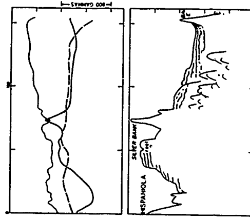
B. Reflection profiles north of Hispaniola.
