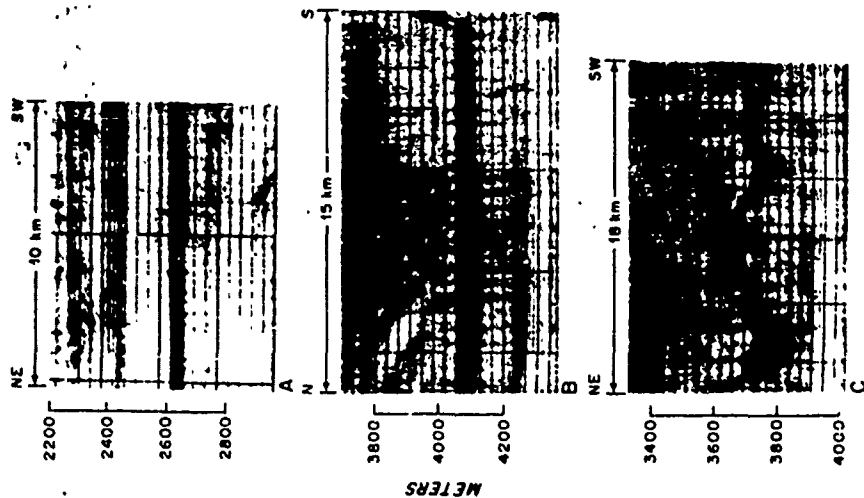
A. Typical 3.5 kHz echo-sounding traces displaying different types of sea bottom in southeastern Bahamas. A. Smooth, flat-bottom, no penetration; lack of penetration is probably due to coarse sediments. B. Smooth bottom with penetration. Strata probably consist of turbidites and pelagic sediments. This type of record is typical of most deeper sections of region. C. Irregular bottom made up of strongly reflecting material, possibly limestone, no penetration. For positions of records see B.
