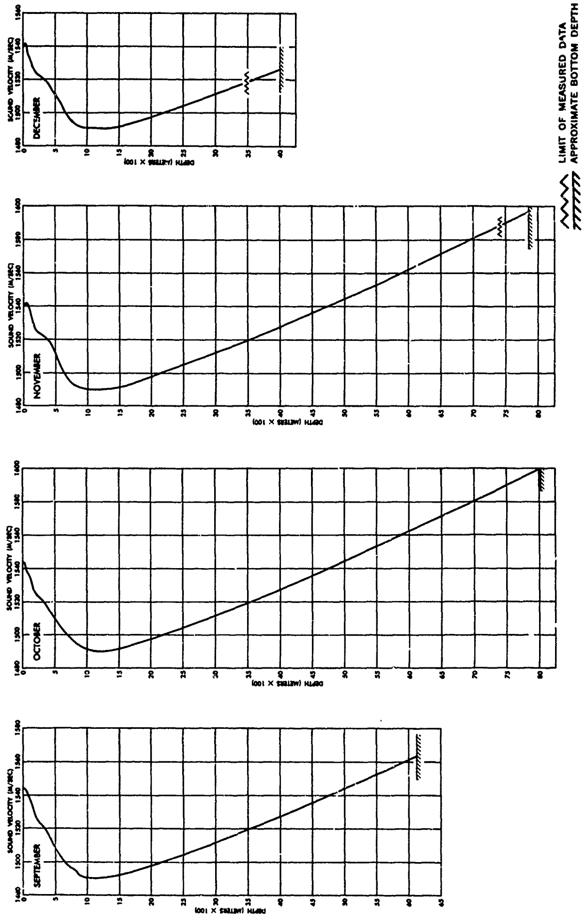
FIGURE 4-21 SOUND VELOCITY PROFILES-PUERTO RICO TRENCH (CONT.)
