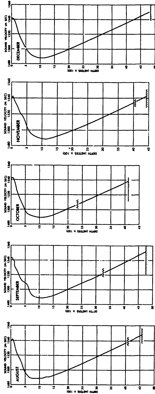
FIGURE 4-15 SOUND VELOCITY PROFILES-NORTH VENEZUELAN BASIN
