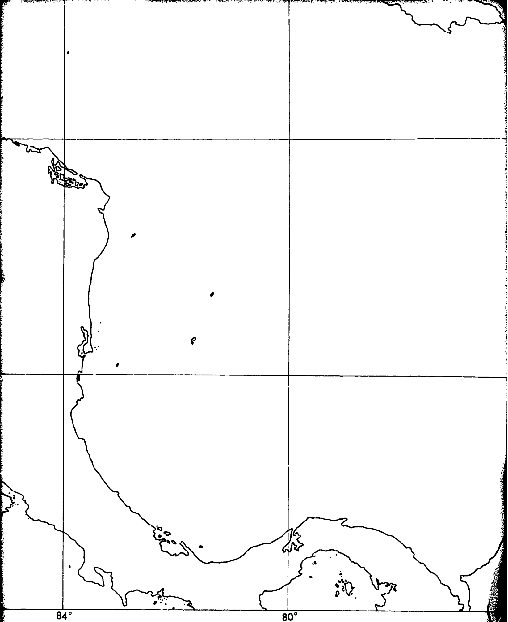
FIGURE 3-1 RESIDUAL MAGNETIC INTENSITY
