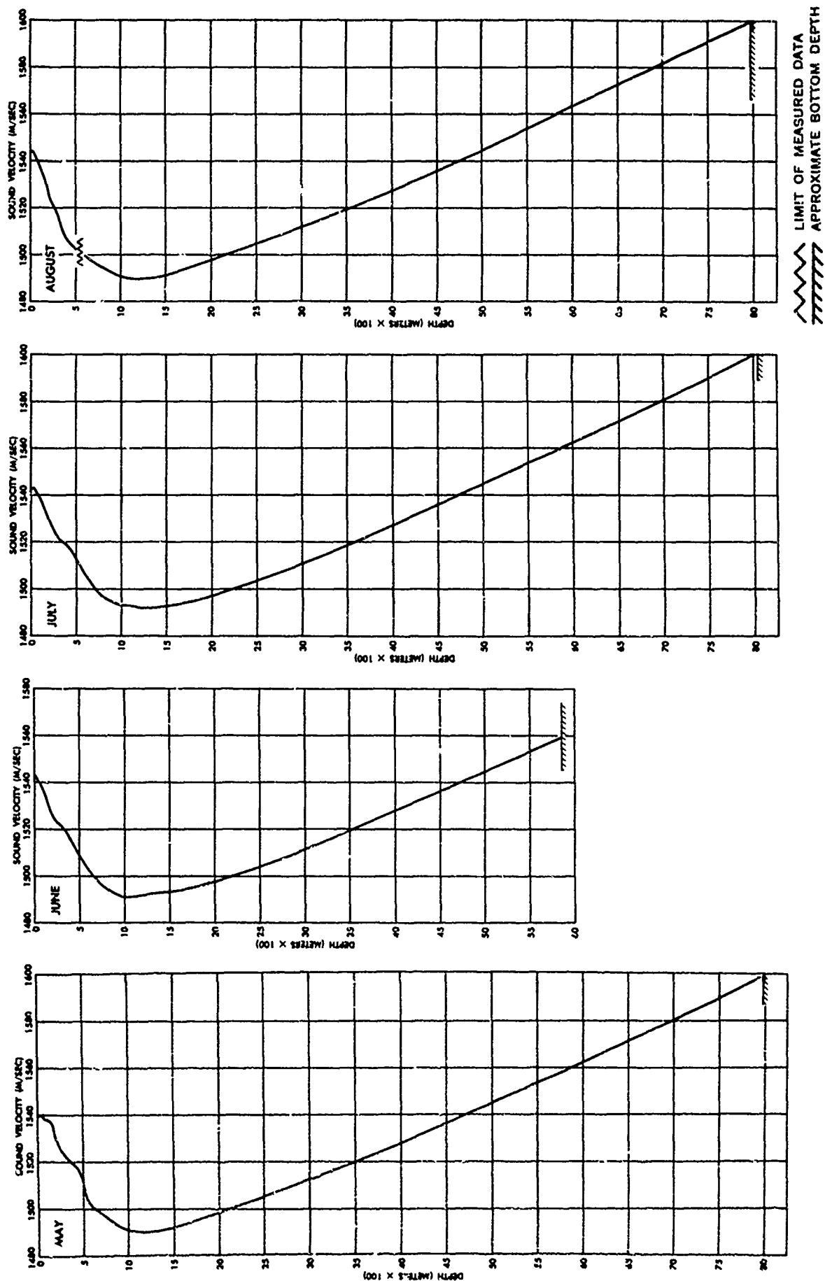
FIGURE 4-20 SOUND VELOCITY PROFILES-PUERTO RICO TRENCH (CONT.)
