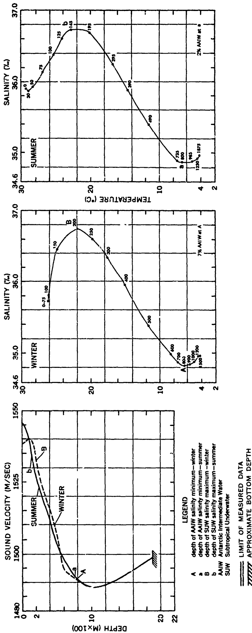
FIGURE 4-59 SOUND VELOCITY/TEMPERATURE-SALINITY COMPARISONS-YUCATAN CHANNEL
