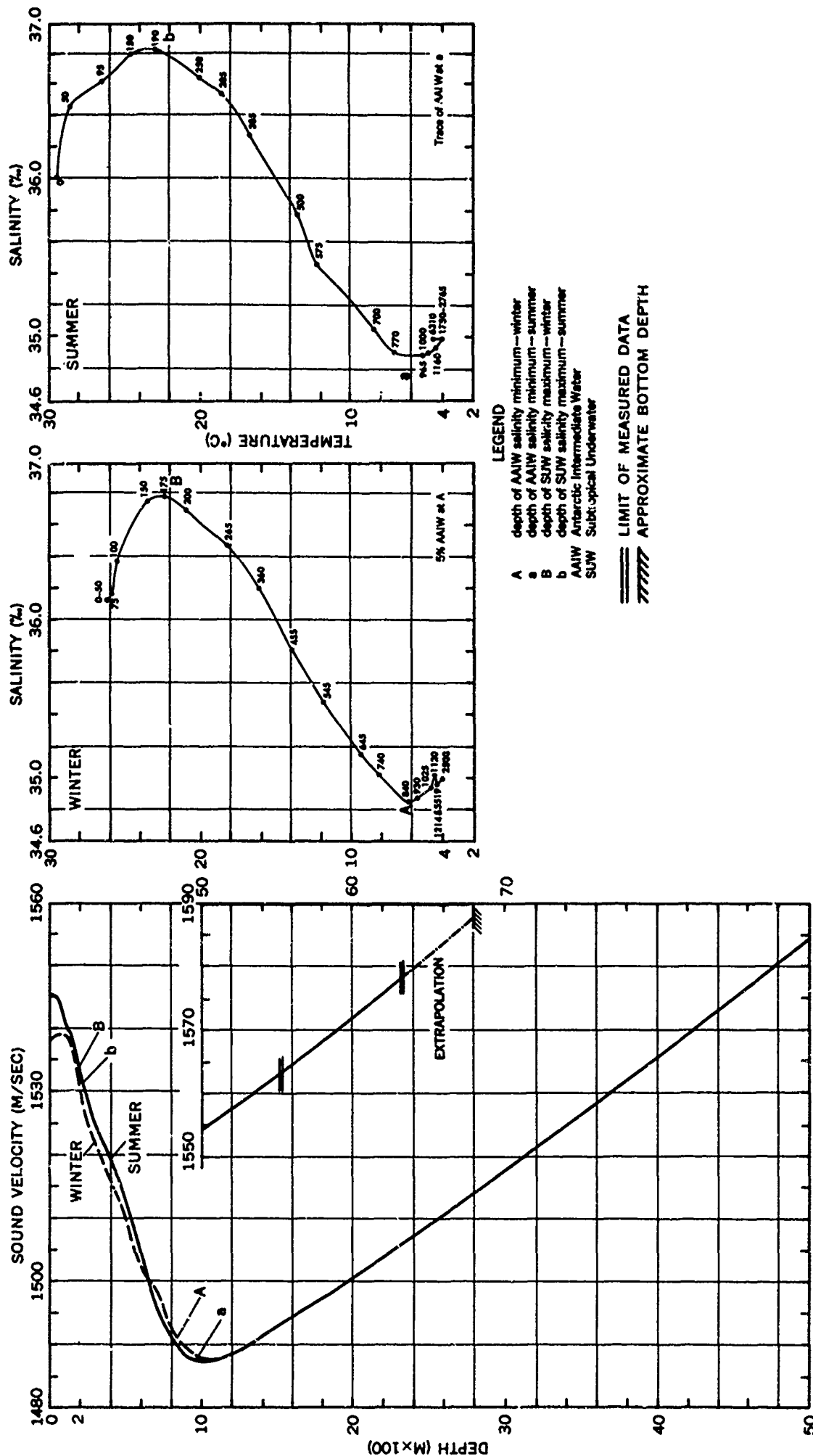
FIGURE 4-45 SOUND VELOCITY/TEMPERATURE-SALINITY COMPARISONS CAYMAN TROUGH
