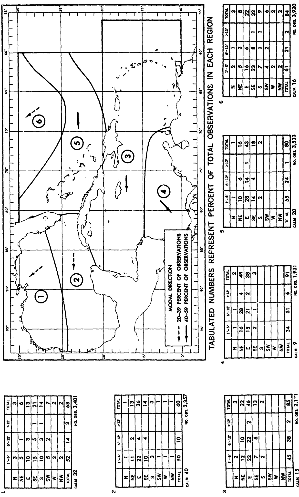
FIGURE 4-135 SUMMARIES OF OBSERVED SWELL HEIGHT AND DIRECTION-SUMMER (AUGUST)
