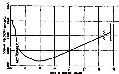
FIGURE 4-16 SOUND VELOCITY PROFILES-SOUTH VENEZUELAN BASIN
