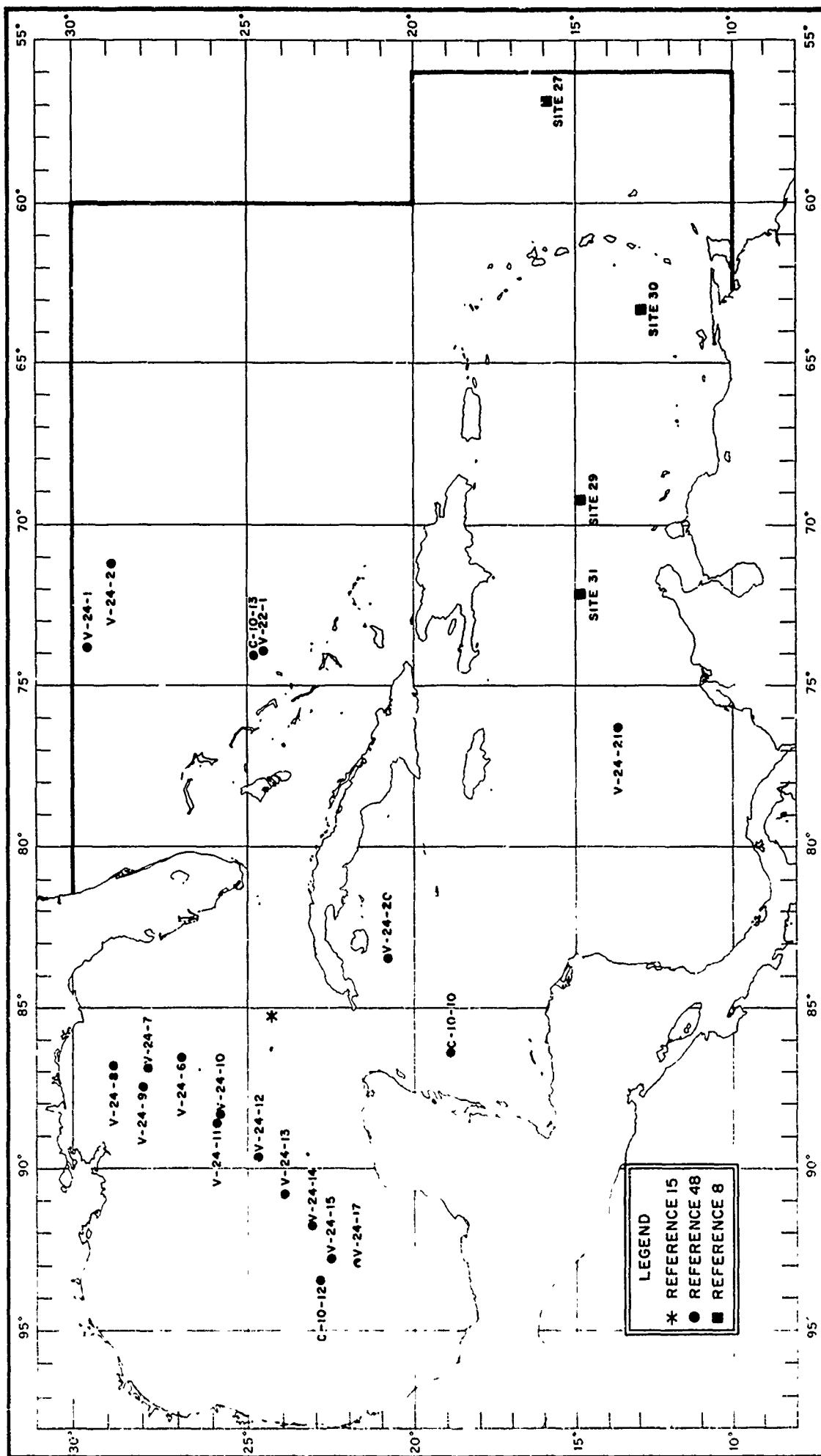
FIGURE 4-123 LOCATIONS OF SEDIMENT VELOCITY STATIONS
