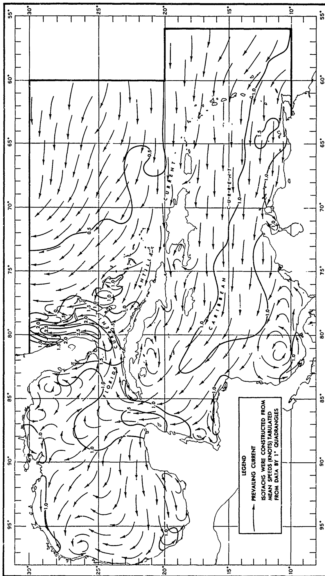
FIGURE 4-137 PREVAILING SURFACE CURRENT PATTERNS-WINTER (JANUARY-MARCH)
