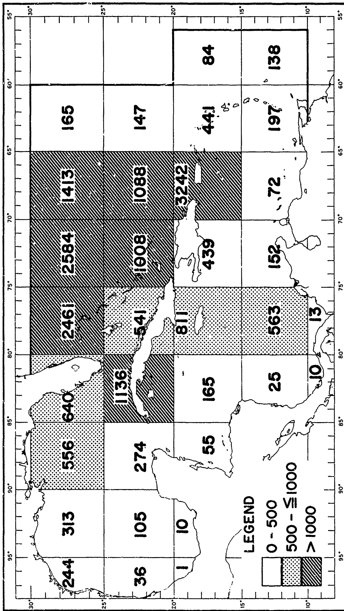
FIGURE 4-5 DISTRIBUTION OF BATHYTHERMOGRAPHS (WINTER)
