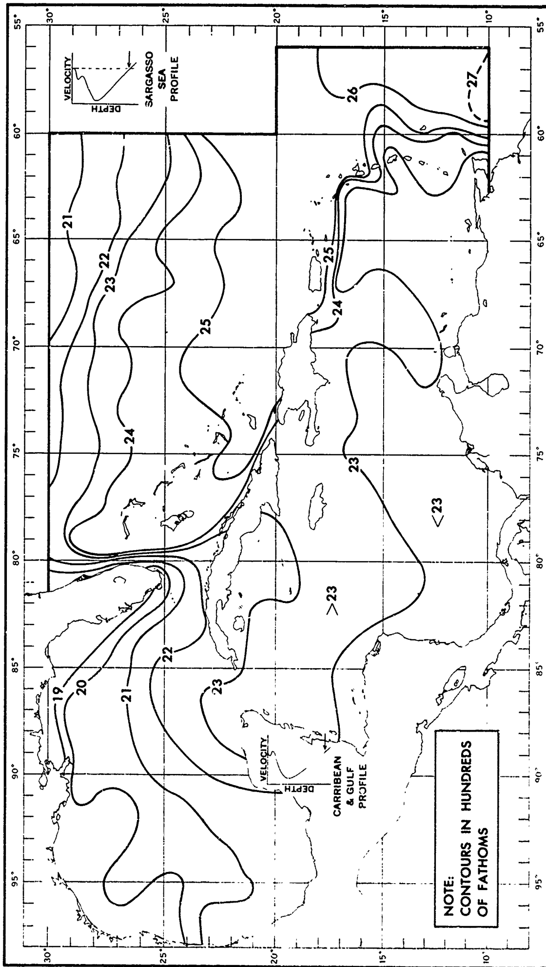
FIGURE 4-91 AVERAGE CRITICAL DEPTH (WINTER, NOVEMBER-APRIL)
