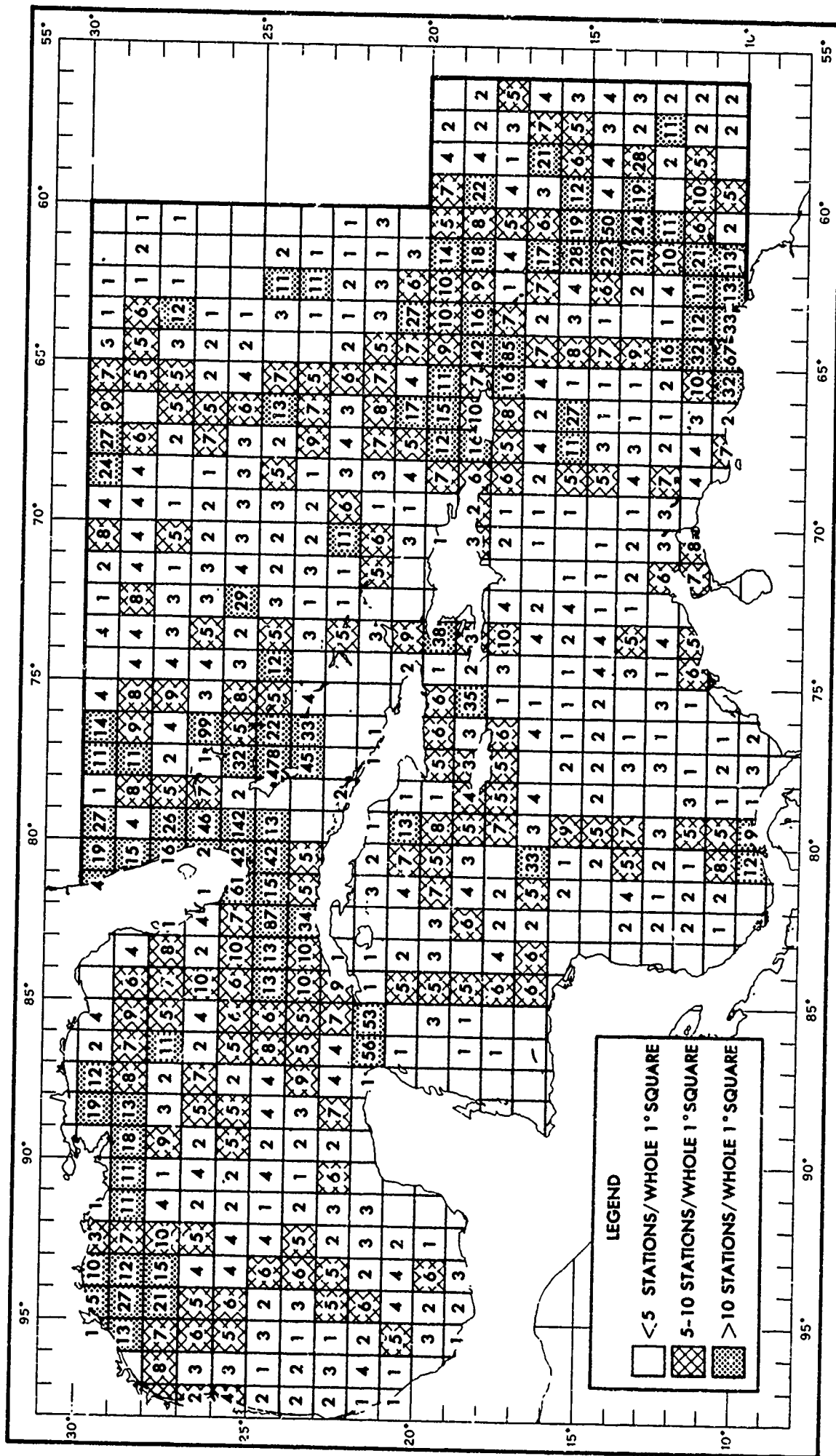
FIGURE 4-2 DISTRIBUTION OF OCEAN STATIONS AND SOUND VELOCIMETER MEASUREMENTS (WINTER, NOVEMBER-APRIL)
