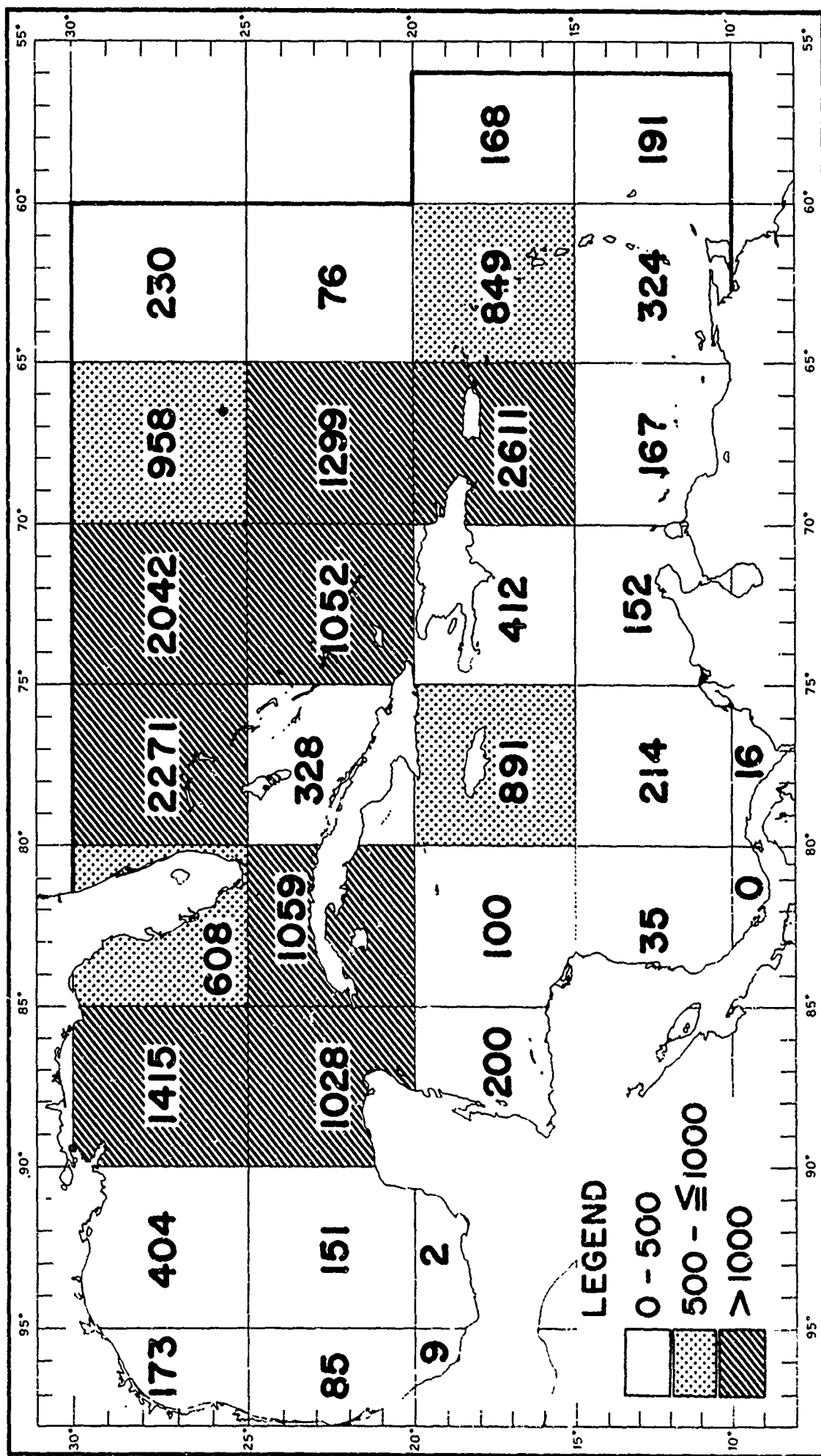
FIGURE 4-6 DISTRIBUTION OF BATHYTHERMOGRAPHS (SUMMER)
