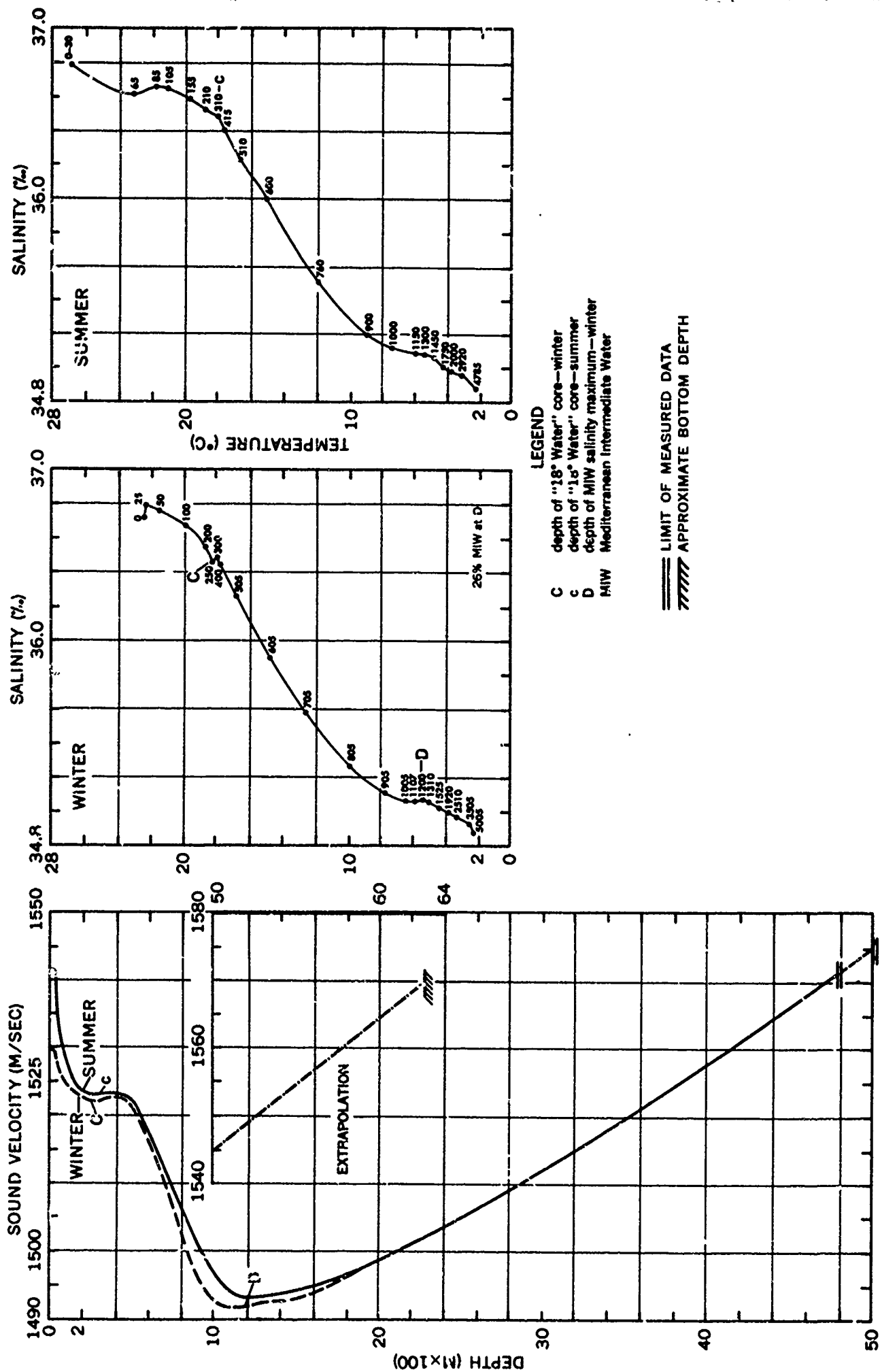
FIGURE 4-41 SOUND VELOCITY/TEMPERATURE-SALINITY COMPARISONS-NORTH AMERICAN BASIN
