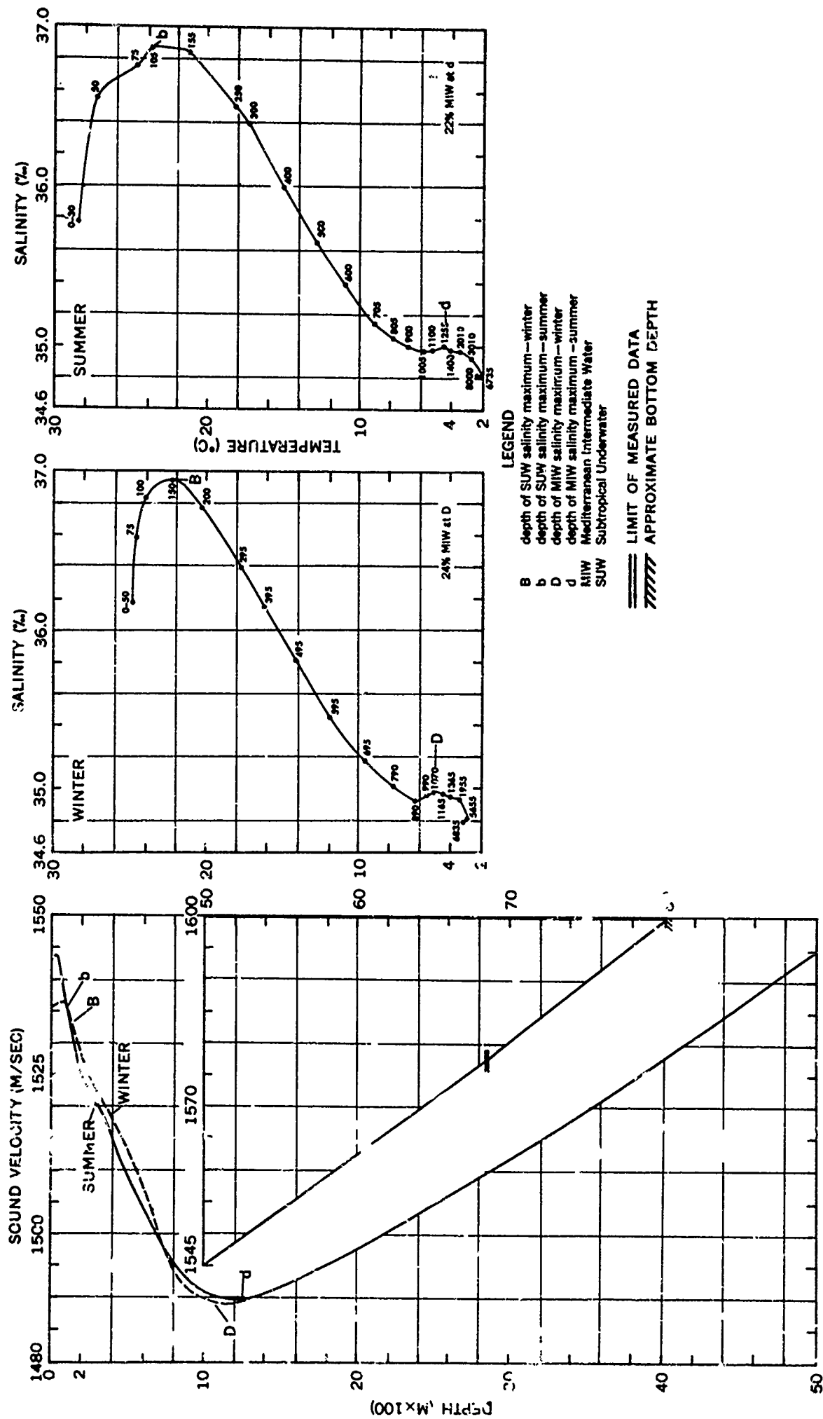
FIGURE 4-46 SOUND VELOCITY/TEMPERATURE-SALINITY COMPARISONS-PUERTO RICO TRENCH
