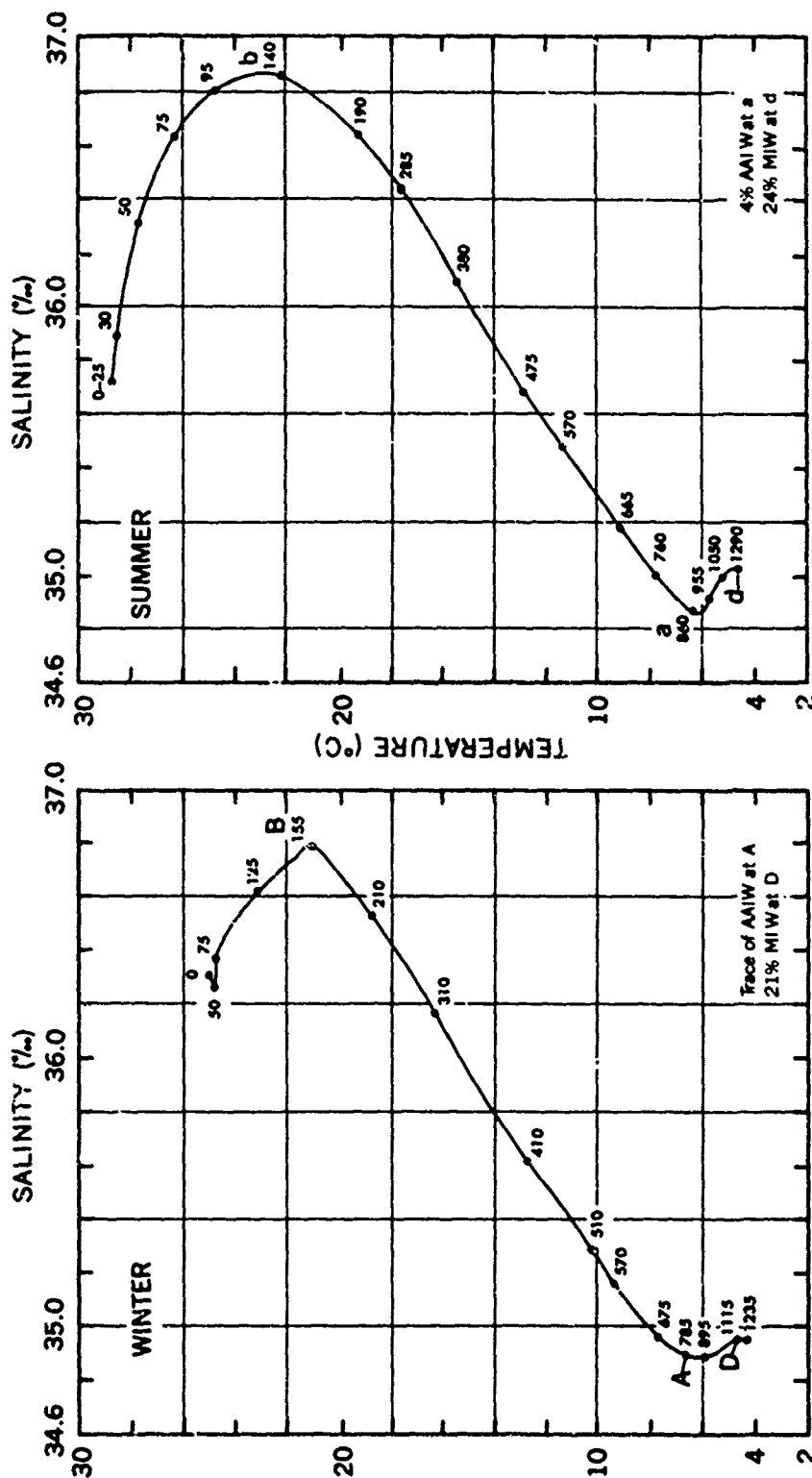
FIGURE 4-63 SOUND VELOCITY/TEMPERATURE-SALINITY COMPARISONS-ANEGADA PASSAGE
