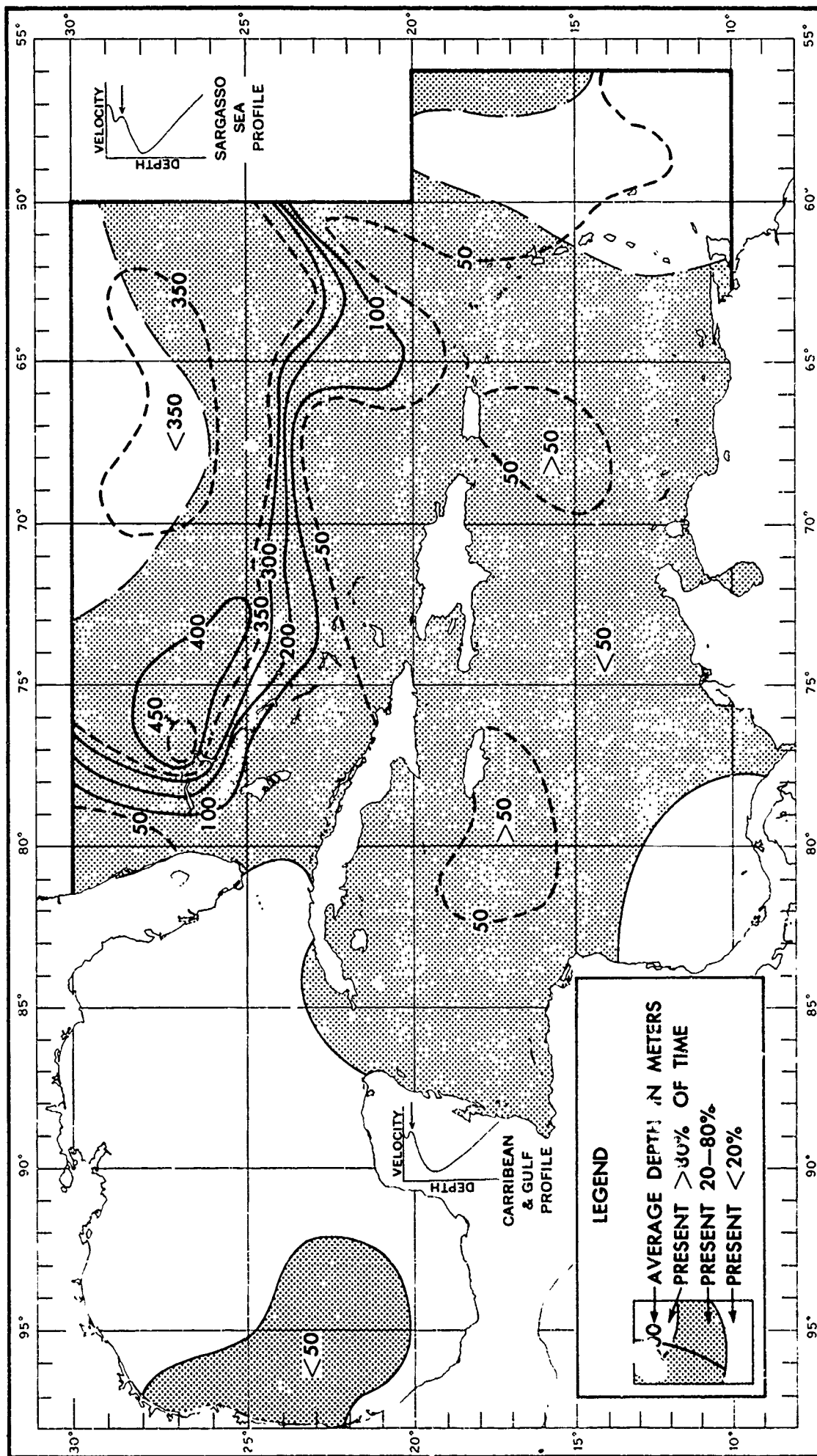
FIGURE 4-72 EXTENT AND AVERAGE DEPTH OF THE SUBSURFACE SOUND VELOCITY MAXIMUM (APRIL-JUNE)
