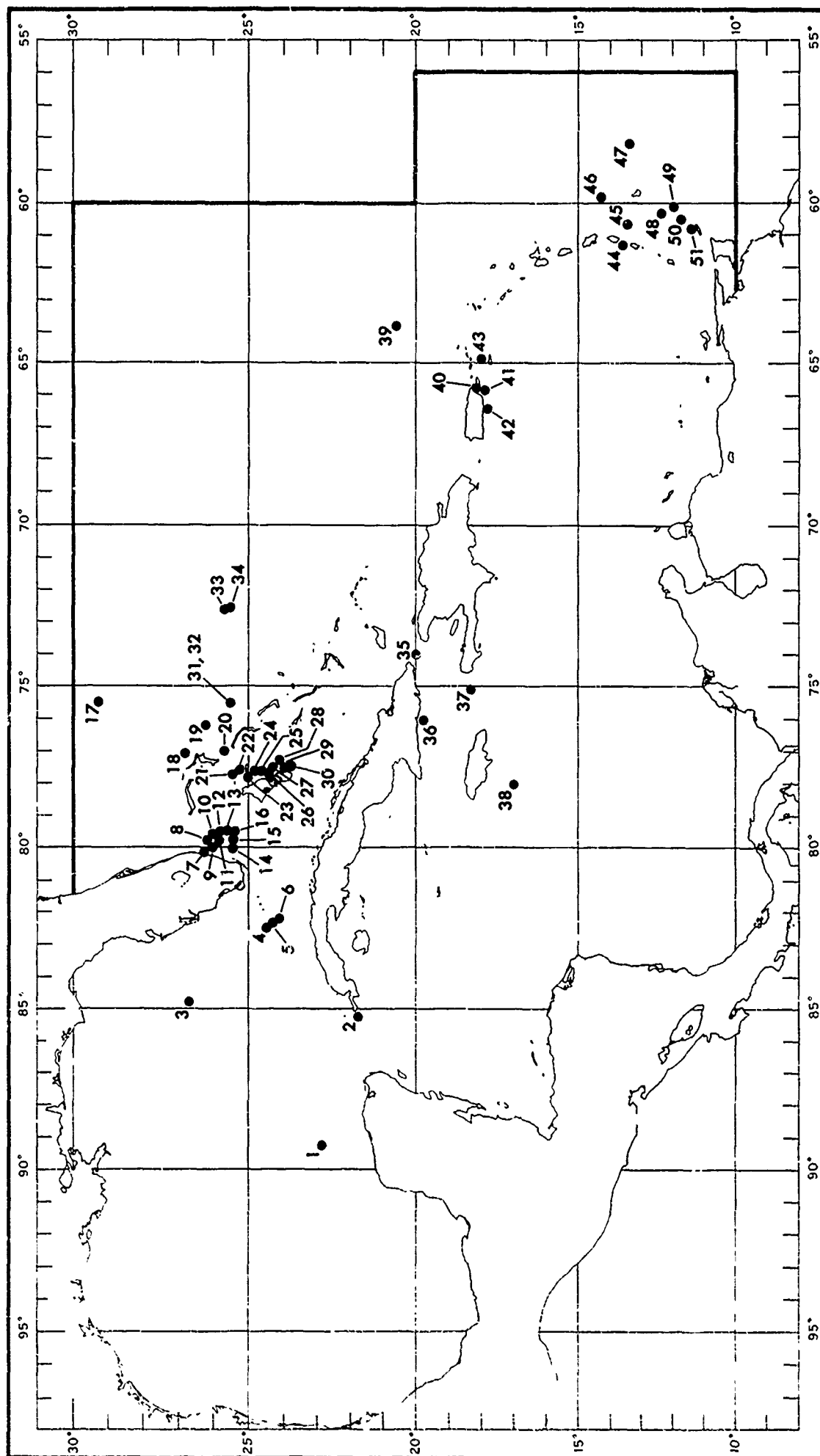
FIGURE 4-149 LOCATIONS OF SUBSURFACE CURRENT PROFILES
