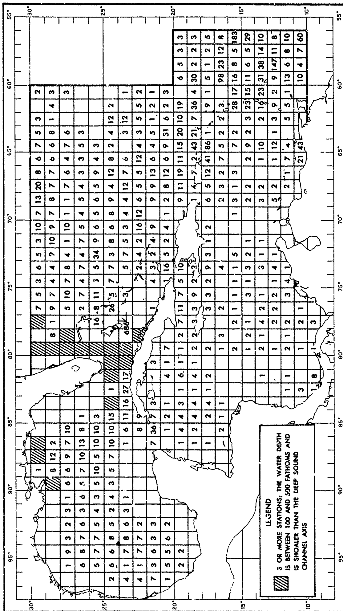
FIGURE 4-4 DISTRIBUTION OF OCEAN STATIONS AND SOUND VELOCIMETER MEASUREMENTS DEEPER THAN AXIAL DEPTH
