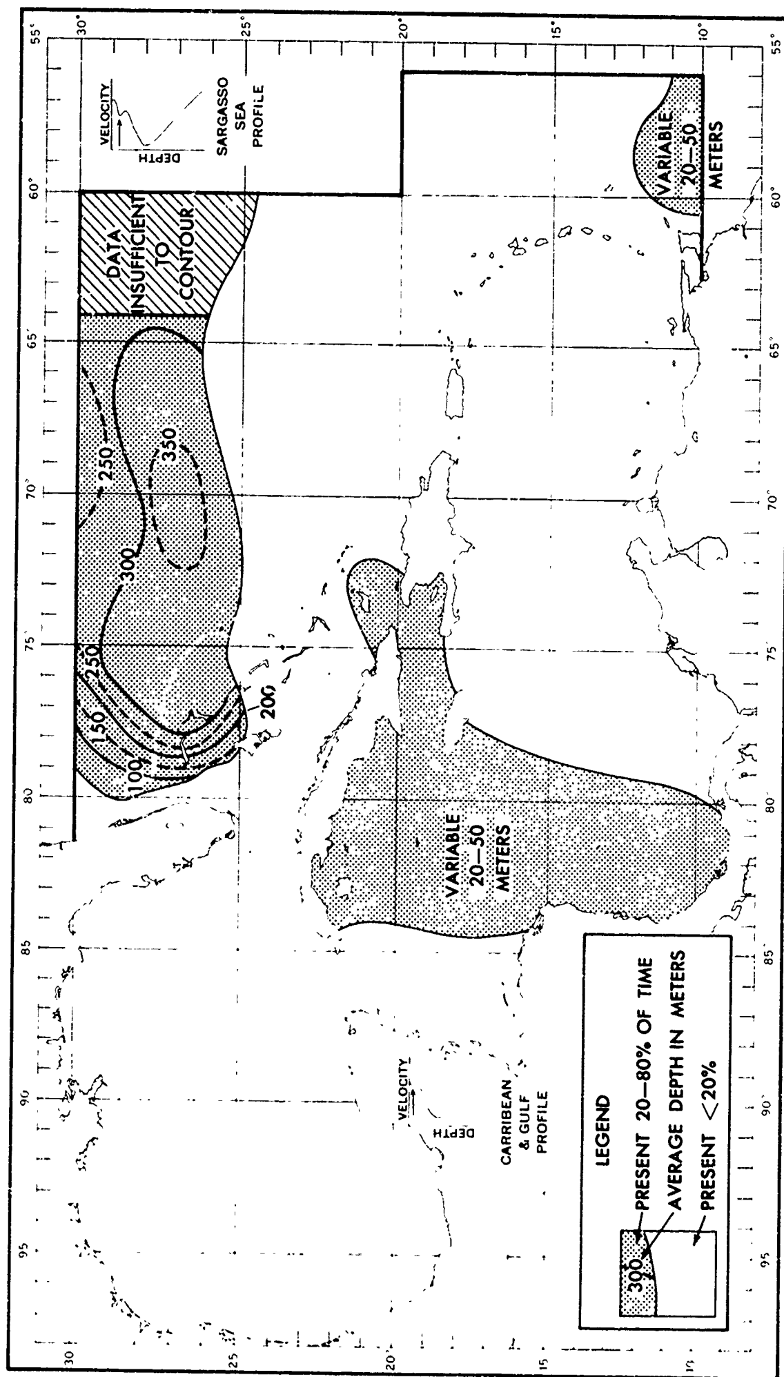
FIGURE 4-67 EXTENT AND AVERAGE DEPTH OF THE SUBSURFACE (SECONDARY) SOUND VELOCITY MINIMUM (JANUARY-MARCH)
