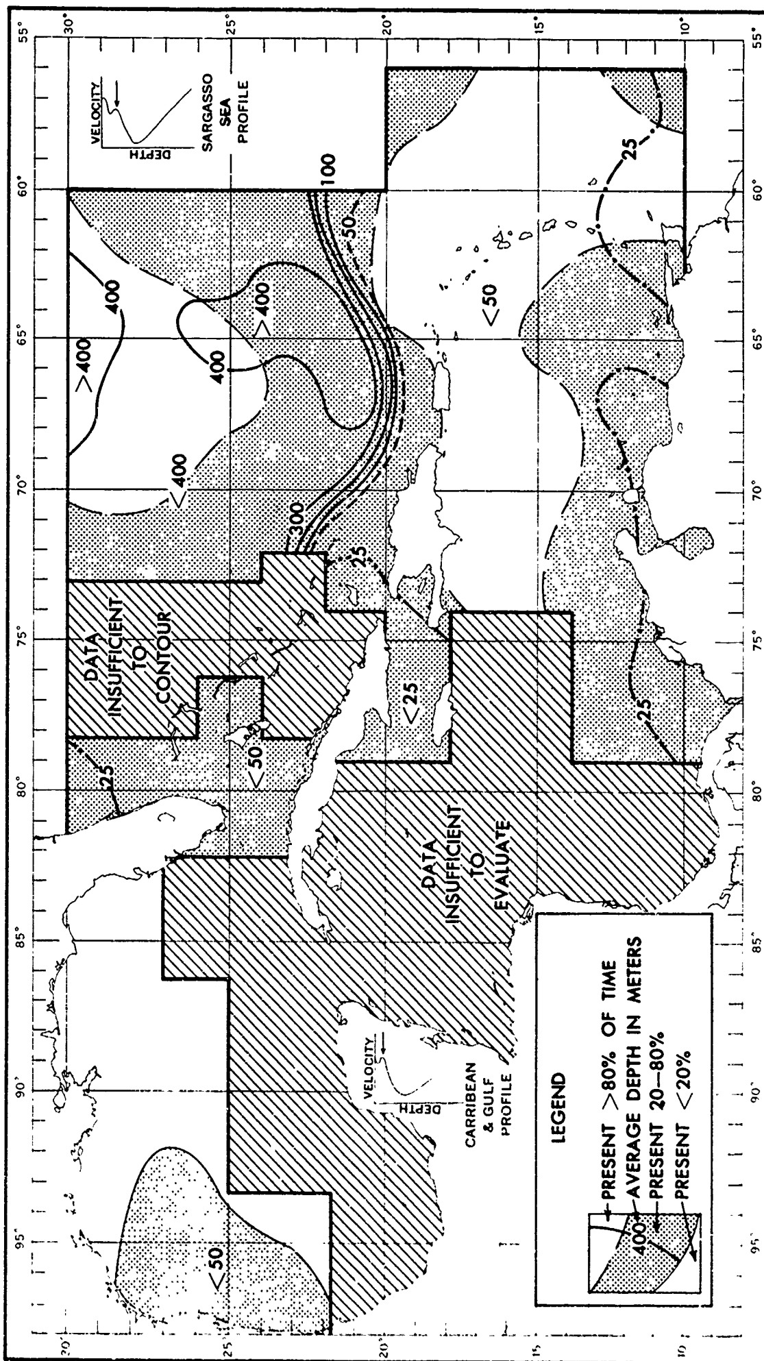
FIGURE 4-73 EXTENT AND AVERAGE DEPTH OF THE SUBSURFACE SOUND VELOCITY MAXIMUM (JULY-SEPTEMBER)
