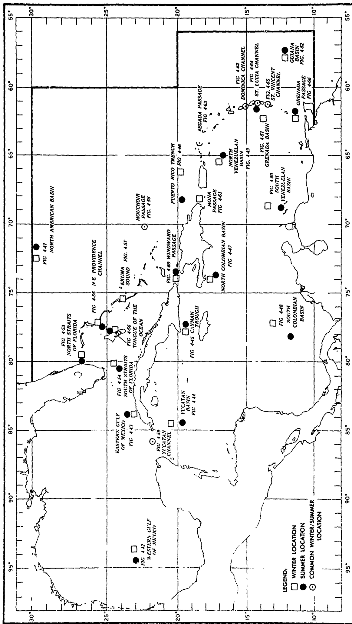
FIGURE 4-40 LOCATIONS OF SOUND VELOCITY/TEMPERATURE-SALINITY COMPARISONS
