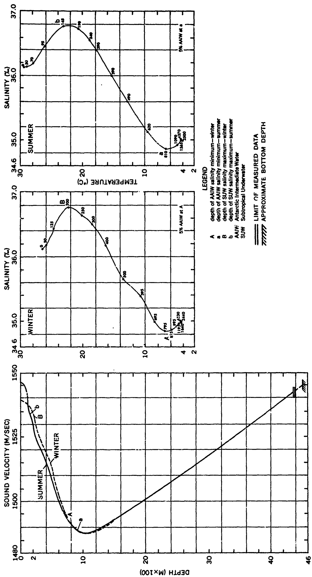
FIGURE 4-44 SOUND VELOCITY/TEMPERATURE-SALINITY COMPARISONS- YUCATAN BASIN
