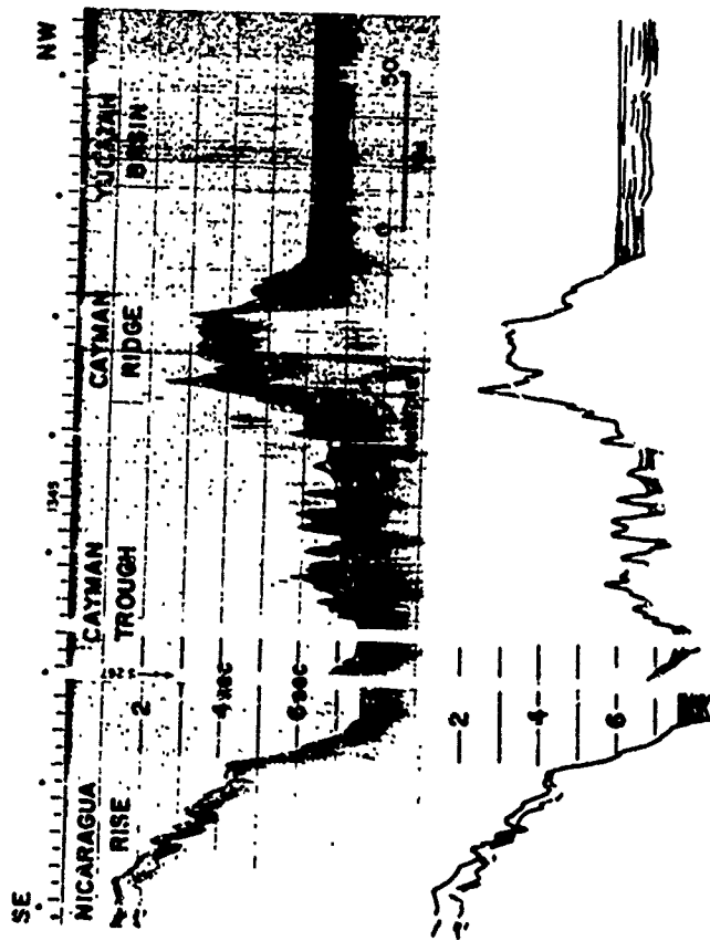
A. Profiler record across Yucatan Basin from Nicaragua Rise (airgun, C-10).
