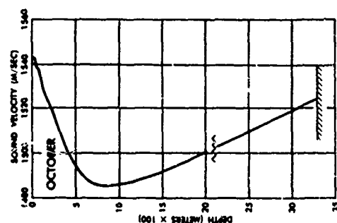
FIGURE 4-16 SOUND VELOCITY PROFILES-SOUTH VENEZUELAN BASIN
