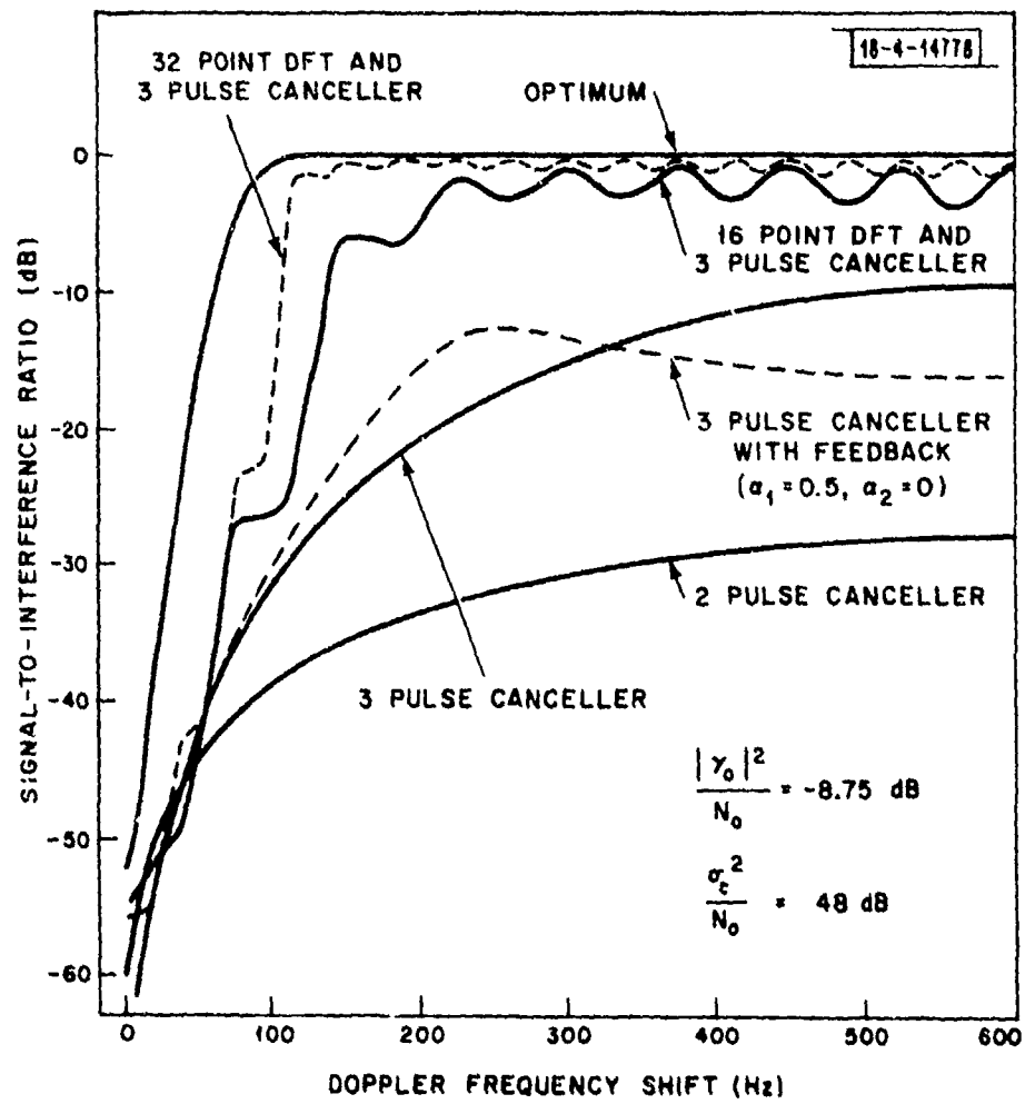
Figure 1. Signal-to-interference ratio for several practical MTI processors.
