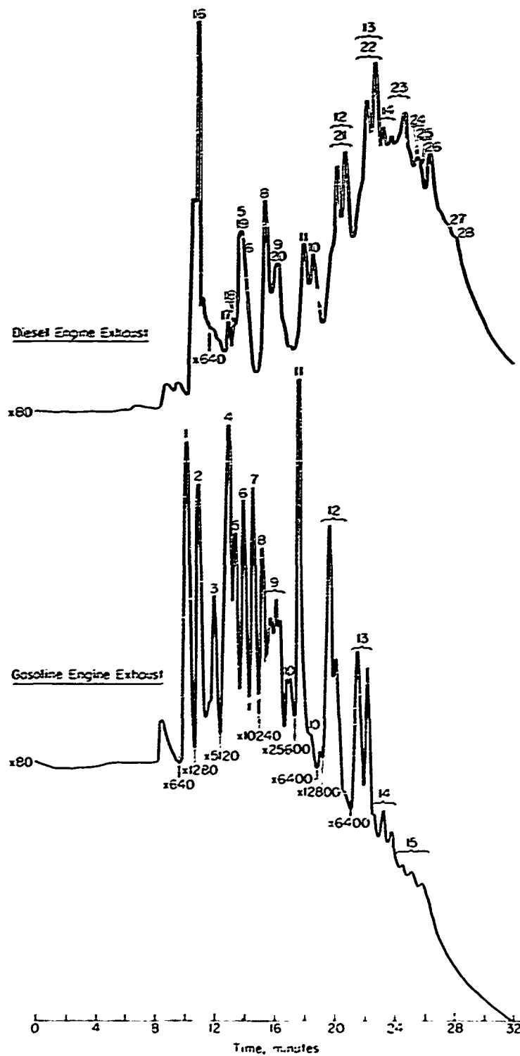
Figure 19. Typical chromatograms of organic fraction of vehicle exhaust collected under field conditions.
