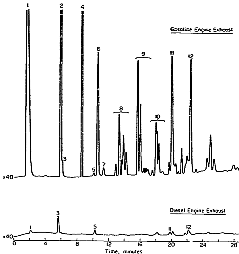
Figure 20. Typical chromatograms of organic fraction of vehicle exhaust obtained by direct injection.
