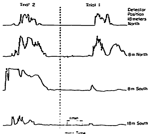
Figure 17. Typical response of condensation nuclei detectors located on both sides of vehicle path of travel in wooded terrain.
