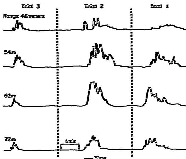
Figure 18. Typical response of condensation nuclei detectors arranged at different downwind distances in wooded terrain.
