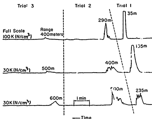
Figure 12. Typical responses of condensation nuclei detectors to M123 10-ton diesel truck operating in open terrain with 10-mph wind speed.
