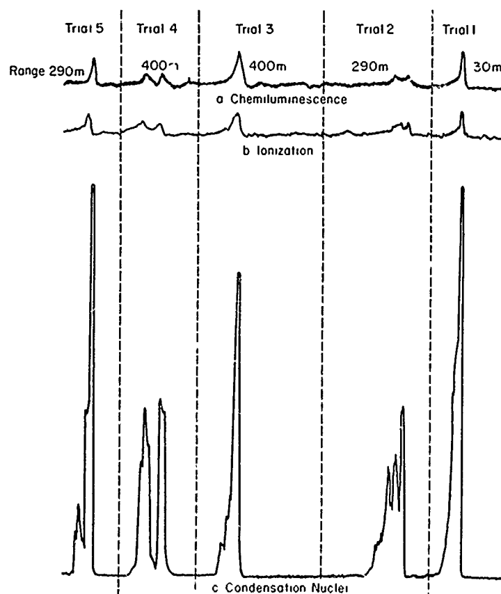
Figure 13. Comparison of responses from chemiluminescence monitor, and Honeywell ionization and condensation nuclei detectors in open terrain.
