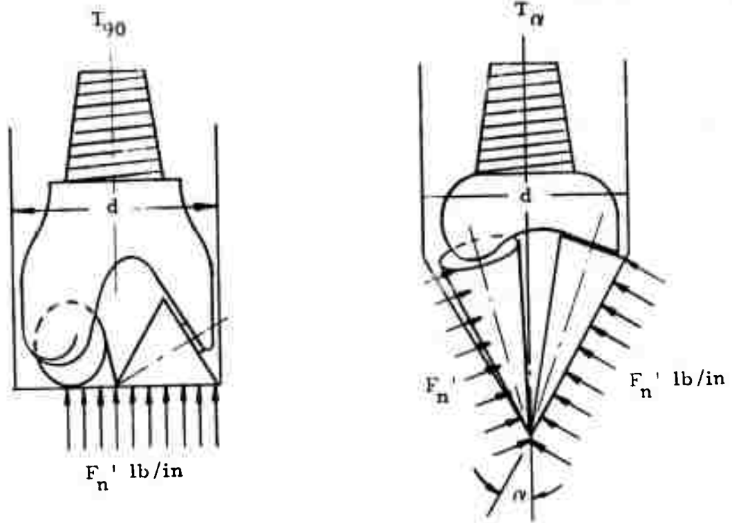
(b) Conical ( \alpha ) Bit
