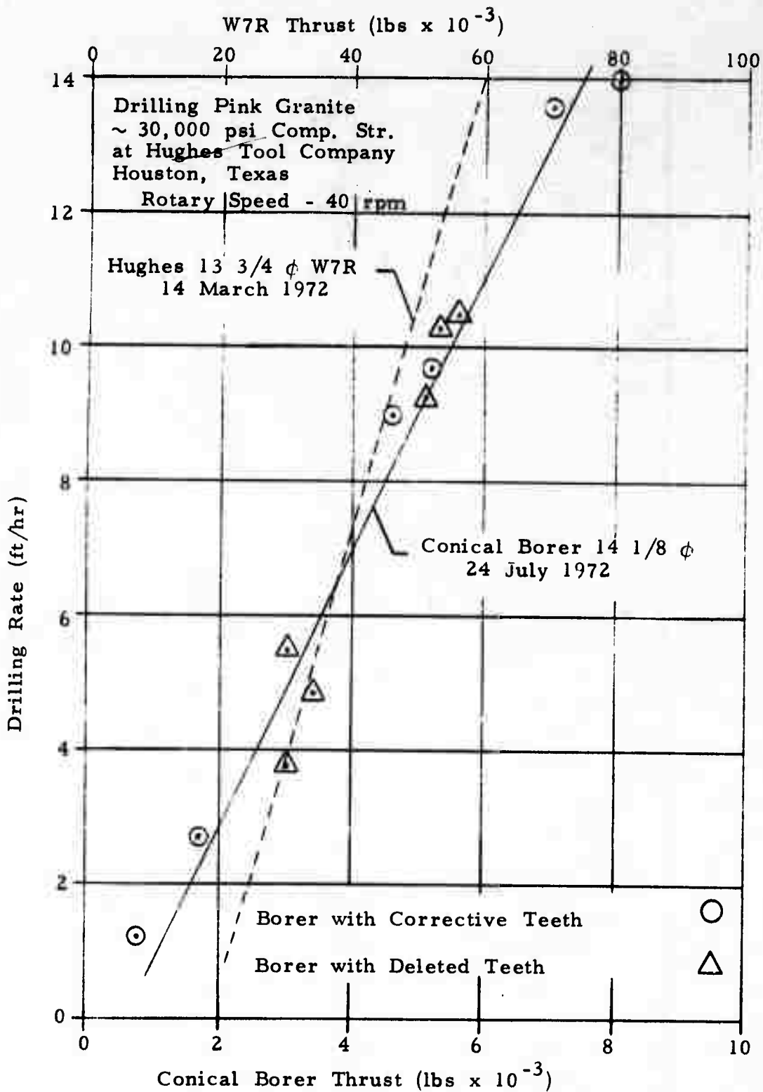
Thrust vs. Drilling Rate for the Nose Section Prototype Conical Borer
