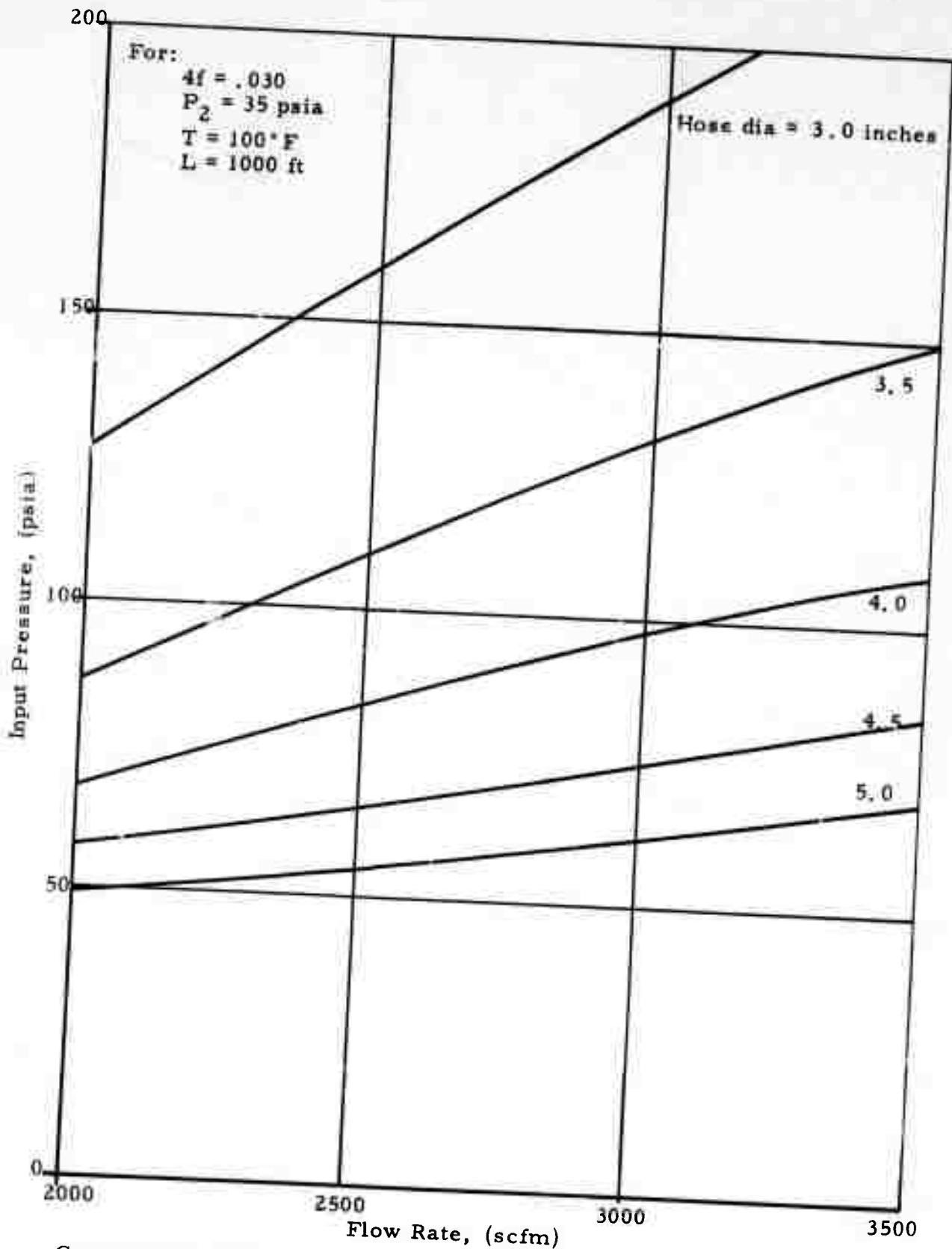
Compressor Input Pressure versus Flow Rate for Various Hose Sizes Figure 25
