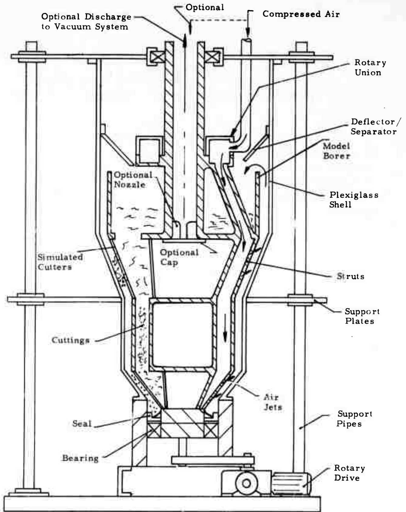
Schematic of Mucking System Model
