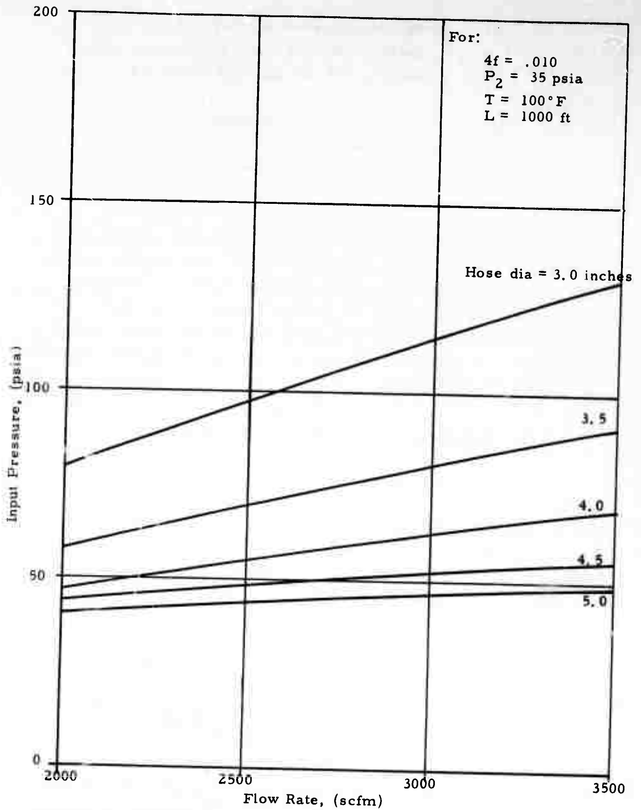
Compressor Input Pressure versus Flow Rate for Various Hose Sizes
