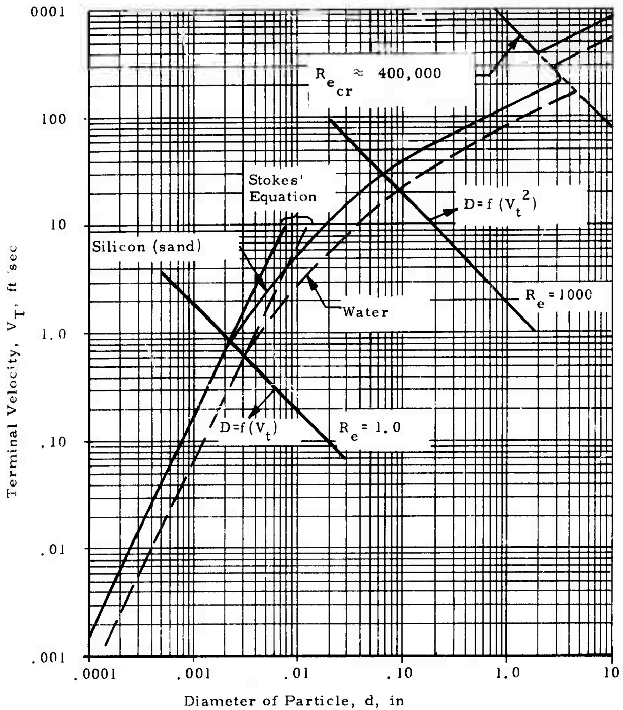
Terminal Velocity of Particles vs. Particle Diameter (7)
