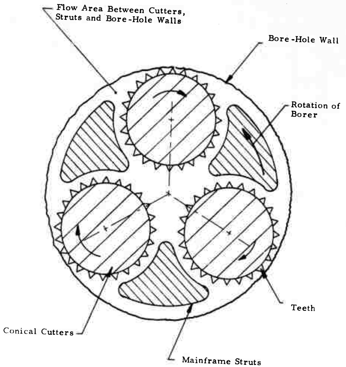
Typical Configuration of Flow Paths in the Area of the Conical Cutters
