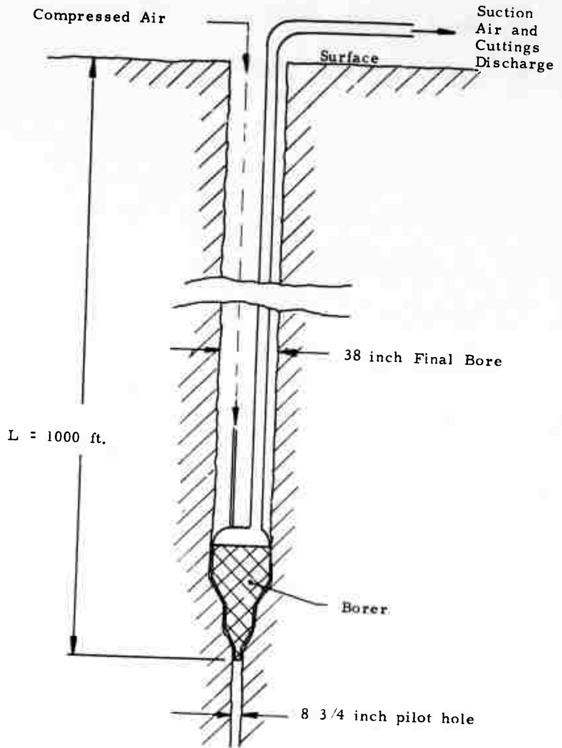
Schematic of Pneumatic Transport System
