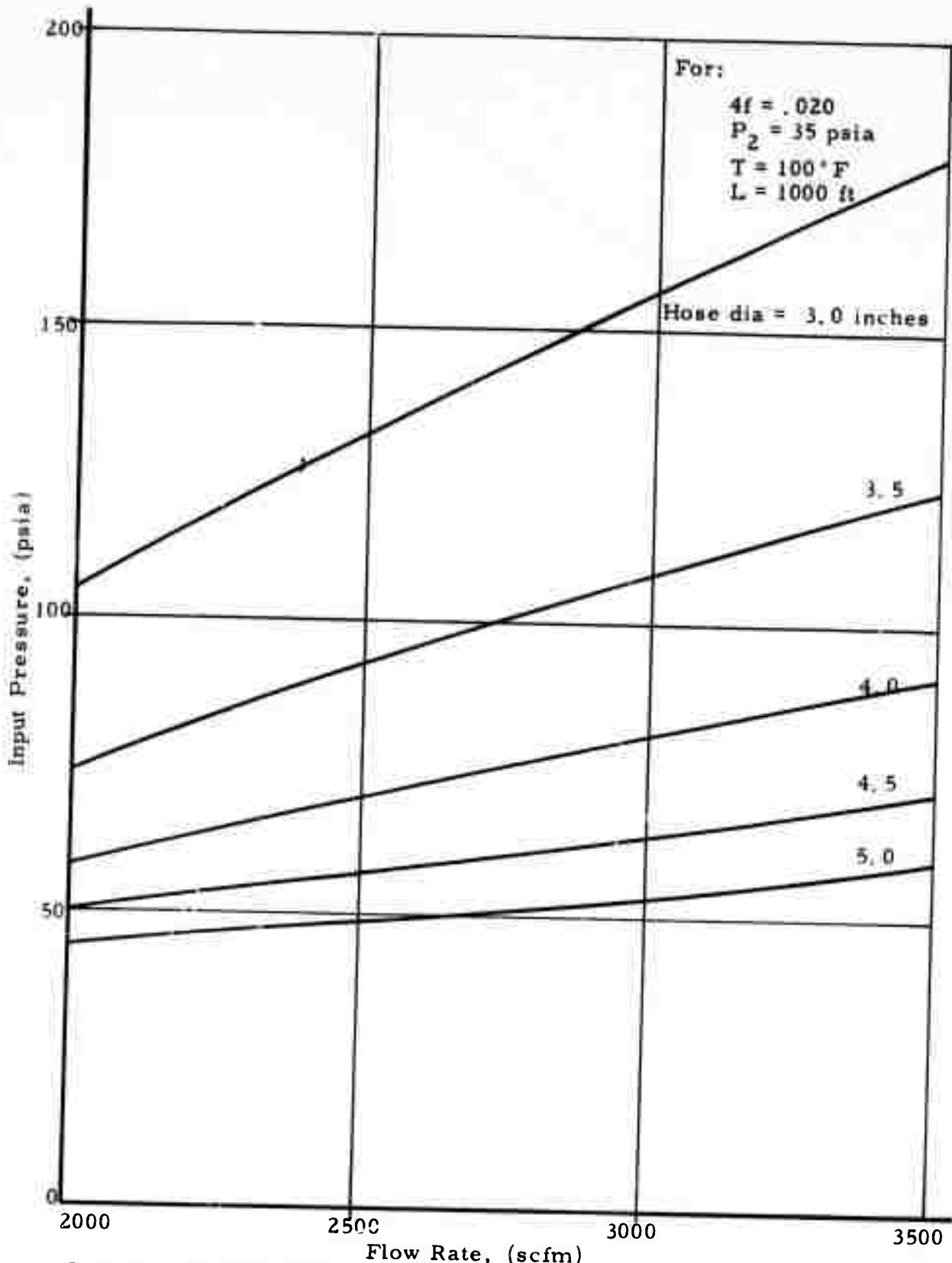
Compressor Input Pressure versus Flow Rate for Various Hose Sizes
