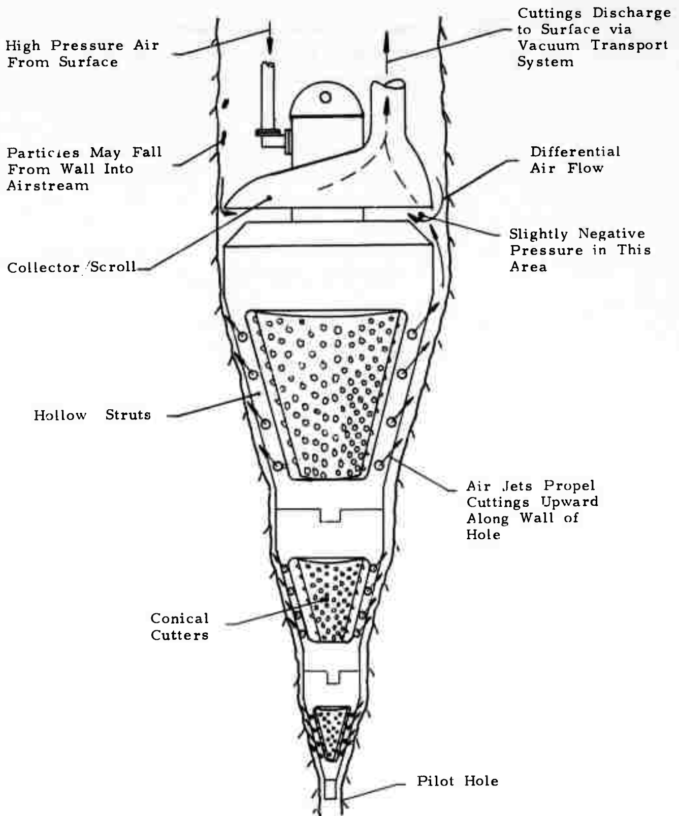
Overall Mucking System Concept
