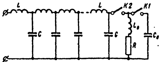
Fig. 5. Pulse-shaping circuit using artificial line: L_0 , R - load parameters; C_0 - capacitor battery for initial field excitation; K_1 , K_2 - switching elements.
