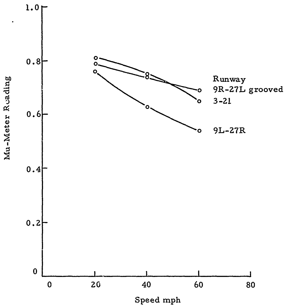
MU vs. SPEED - WET
