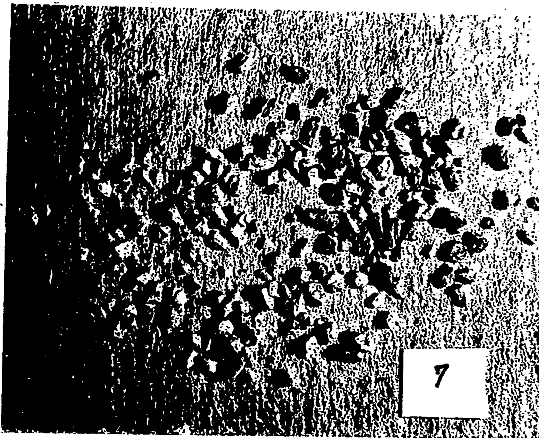
Photo F3. SOM-7, expansive clay, x2
