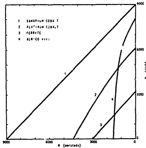
Fig. 1. Demagnetization curve for various permanent magnet materials.
