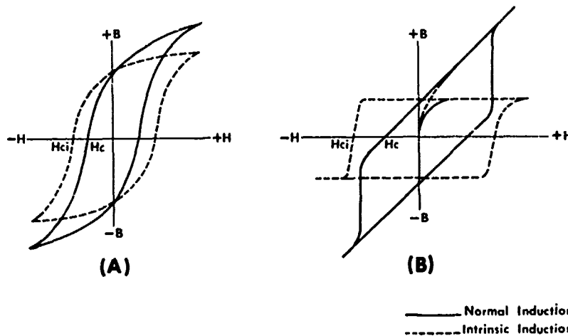
Fig. 2. Comparison of magnetization, M , and induction, B , as a function applied field, H .
