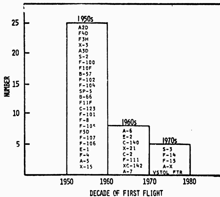
Figure 14 - Military Fixed Wing Aircraft Programs (25,000 - 100,000 Pounds)
