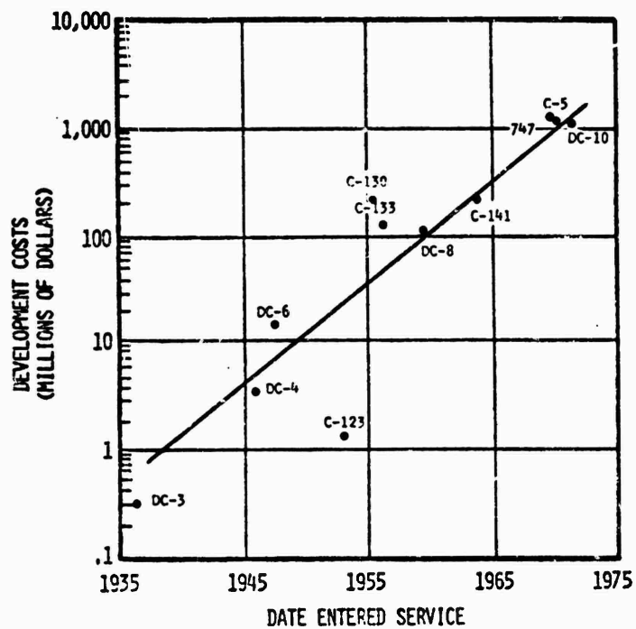
Figure 9 - Transport Aircraft Development Costs
