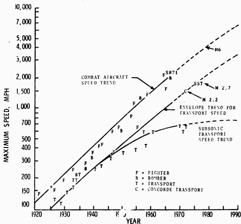
Figure 1 - Speed Trends of Aircraft
