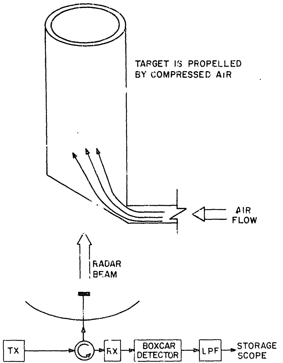
FIGURE 1. DOPPLER TECHNIQUE FOR MEASURING SMALL CROSS SECTIONS
