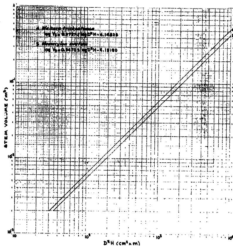
Figure 6. Allometric relation between stem volume and D^2H .
