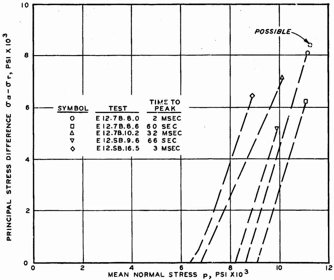
Figure 4.10 Principal stress difference versus mean normal stress showing peak stresses from five shear tests on tuff from Tunnel U12e-12.
