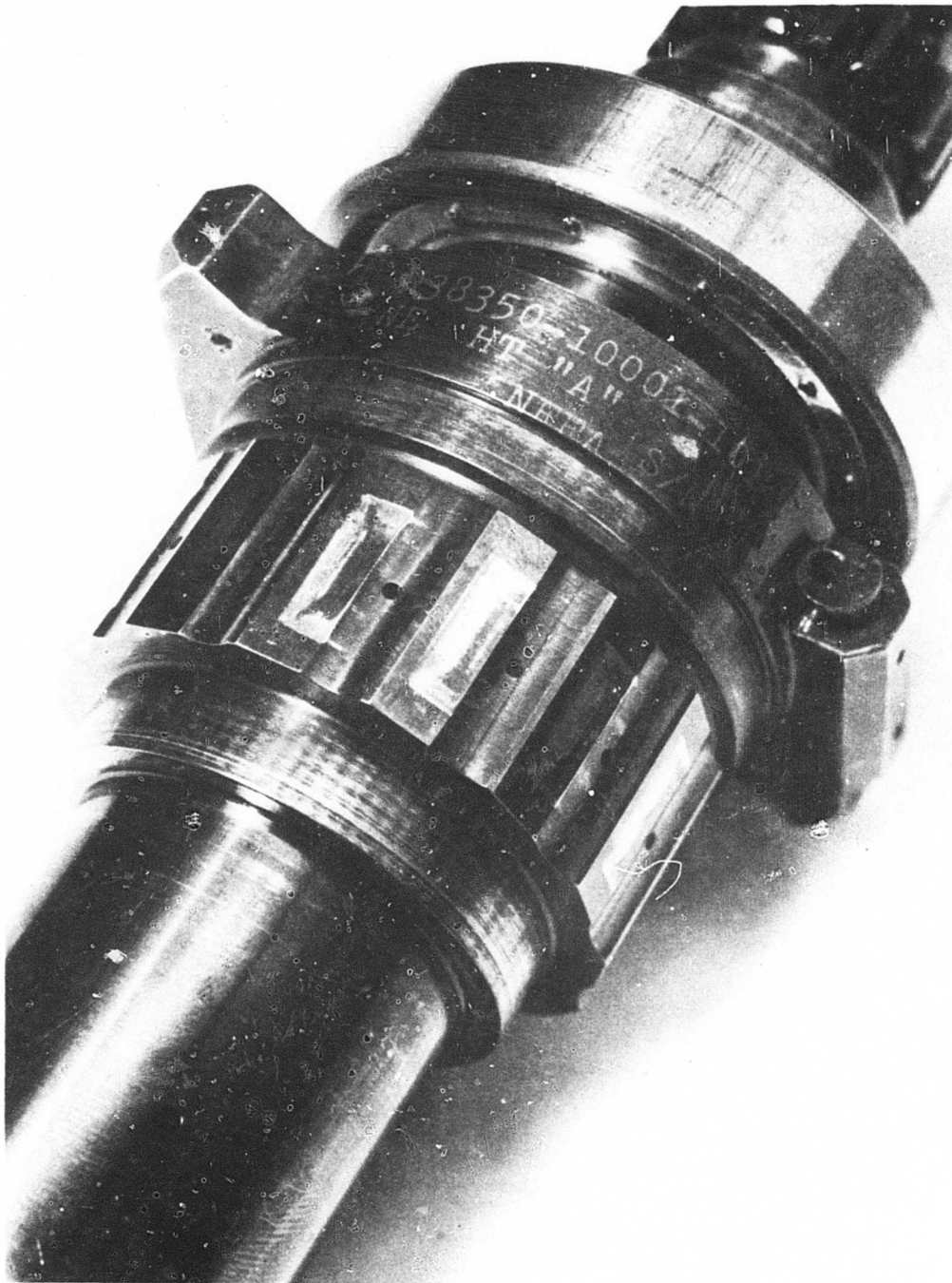
Figure 24. Cam Condition After Delayed Engagement.
