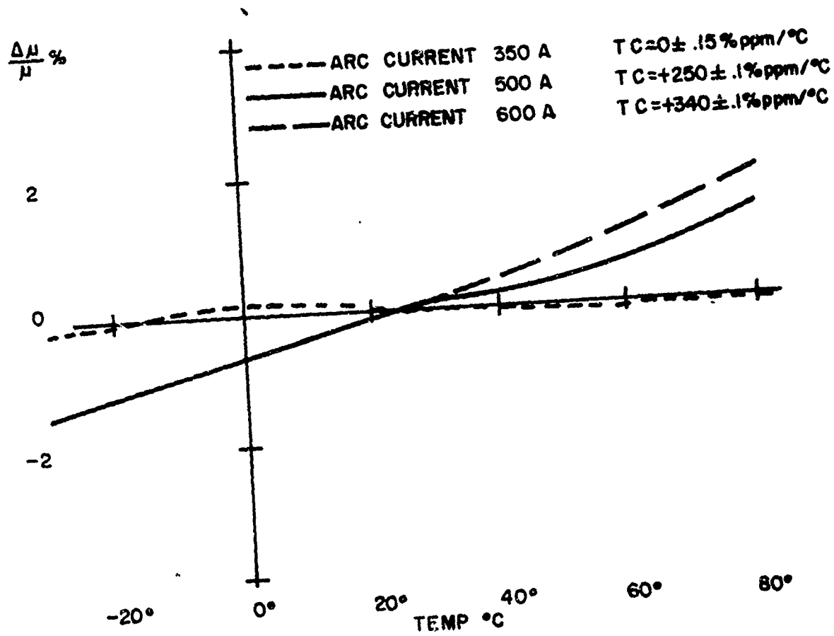
FIG. 7 EFFECTS OF ARC CURRENT ON TC AT A WORKING DISTANCE OF 1-1/2 IN (FLUID BED POWDER).
