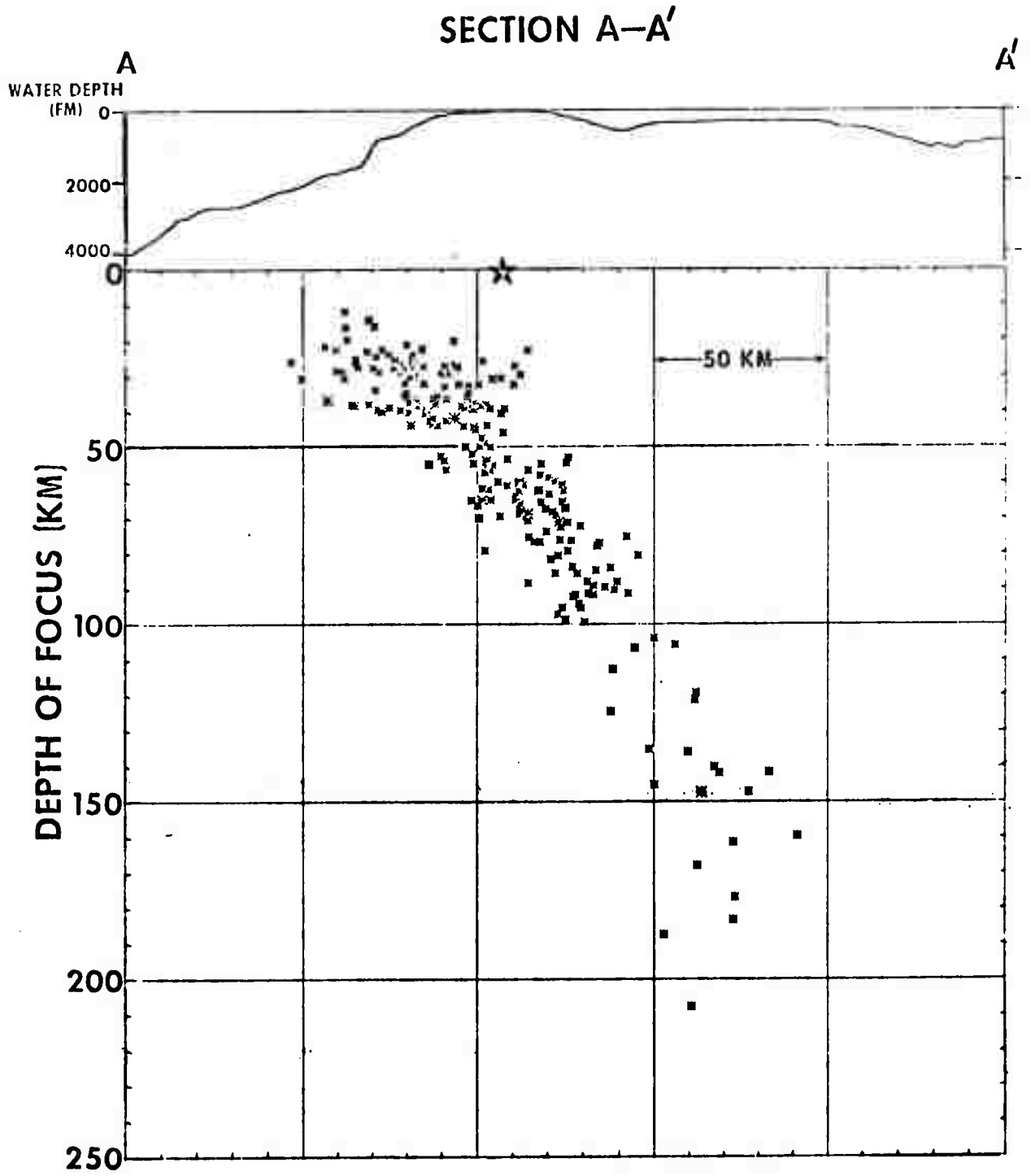
Figure 5. Earthquake depth of focus profile near Amchitka.
