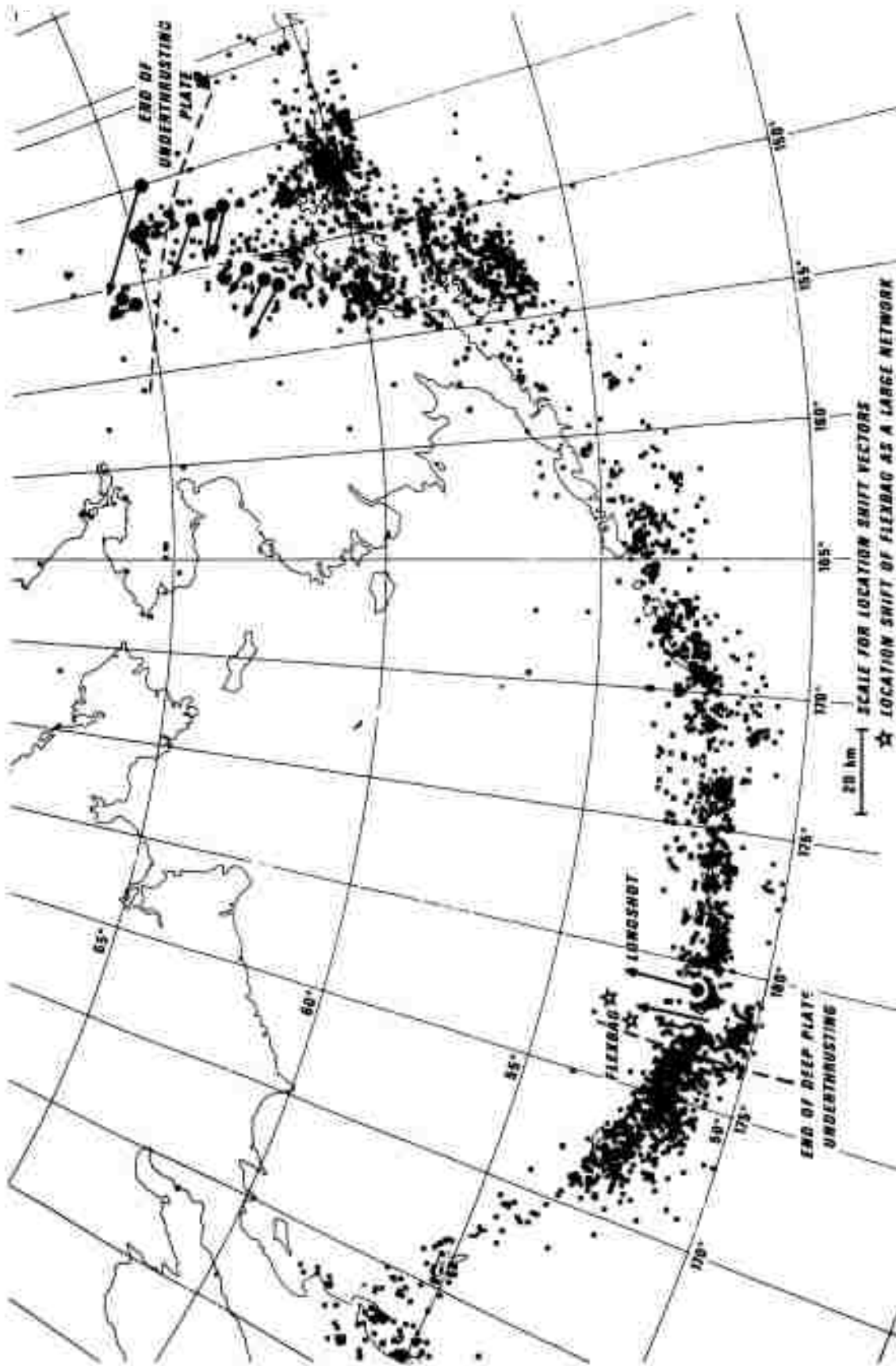
Figure 3. Seismicity and location shifts for Aleutian-Alaskan region.
