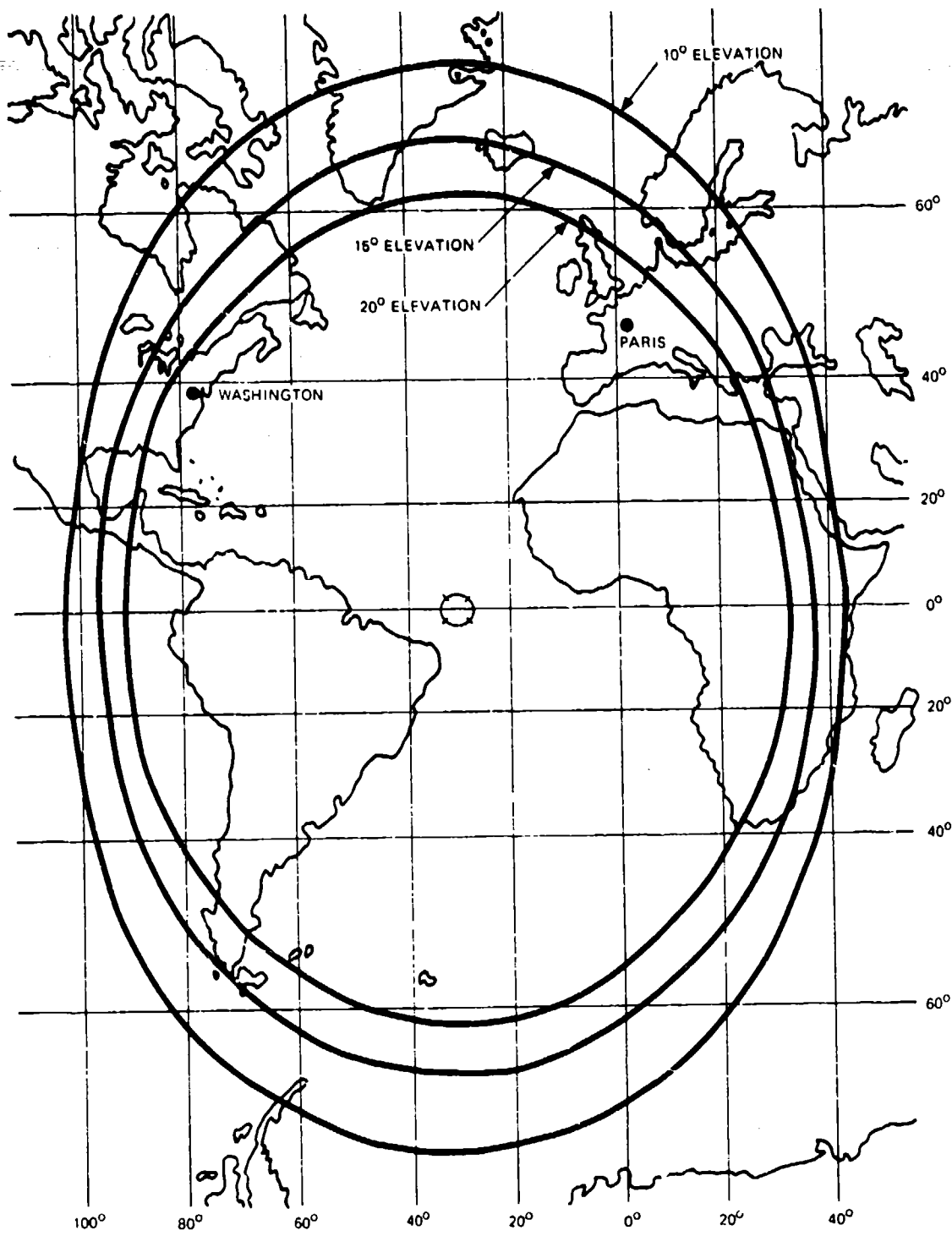
Figure 2-5. Coverage Contours for a Synchronous Satellite
