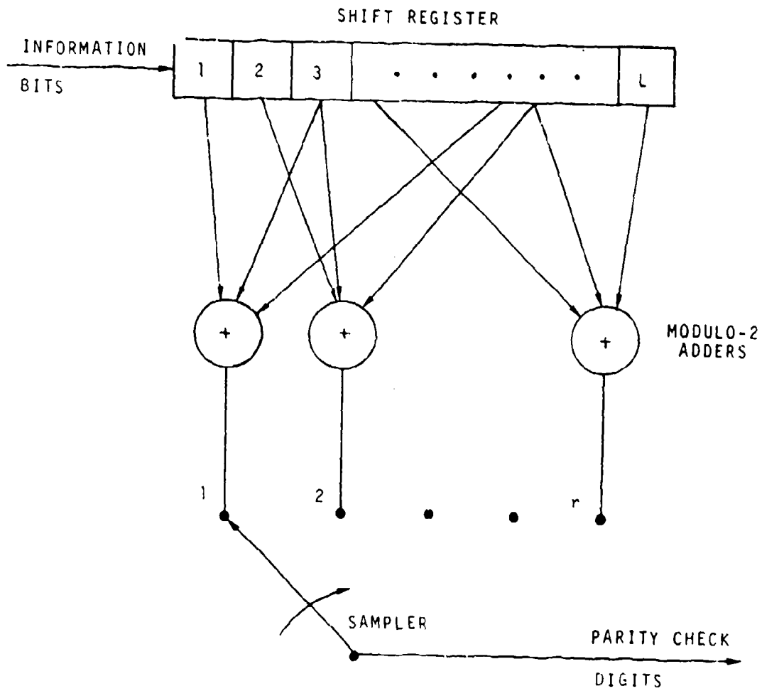
Figure 4-14. Convolutional Encoder
