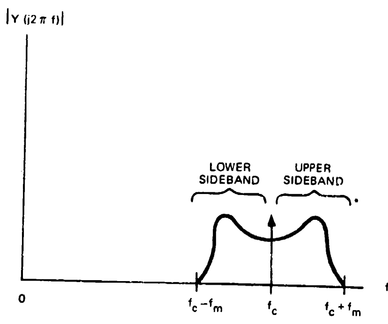
Figure 4-7. Spectrum of Amplitude Modulated Carrier
