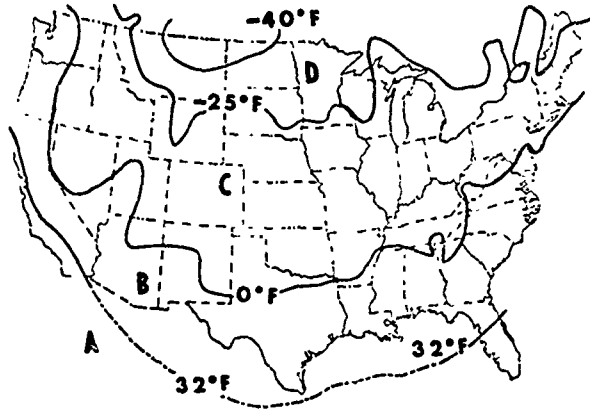
Figure 2. Lowest 1-day mean temperature isothermal lines (after ref 5).
