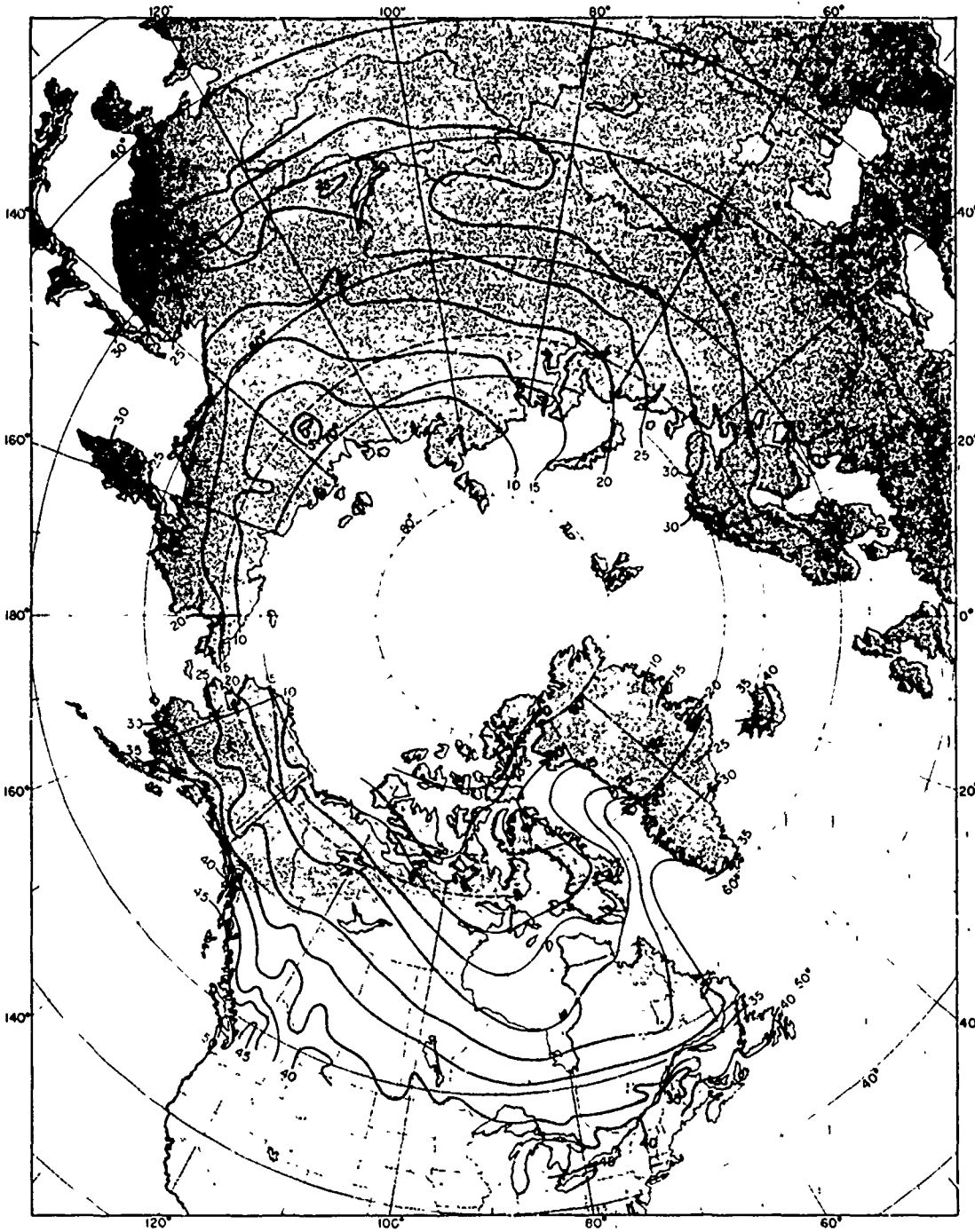
Figure 4. Mean annual temperatures of the Northern Hemisphere. 6
