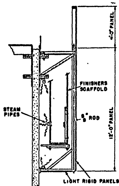
Figure 28. Rigid enclosure for winter slip-form work.*
