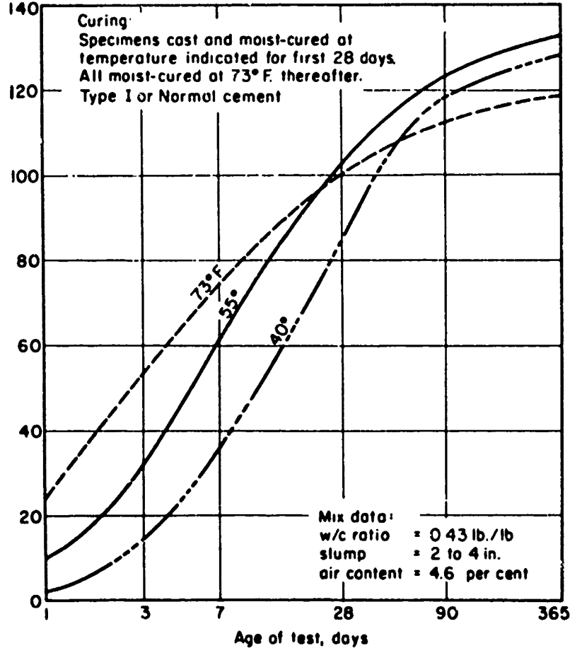
Figure 19. Effect of low temperatures on concrete compressive strength at various ages.**
