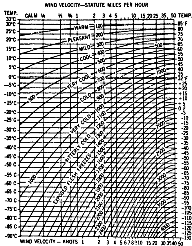
Figure 7. Graph of windchill related to temperatures and surface-wind velocity. 4
