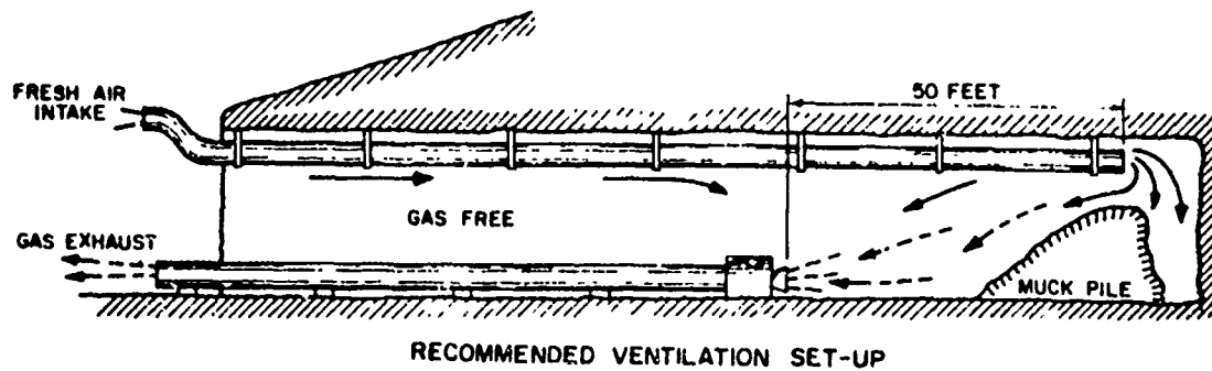
Figure 16. Ventilation. 47
