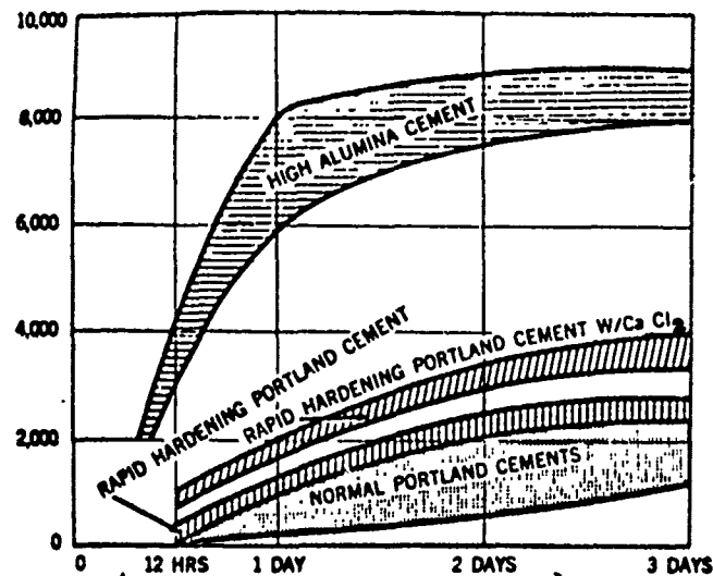
Figure 23. Comparison of compressive strengths. 14
