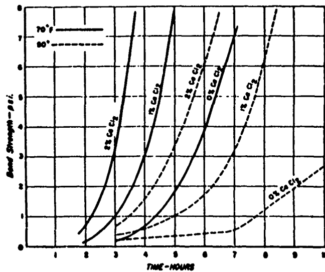
Figure 25. Increase of early strength accompanying the use of calcium chloride. 14
