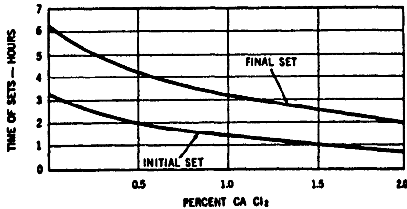
Figure 24. Effect of calcium chloride on initial and final set of portland-cement concrete. 14
