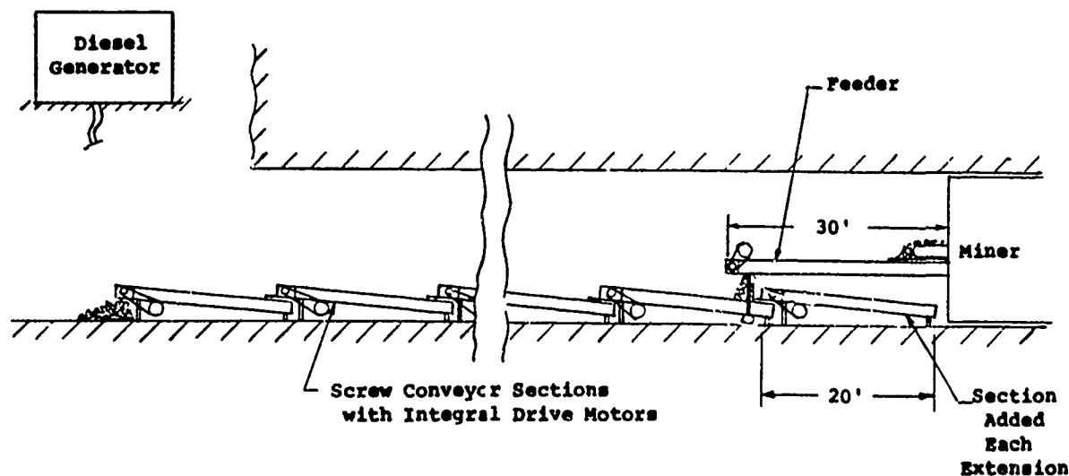
Figure 18. Modular screw conveyor concept. 25
