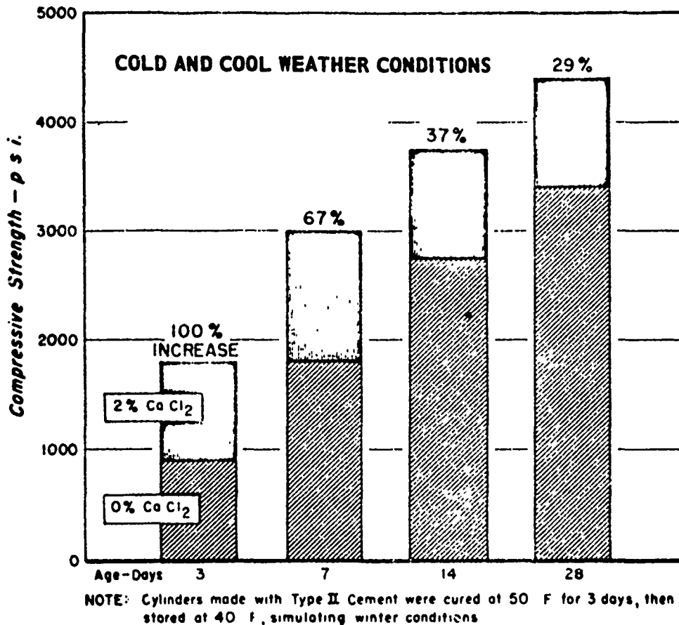
Figure 26. Compressive strength increase (using CaCl 2 ). 5
