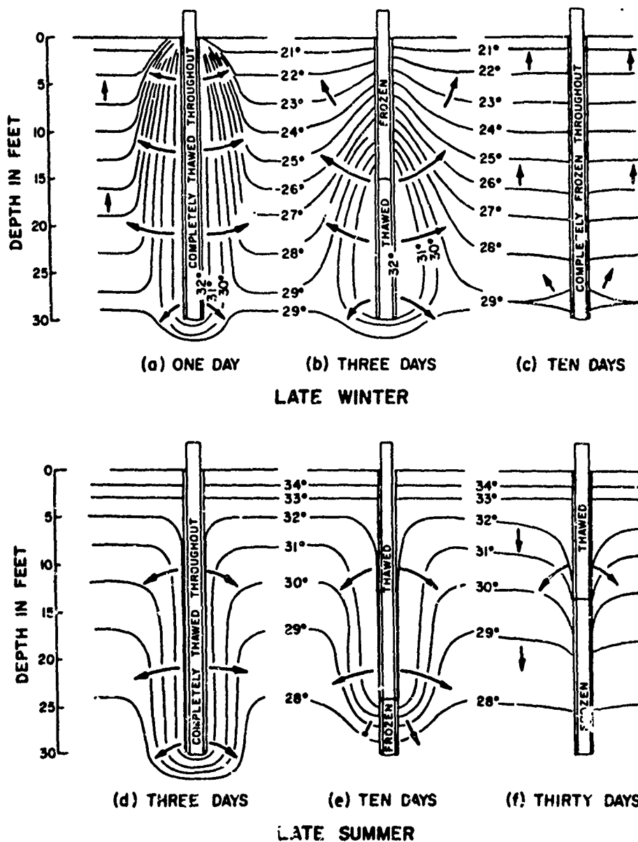
Figure 14. Natural freezeback of piles in permafrost during winter and summer. 15
