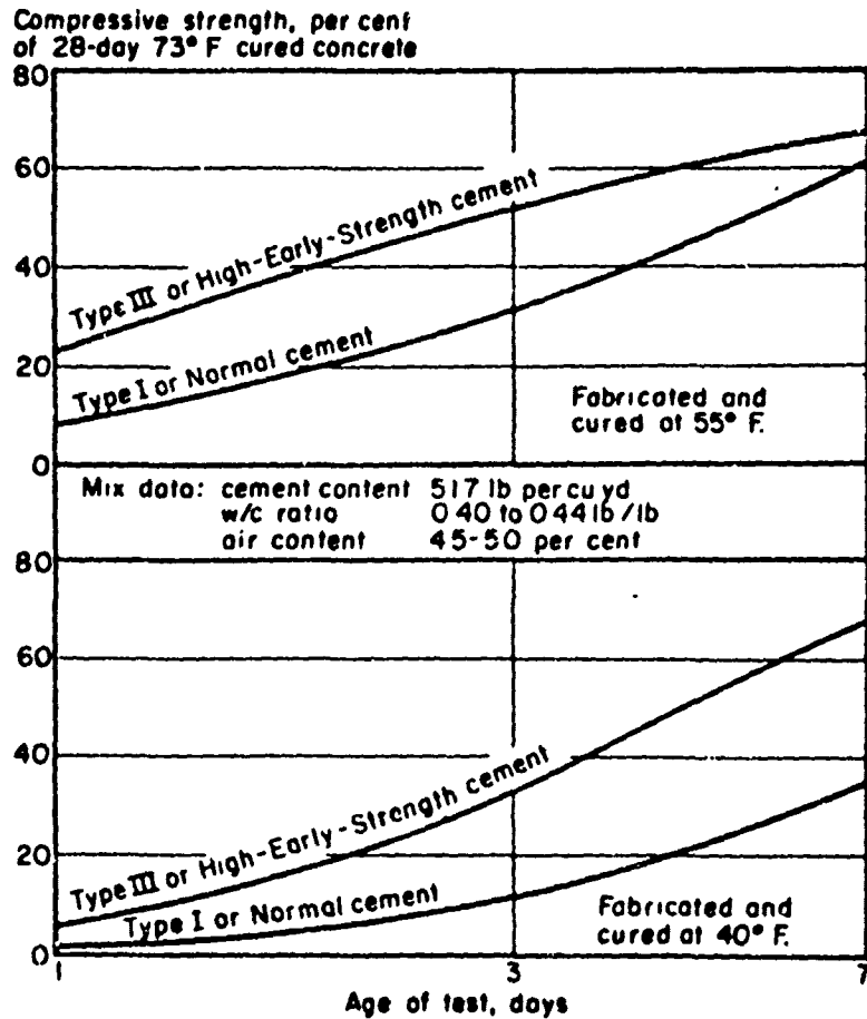
Figure 20. Early compressive strength relationships involving portland cement types and low curing temperatures.*
