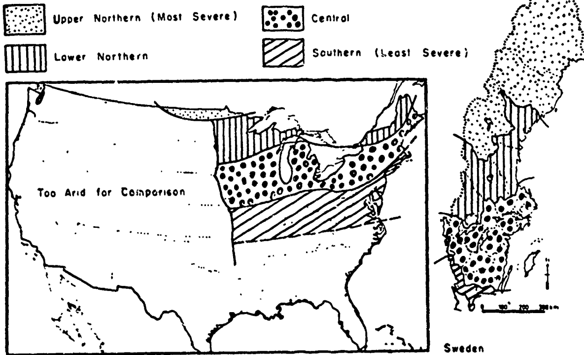
Figure 3. Comparison of climatic conditions of Sweden and the United States. 2
