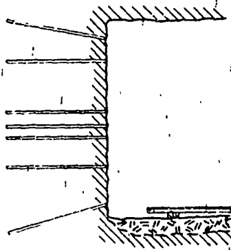
LONGITUDINAL SECTION OF DRILL PATTERN.
