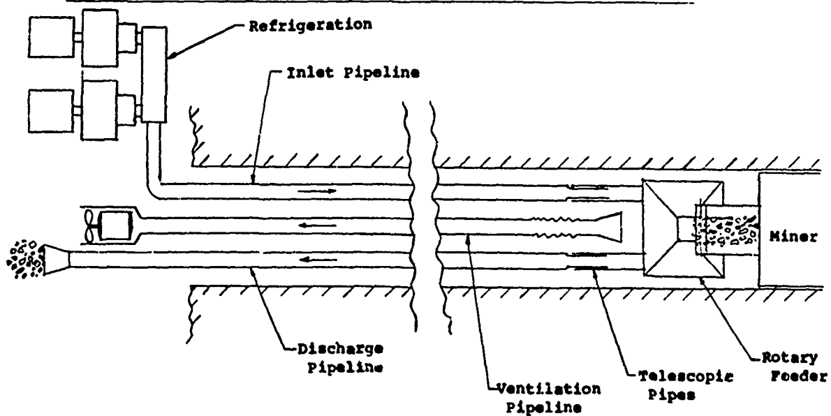
Figure 17. Pneumatic pressure concept. 25
