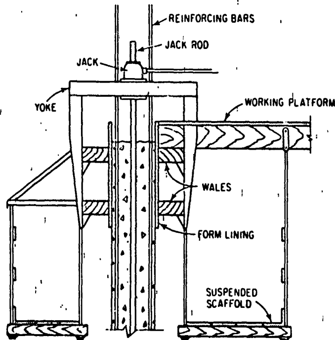
Figure 27. Slip form for concrete wall. 26*
