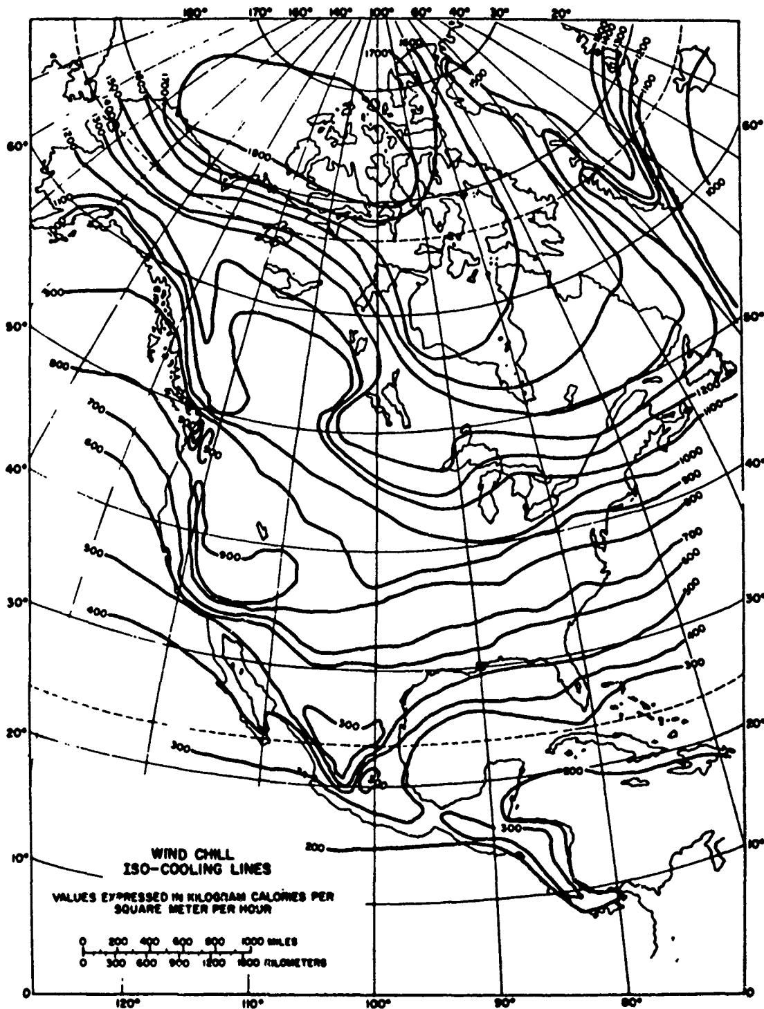
Figure 8. January windchill values for North America. a
