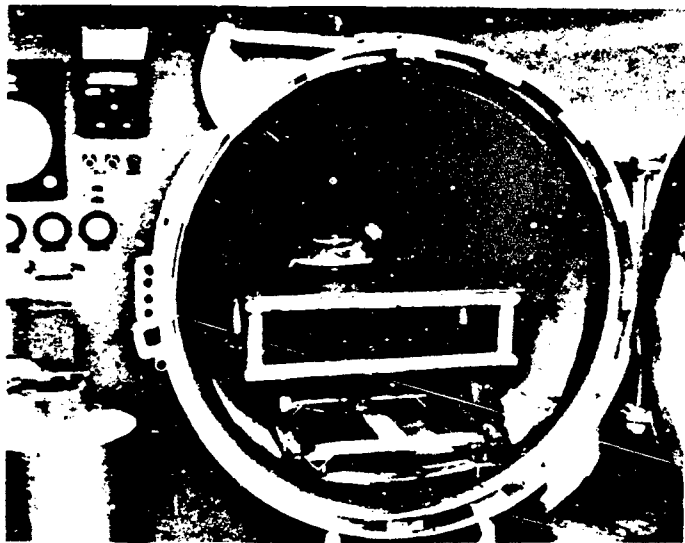
Figure 18. Vacuum Bagged Part in Autoclave Ready for Curing
