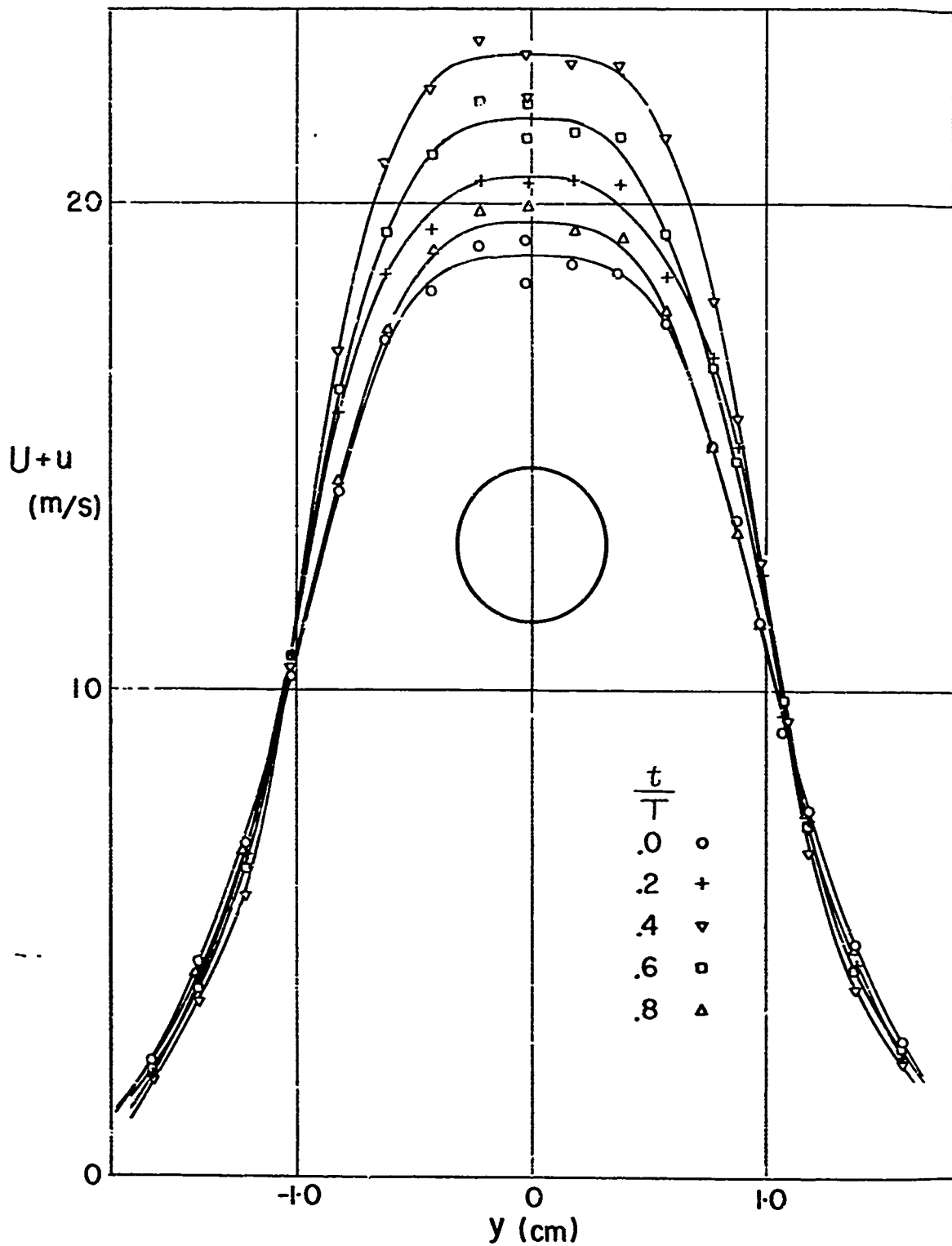
Fig. 8 Instantaneous velocity distribution of pulsating jet at x = 5 cm, f = 450 Hz
