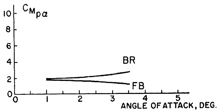
Fig 25 Comparison of the nonlinear aerodynamic coefficients of body of revolution (BR) and body with boattail fins (FB)
