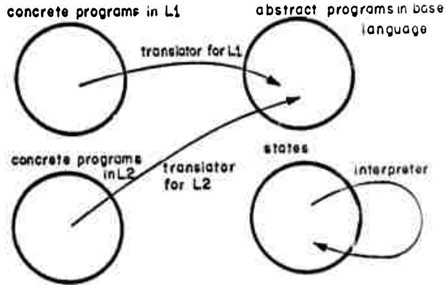
Figure 3. Language definition in terms of a common base language.
