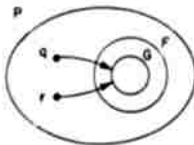
Figure 16. Procvr diagram for program 1 showing absence of necessary conditions for the occurrence of cycles.
