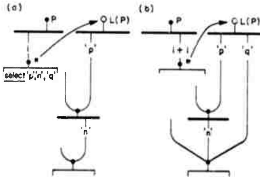
Figure 6. Interpretation of a select instruction.
