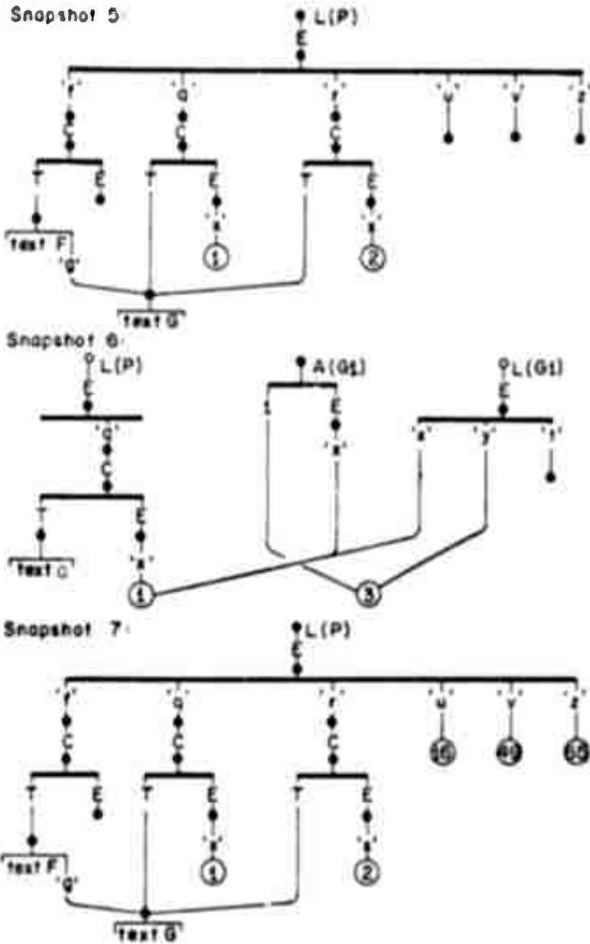
Figure 14. Interpretation of c block structured program — application of closures.
