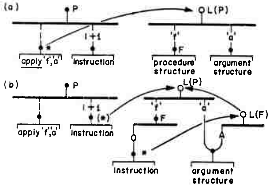
Figure 10. Initiation of a procedure activation by an apply instruction.
