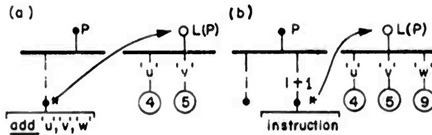
Figure 5. Interpretation of an instruction specifying a binary operation.
