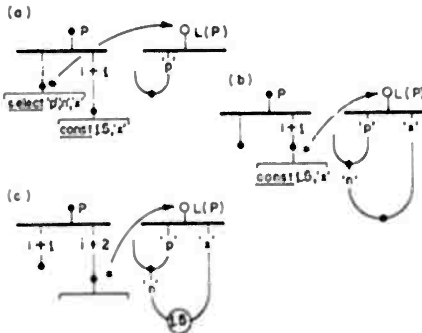
Figure 7. Structure building using select and const instructions.
