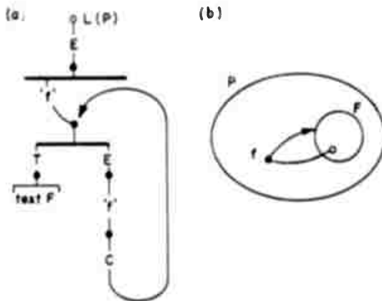
Figure 15. Interpreter state for program 2 showing the cycle introduced, and the corresponding procvr diagram.
