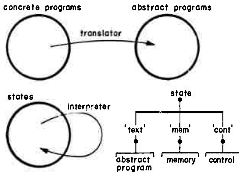
Figure 2. Language definition by the Vienna method.
