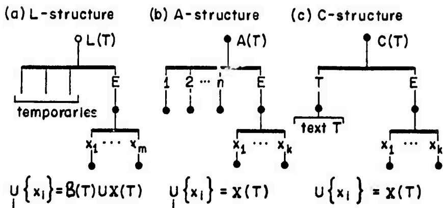
Figure 12. Formats of local, argument, and closure structures for the interpretation of block structured programs.
