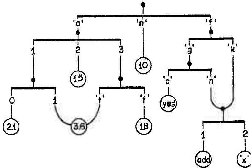
Figure 1. An example of an object.
