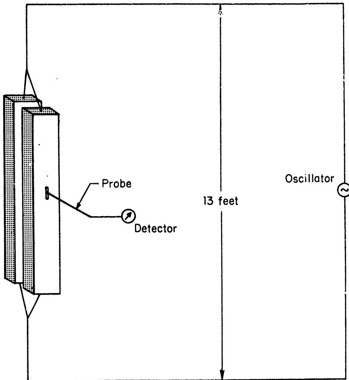
EXPERIMENTAL APPARATUS
