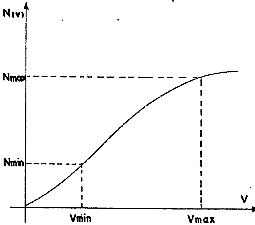
Figure 21. Gain Characteristic with Positive Bias Voltage and Positive Slope.
