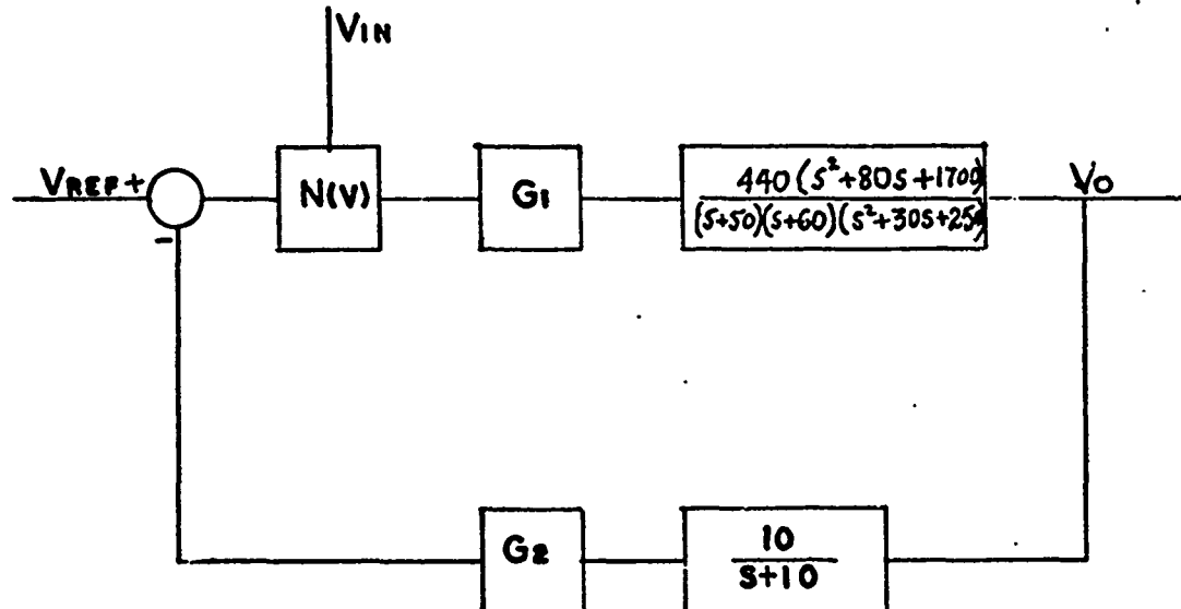
Figure 60. Block Diagram of AGC System for Example 2.
