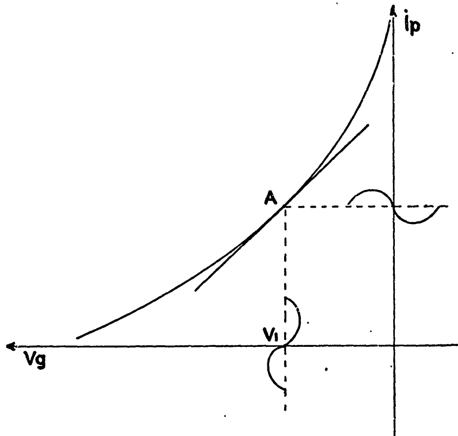
Figure 16. Typical Amplifier Characteristic.
