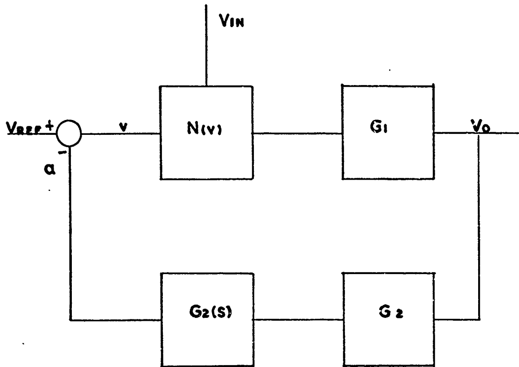
Figure 28. Block Diagram of the Simulated Example.
