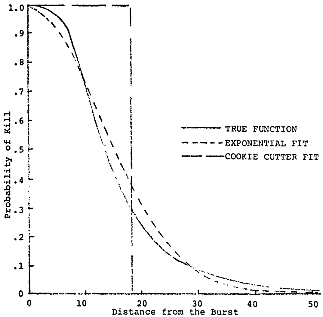
Figure 3. Round Lethality Function
