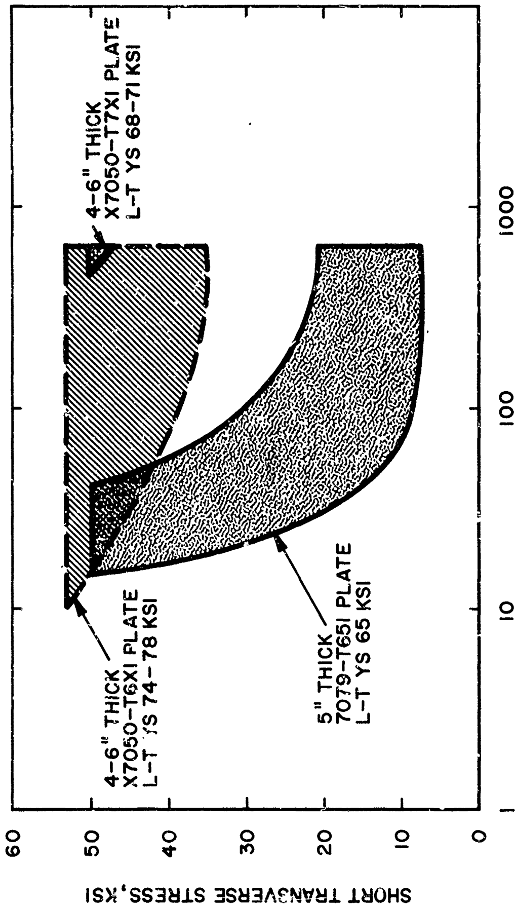
FIG.11 COMPARES PERFORMANCES OF THICK X7050 AND 7079-T65I PLATE
