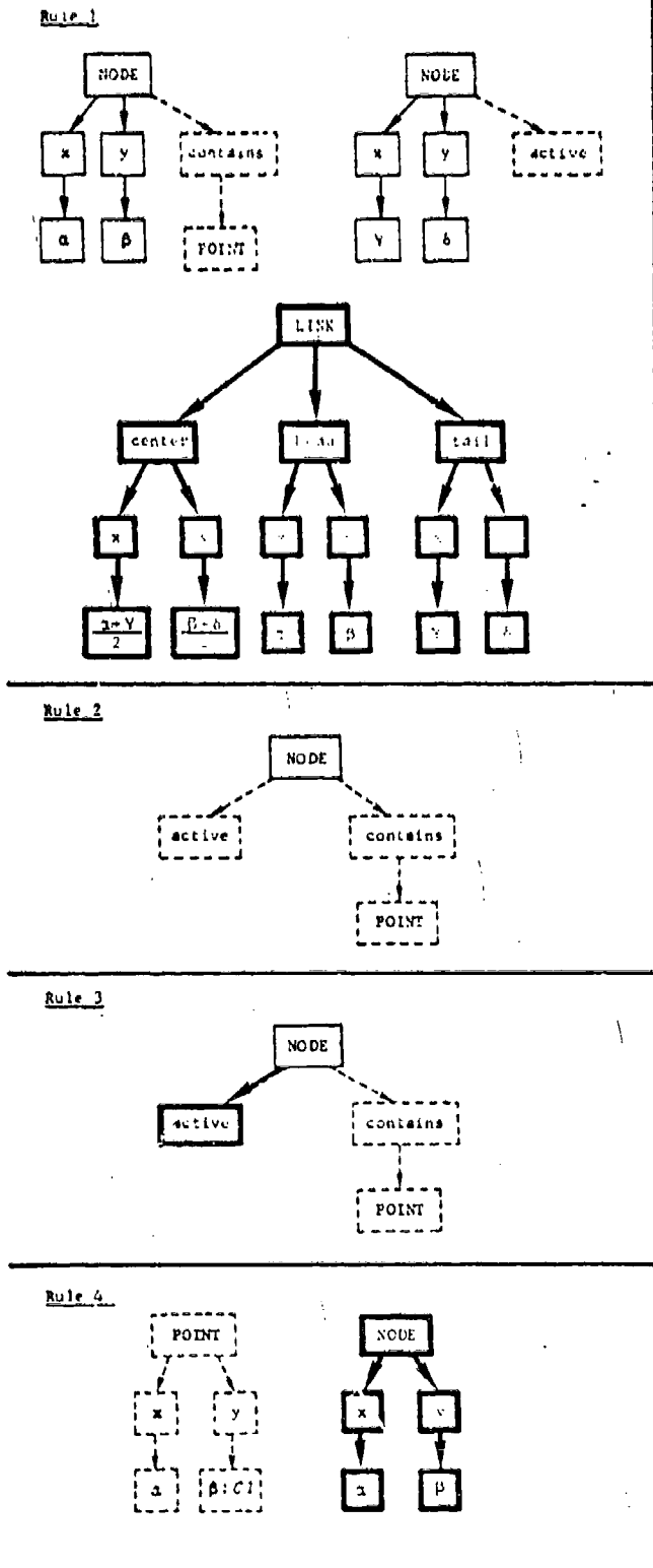
Fig. 2--A Set of Four Pattern-Replacement Rules
