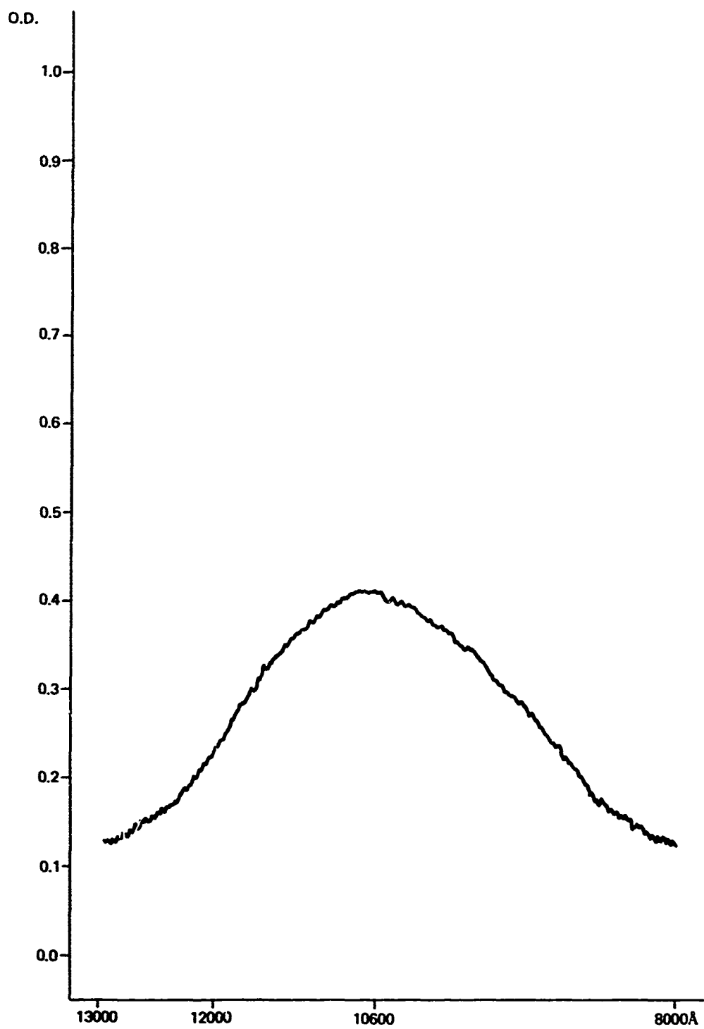
Figure 15. Optical Density of 106-5 Dye in PMMA
