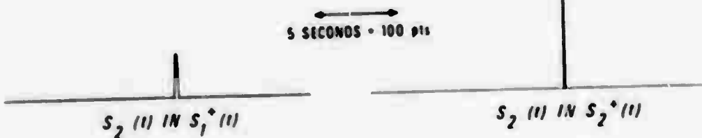
Figure 3. Comparison of distortion introduced by truncated optimum filters and ordinary beamforming. Seven channels (21-27) with S_1(\cdot) at 17 kn/sec, 300 degrees and S_2(\cdot) at 23 kn/sec, 300 degrees.
