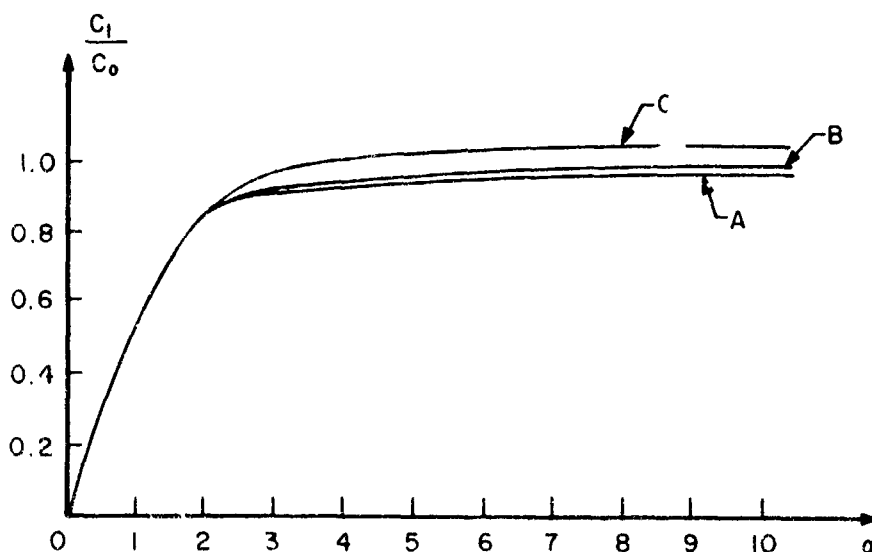
Figure 26. Variation of the phase velocity with respect to \alpha under the following conditions of longitudinal constraint and Poisson's ratio: Curve A: k = 0 , unconstrained tube and \sigma = 1/2 Curve B: k = -2 , tube with small constraint and \sigma = 1/2 Curve C: k = -\infty , completely constrained tube and \sigma = 1/2
