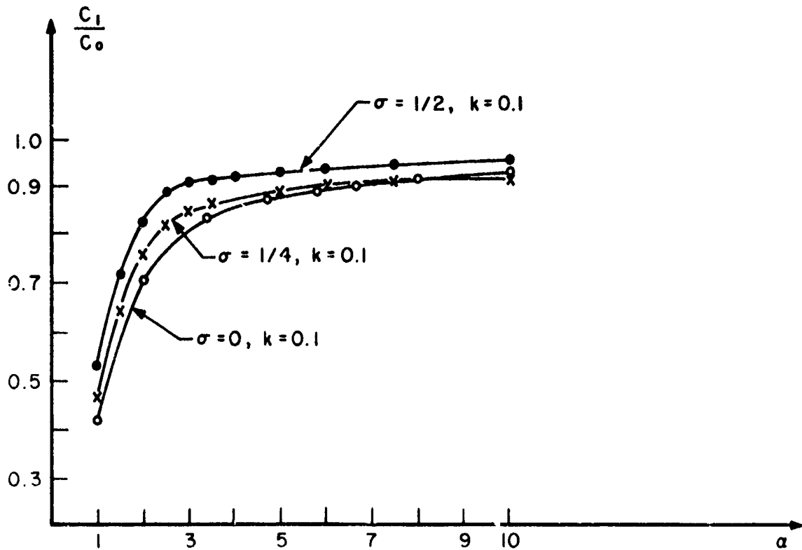
Figure 24. Variation of c_1/c_0 with respect to \alpha . Note that for values of \alpha greater than 3, which are those of greatest practical interest, the change in the velocity ratio, c_1/c_0 , with respect to \alpha is quite small.
