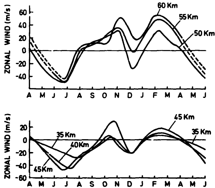
Figure 9. Seasonal Variation of Zonal Wind Component at Sonmiani (25°N) [92]
