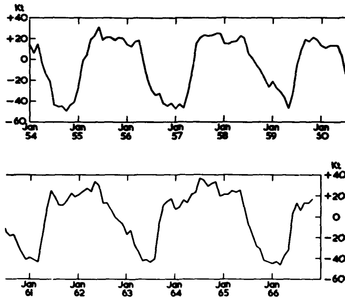
Figure 10. Monthly Mean Zonal Wind Components at 50 mb for Canton Island (2° 46'S, 171° 43'W). Components towards the east are positive [94]
