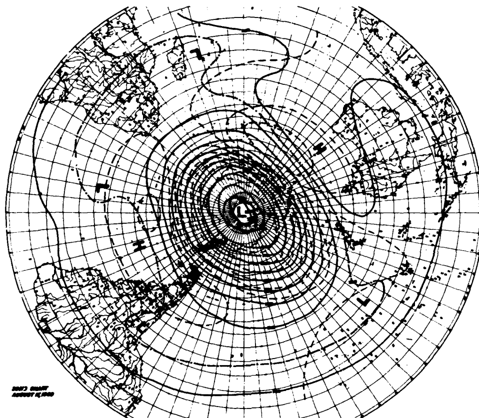
Figure 5. Analysis Chart (30 mb) for 17 August 1969. Units: geopotential meters and degrees Celsius [90]
