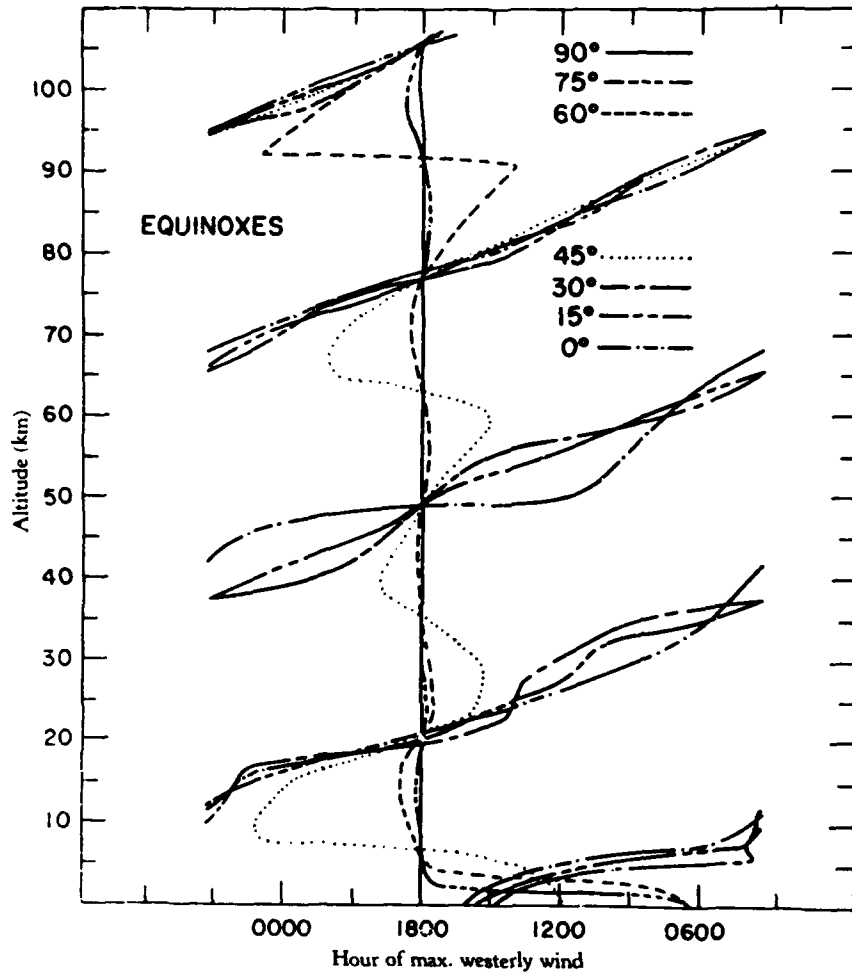
Figure 13. Altitude Distribution of the Phase of the Solar Diurnal Component of the W-E flow at 15^\circ Intervals of Latitude for Equinoctial Conditions [104]
