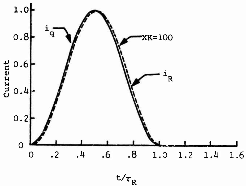
Figure 5. Example of Results from Study of Ideal Circuit
