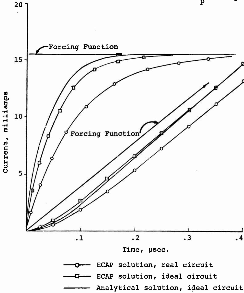
Figure 36. Results of Circuit Studies, HST-41 Crystal
