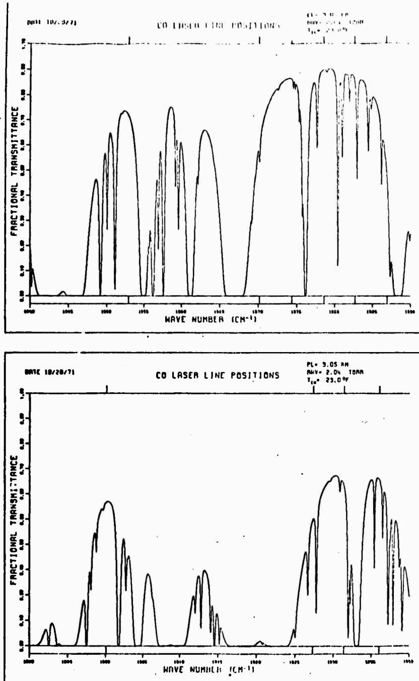
Fig. 1. Calculated horizontal atmospheric transmittance in the region 1890 to 1940 \text{cm}^{-1} through a 3.05 km path in which the absorbing gas is 2.04 torr of water vapor. The temperature and amount of water vapor present are those occurring at Rome, New York, January 6, 1971. Fewer water lines were used to calculate the transmittance than was used in the calculations for the same conditions listed in Table 1 to limit the computer time necessary to produce this plot.
