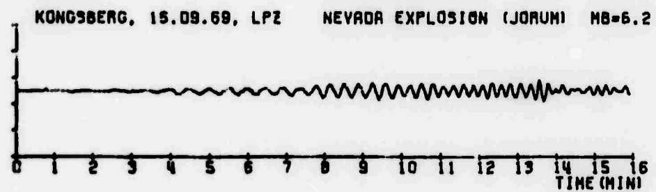
Fig. 13. Nevada explosion. Raw trace (bottom) and chirp filter output (top).
