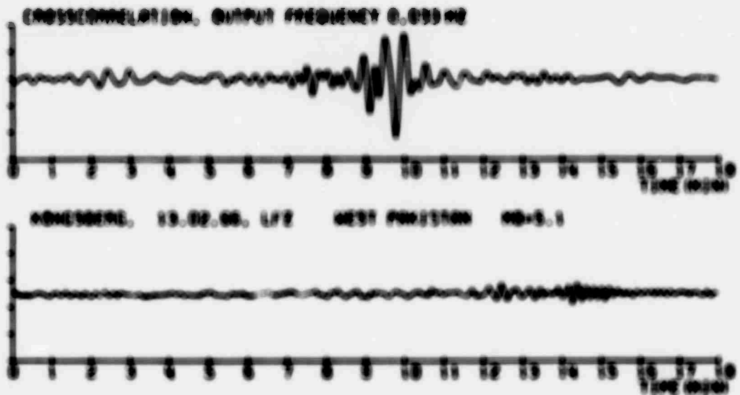
Fig. 9. West Pakistan event. Raw trace (bottom) and extended chirp filter output (top).
