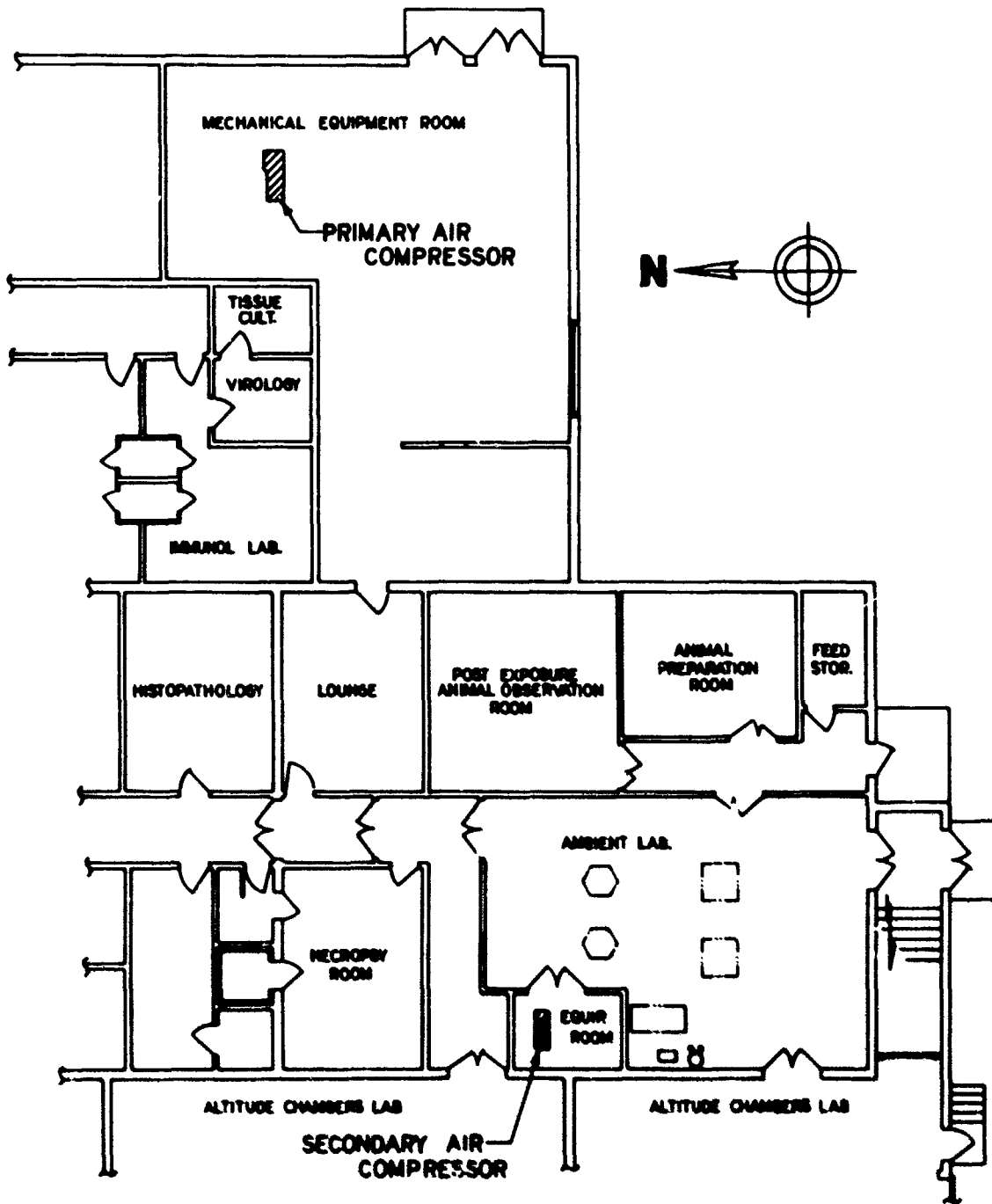
Figure 8 Plan View of Instrument Air Compressor Stations
