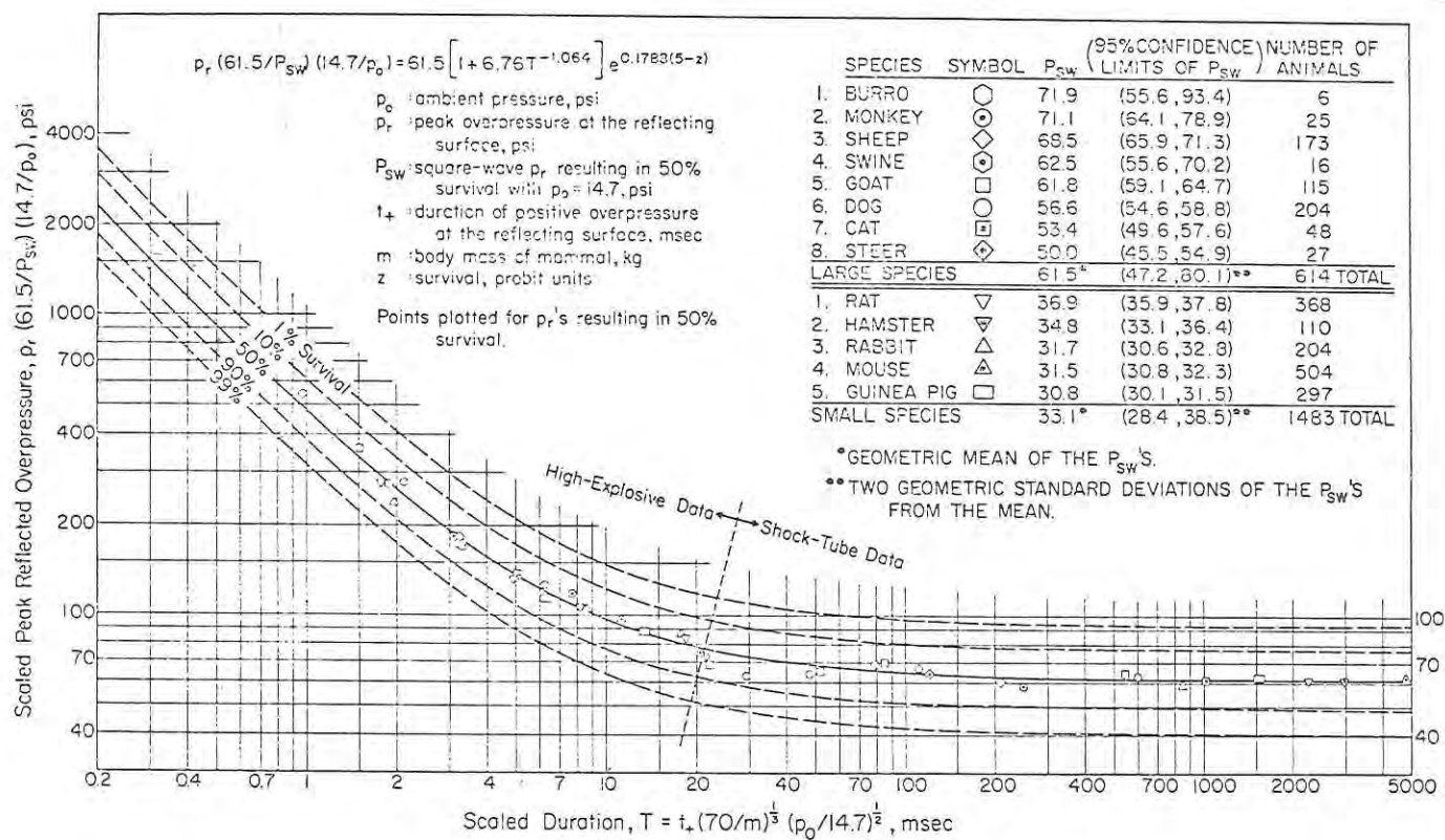
Figure 32. --Survival curves (24-hour), applicable to "sharp-rising" blast waves, derived from the analysis of data for 12 mammalian species (excluding guinea pigs). See text for explanation of plotted points. From Bowen et al. (Reference 94).
