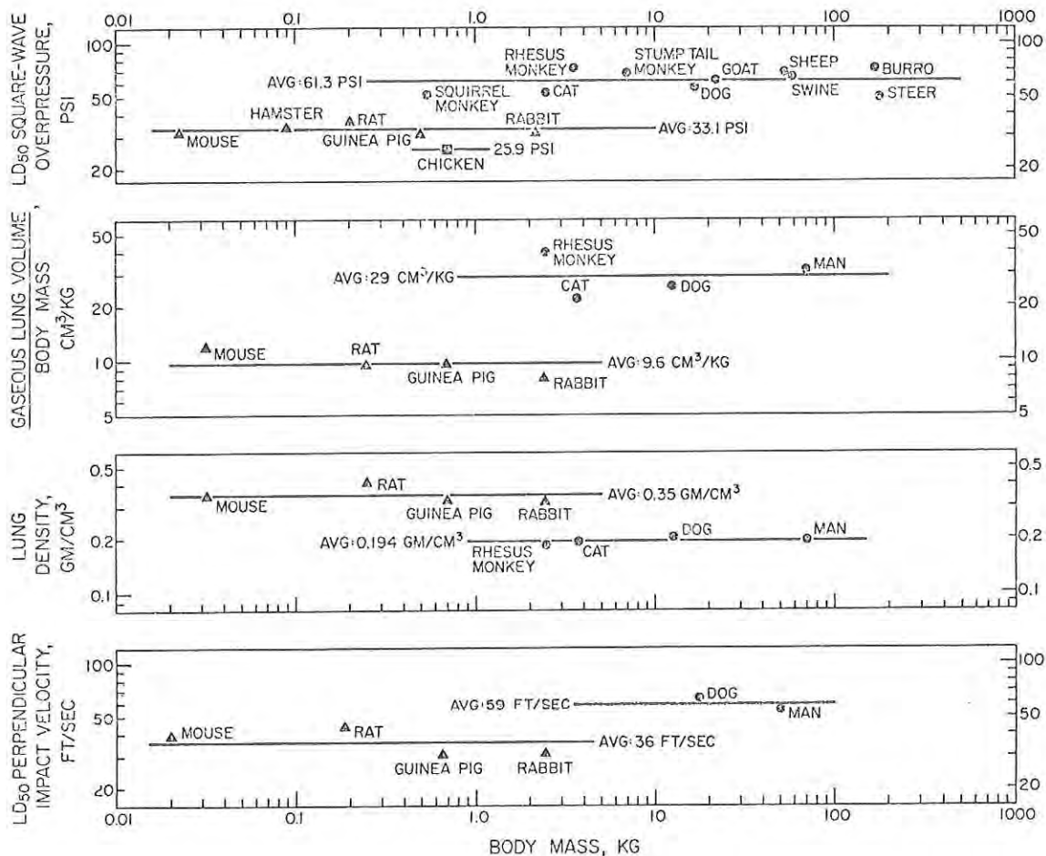
Figure 37. --Animal body mass versus the "square-Wave" overpressure for 50-percent survival at sea-level, the average gaseous lung volume divided by body mass, the average lung density, and the 50-percent lethal velocity for perpendicular impact with a non-yielding surface. Note that in each instance the mammals segregate into two groups and that the average values for the more- and less-tolerant groups. Pressure data from Fletcher (Reference 59), lung data from Crosfill and Widdicombe (Reference 63), impact data from Jones et al. (Reference 97). After Fletcher (Reference 59).
