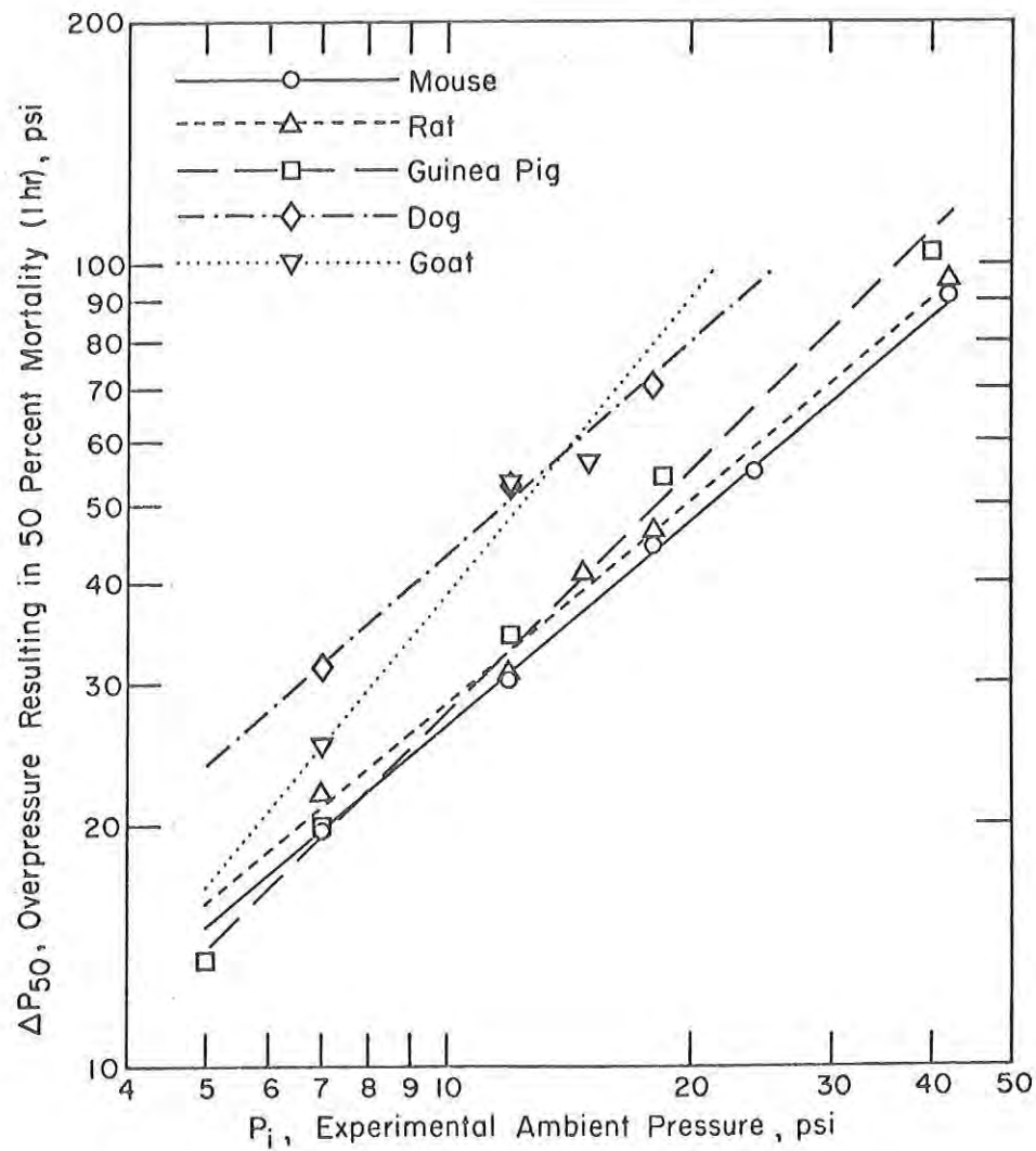
Figure 9. --Relation of the 50-percent, 1-hour survival pressure to experimental ambient pressure for 5 species of mammals. After Damon et al. (Reference 67).
