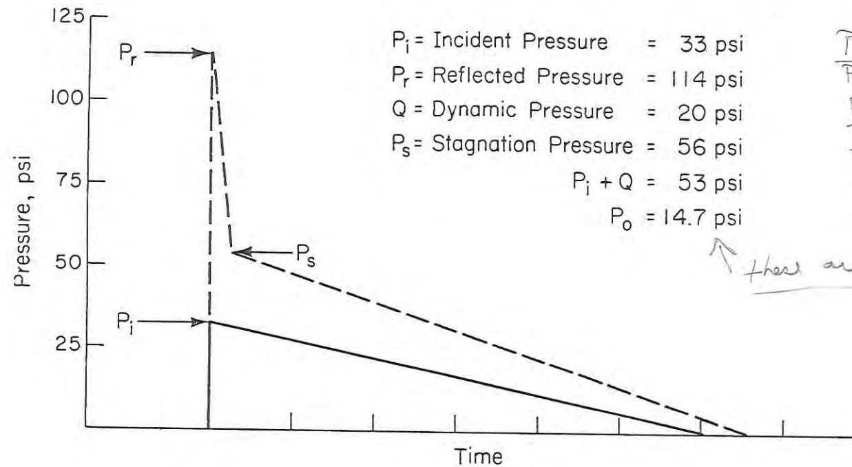
Figure 10.--The relations between the incident, reflected, dynamic, and stagnation pressures. Modified from White and Richmond (Reference 68).
