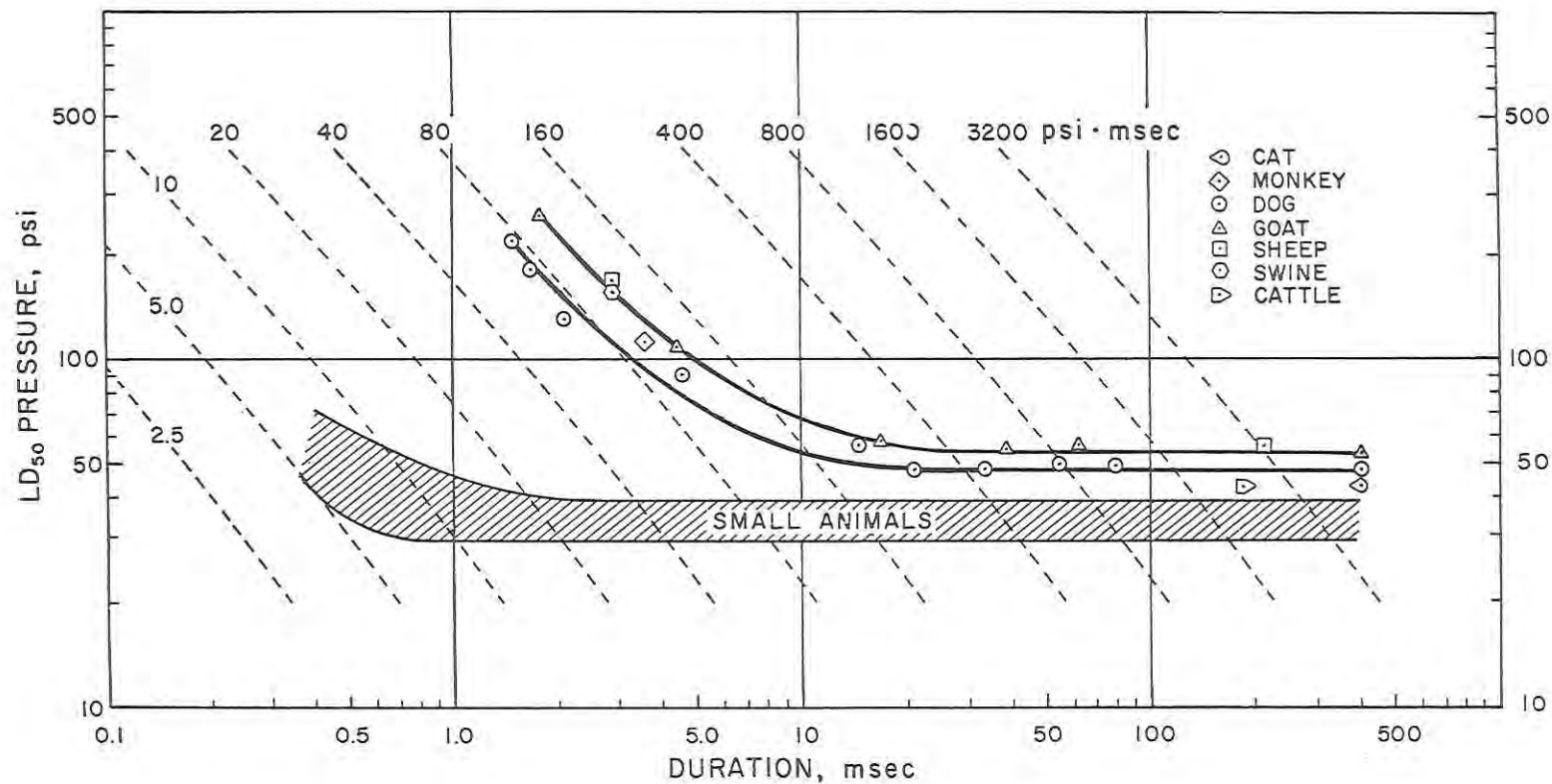
Figure 5.--The pressure-duration relationship and lethality at 24 hours for large and small animals (mice, rats, hamsters, guinea pigs, and rabbits). All measurements were made at an ambient pressure of 12 p.s.i. After Richmond et al. (Reference 52).
