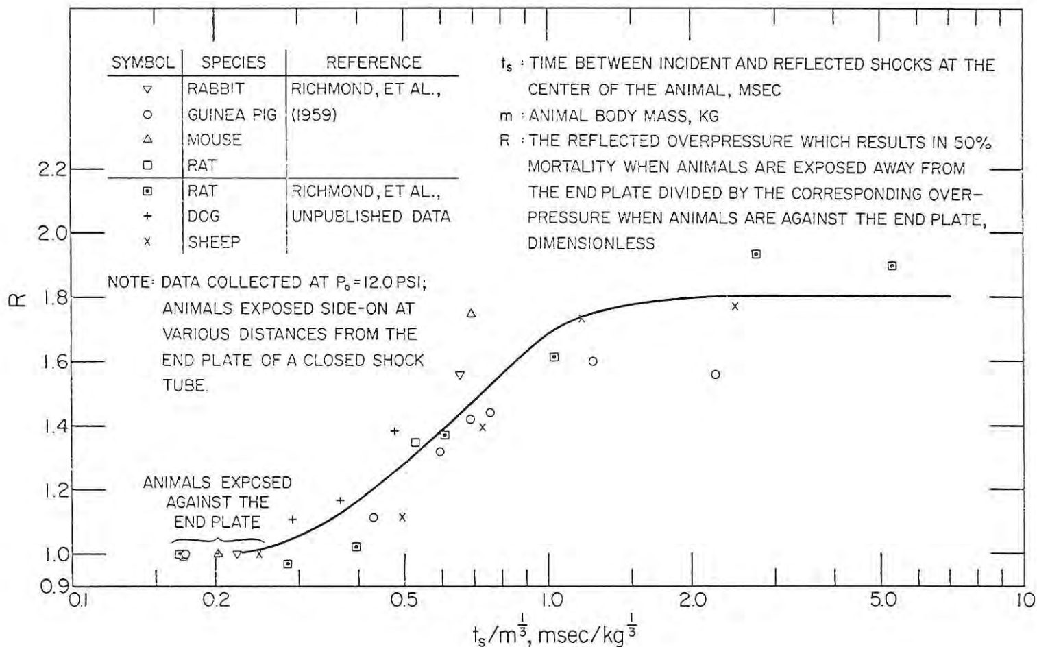
Figure 31. --Increase in tolerance when the time to maximum pressure is delayed by separating the incident and reflected pressure pulses for "fast-rising," "long-duration" waves. Data from Richmond et al. (References 72 and 88). After Fletcher (Reference 59).
