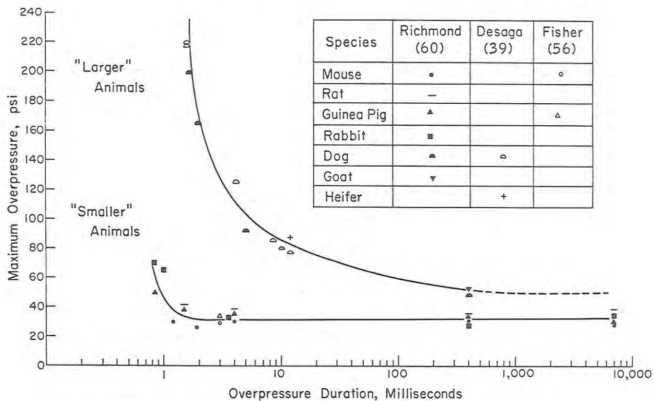
Figure 8. -- Fifty-percent, twenty-four-hour survival curves for larger and smaller animals. Modified from Richmond et al. (Reference 60).
