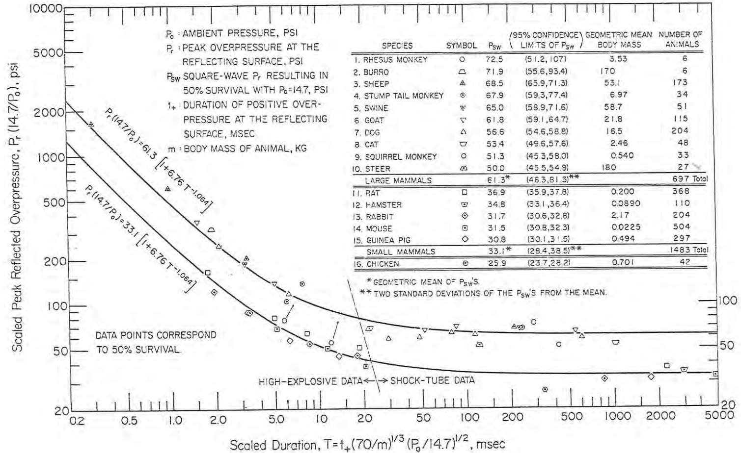
Figure 33. --Scaled peak reflected overpressures and scaled durations for "sharp-rising" blast waves which will result in 50-percent mortality. The curves, computed for a hypothetical average large and small mammal, were derived from data mostly tabulated by Bowen et al. (Reference 94). After Fletcher (Reference 59).
