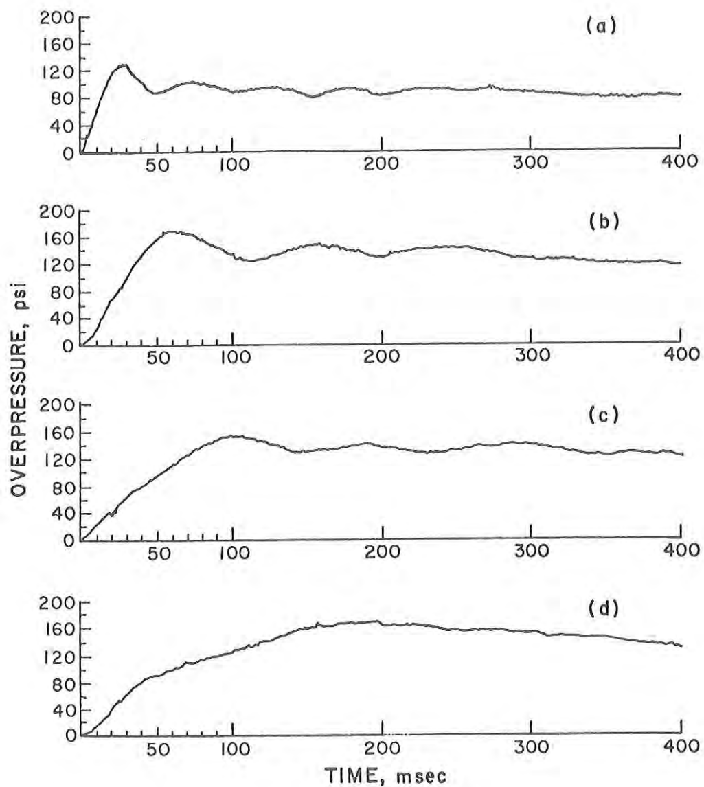
Figure 16. --"Slow-rising," pressure-time patterns with various rates of rise. Recordings made at an ambient pressure of 12 p.s.i. After Richmond et al. (Reference 73).
