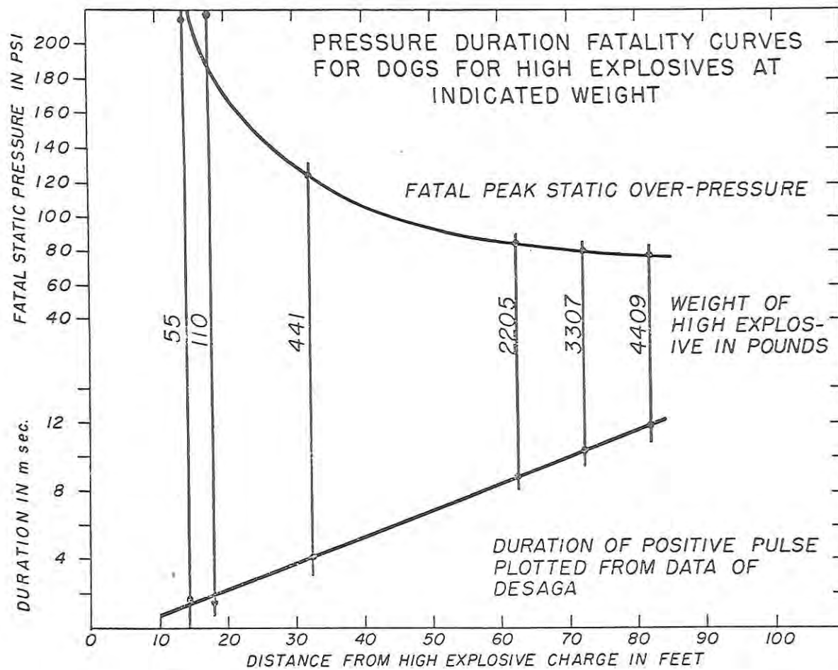
Figure 1. --Fatal overpressure-time conditions for dogs exposed to blast waves produced by high explosives. Plotted from the data of Desaga (Reference 39).
