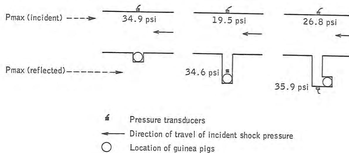
Figure 12. --Maximal incident and reflected overpressures associated with 50-percent lethality over 24 hours in guinea pigs as a function of exposure geometry. From Richmond et al. (Reference 70) and White et al. (Reference 4).
