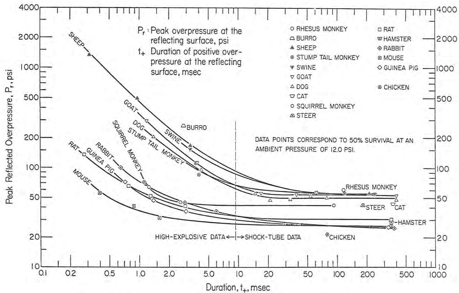
Figure 3.--Pressure-duration curves for 50-percent, 24-hour survival when exposure involves "sharp-rising" overpressure. From Fletcher (Reference 59).
