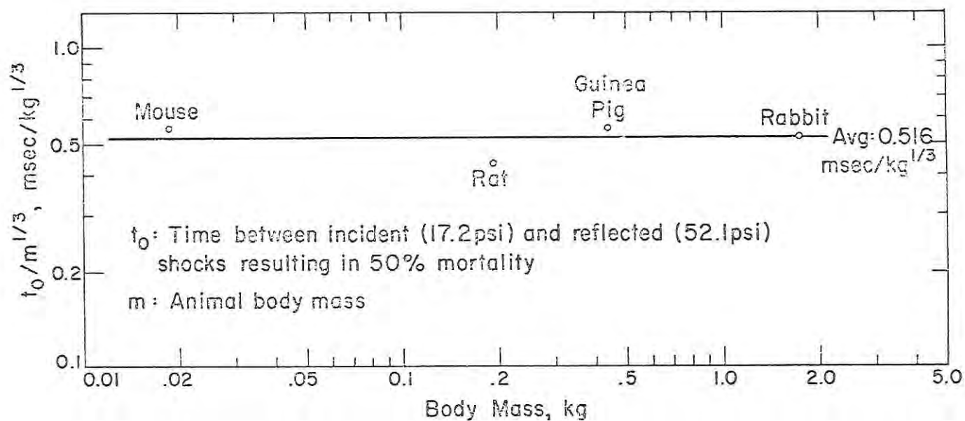
Figure 30.--A test of body-mass scaling for similar animals. The plotted data show that the 4 species of animals have approximately the same sensitivity to time separations of the incident and reflected shocks which are proportional to the cube root of body mass. Data from Richmond et al. (Reference 72). After Bowen et al. (Reference 77).
