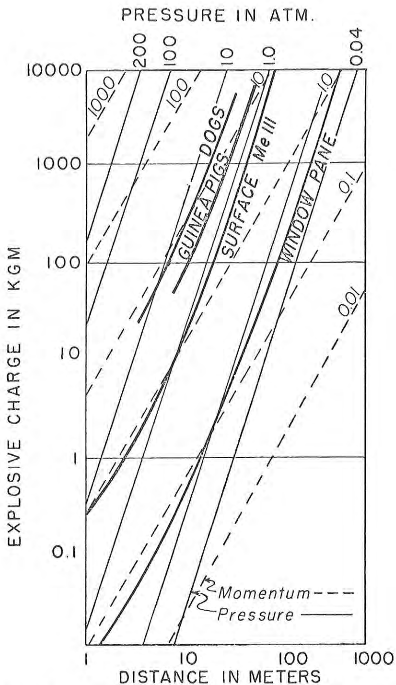
Figure 2. --Charge-distance diagram showing characteristic lines of destruction for dogs, guinea pigs, aircraft surfaces, and windowpanes. Solid and broken lines show pressure in atmospheres and momentum in atmosphere-milliseconds, respectively. Modified from Schardin (Reference 42).
