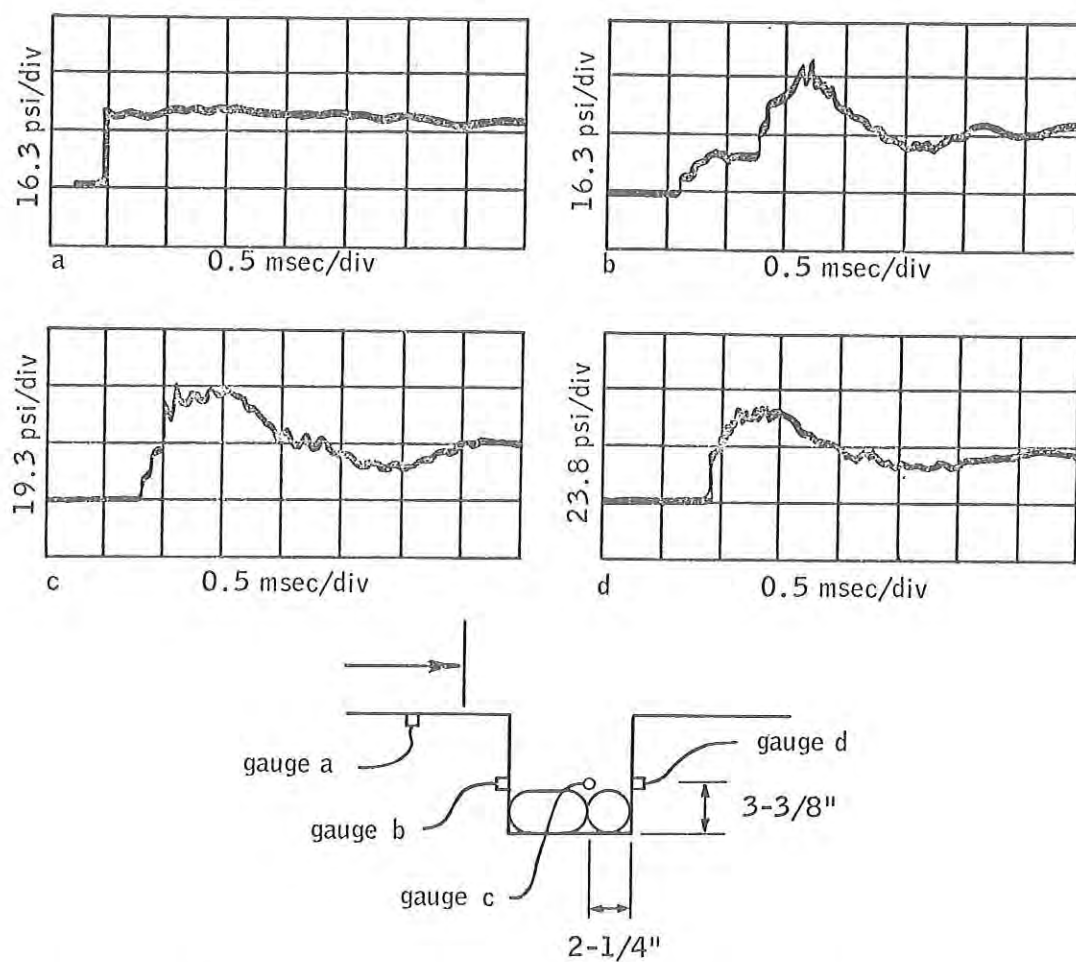
Figure 13. --Pressure-time records associated with the deep chamber. From Richmond et al. (Reference 70).
