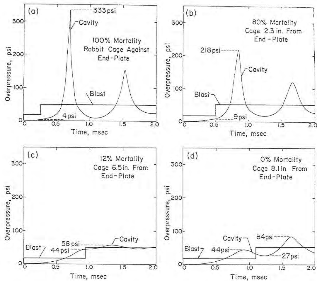
Figure 28. --Computed intrathoracic overpressure versus time for 1.7-kg. rabbits exposed at various distances from the end plate of a shock tube. The incident and reflected shocks were 17.2 and 52.1 p.s.i., respectively. Mortality data from Richmond et al. (Reference 72). After Bowen et al. (Reference 77).
