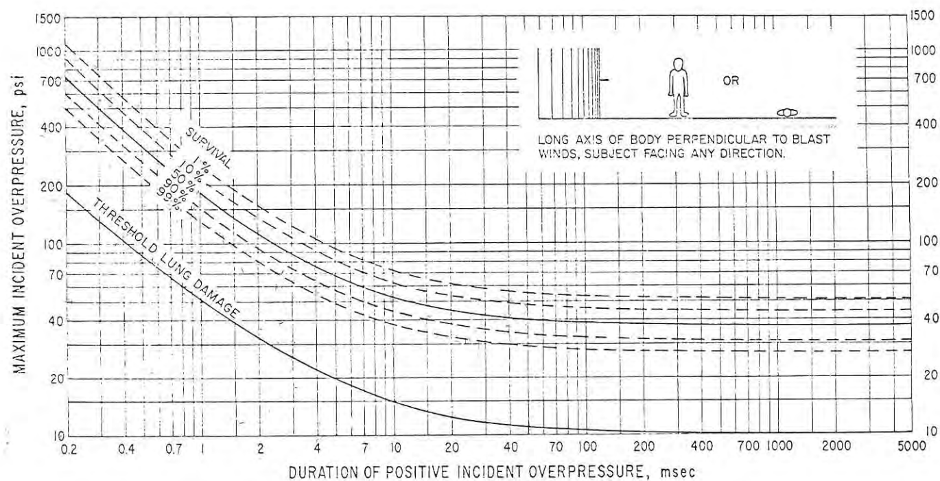
Figure 35.--Survival curves predicted for 70-kg. man applicable to free-stream situations where the long axis of the body is perpendicular to the direction of propagation of the shocked blast wave. After Bowen et al. (Reference 94).
