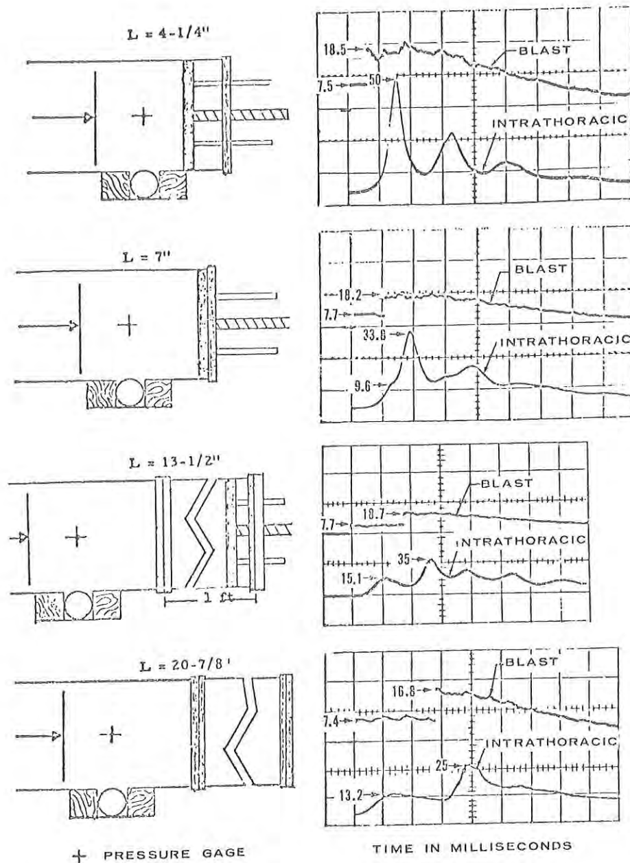
Figure 29.--Incident and reflected blast-pressure pulses and intrathoracic pressure-time responses recorded in guinea pigs with an intraesophageal transducer. Data, courtesy of Mitchell and Gaylord, obtained under the direction of Jones and Richmond (Reference 93); results also used in a recent study by Fletcher (Reference 59).
