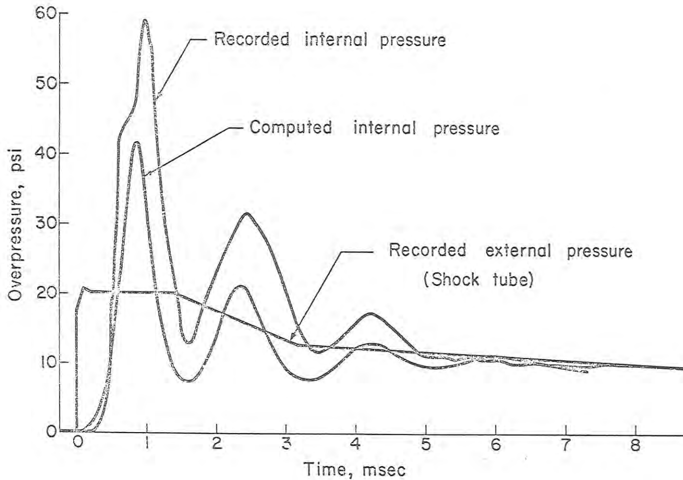
Figure 21. --Comparison of computed and recorded internal pressure-time curves for a rabbit exposed in a shock tube to a 20-p.s.i., "long-duration" pressure pulse. The internal transducer was located in the esophagus near the level of the heart. After White et al. (Reference 83).
