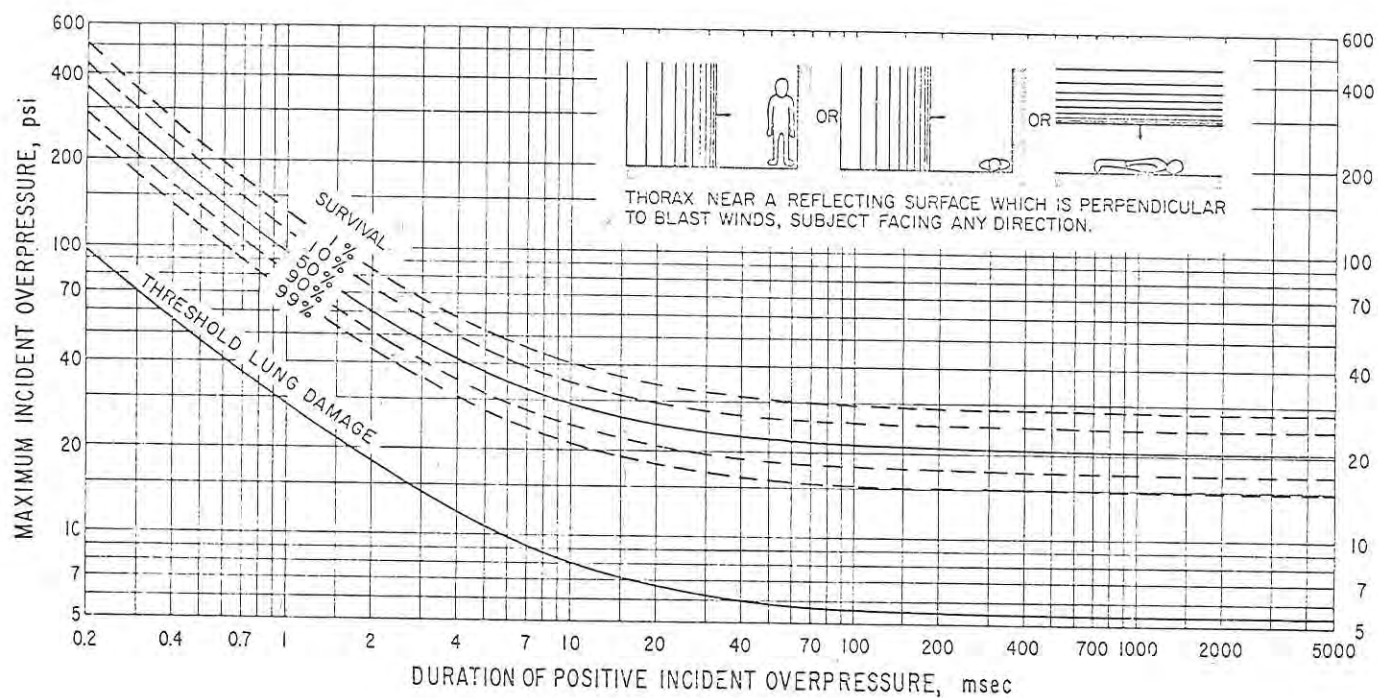
Figure 36.--Survival curves predicted for 70-kg. man applicable to blast situations where the thorax is near a surface against which a shocked blast wave reflects at normal incidence. After Bowen et al. (Reference 94).
