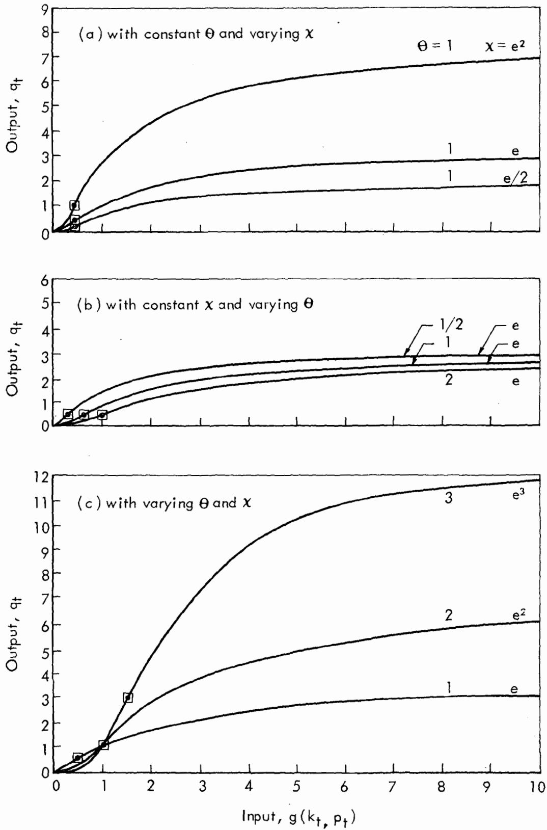
Fig.8 — Plot of the production function q_t = \chi e^{-\theta g(k_t, p_t)}
