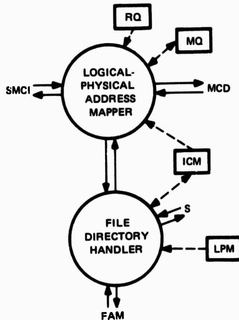
Figure 3.14 - LPAM Module
