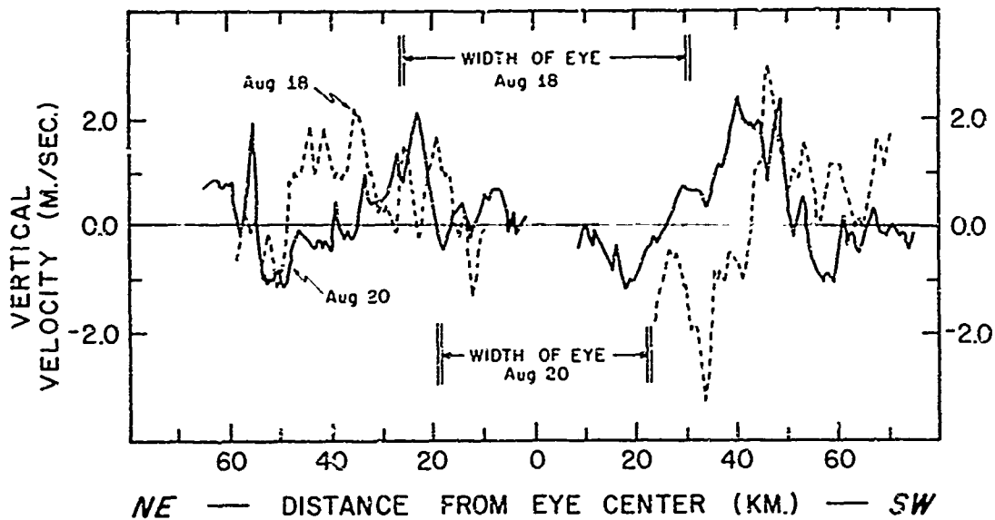
Figure F-1. Composited vertical velocity profile for Hurricane Debbie as determined from the RFF 39-C DC-6 aircraft. The profile represents an average of 8 radial legs on 20 August 1969, and 5 radial legs on 18 August, which were on a northeast-southwest azimuth. Compositing was done with respect to the inner face of the eyewall cloud, the mean positions of which are indicated by the width of the eye.
