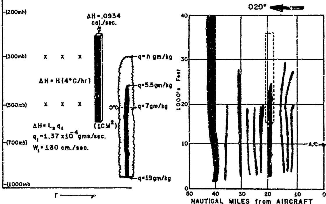
Figure B-2. Radar echoes from the original picture reproduced in Fig. 1 are in the right side of the diagram. The center of Hurricane Debbie was about 50 n miles north-northwest of the aircraft. The eyewall (40 n miles from aircraft) extended higher than 40,000 ft (limit of the radarscope). The left portion refers to calculations of amount of heat that can be released by seeding and to the amount of heat required for modification of a hurricane in the simulation experiment with a theoretical model (see text).
