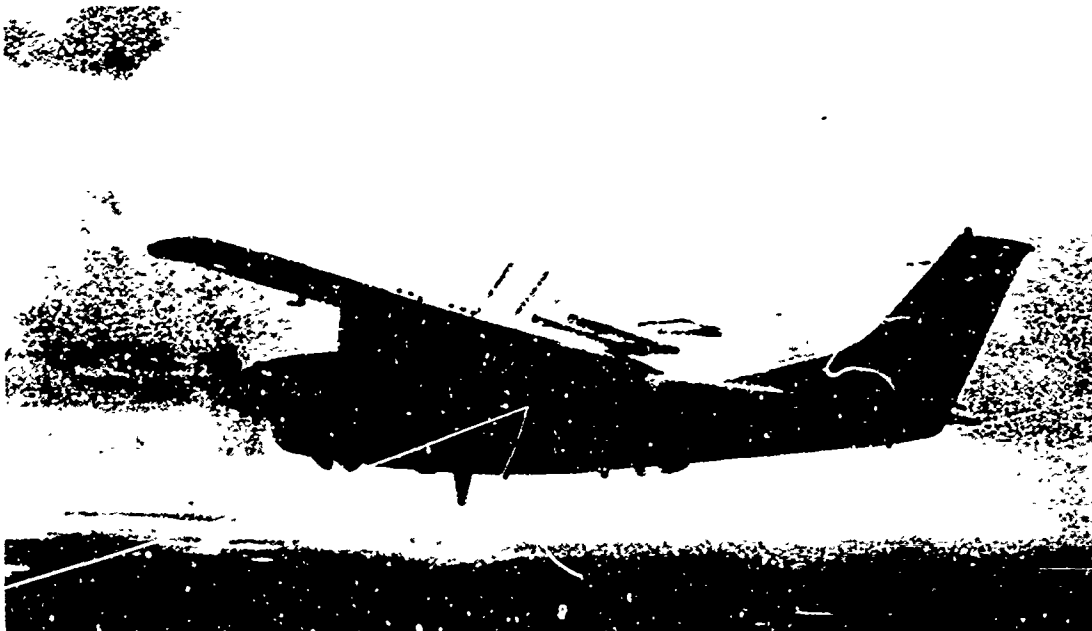
Figure I-1. Navy-leased Cessna 210(77R). Streamlined rack for STORMFURY type air-dropped flares on port wing, boom for burn-in-place flares on starboard wing.
