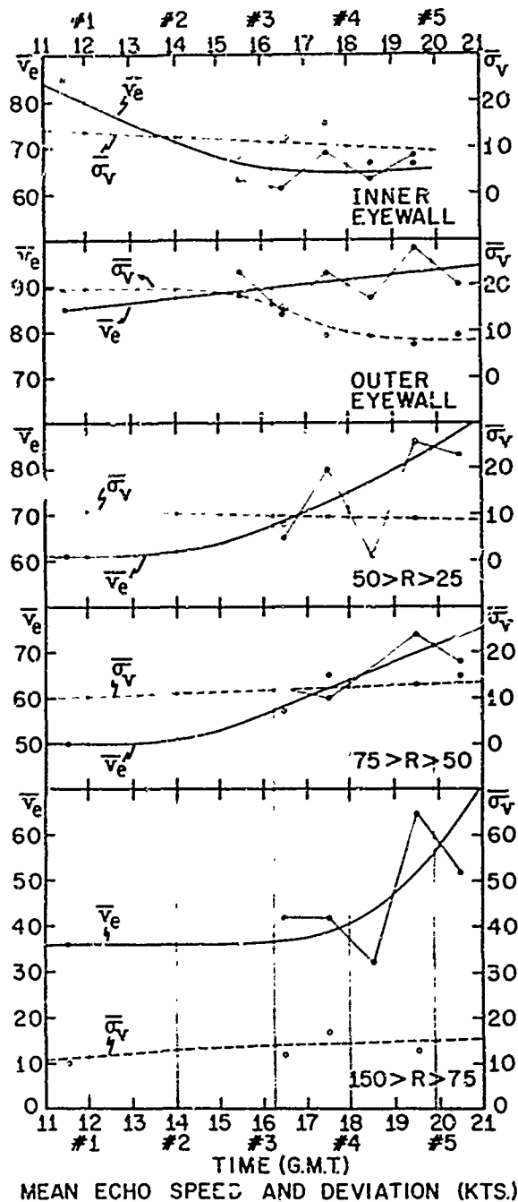
Figure J-6. Azimuthally averaged echo speeds at selected range intervals together with the mean maximum deviations about the azimuthal mean. Scale for the mean values (solid circles) is on the left and the scale for the deviations (open circles) is on the right. The thin vertical lines indicate the seeding times.
