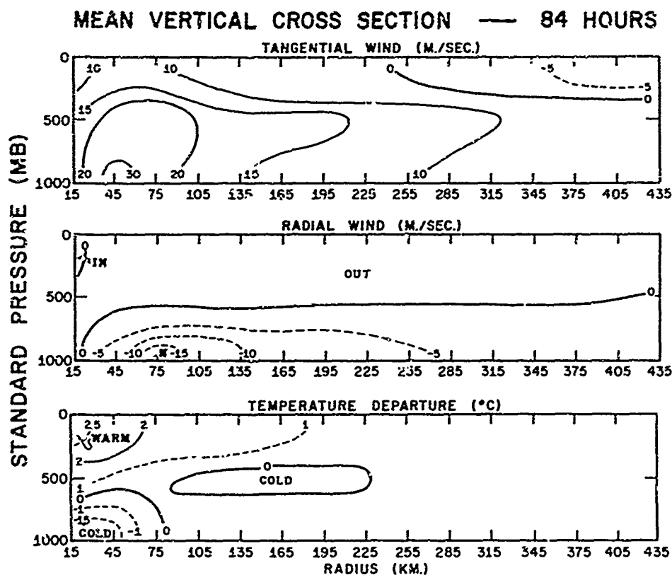
Figure D-5. Azimuthal mean vertical cross sections for the tangential wind, the radial wind, and the temperature anomaly at 84 hours. Isotherms are labeled in °C; isotachs are labeled in m\ sec^{-1} .
