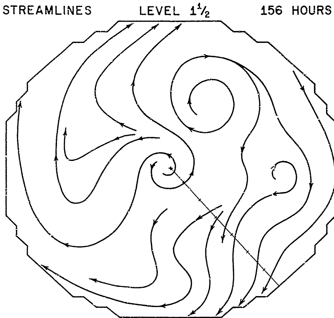
Figure D-7. Streamline analysis for the upper troposphere (level 1½) at 156 hours.
