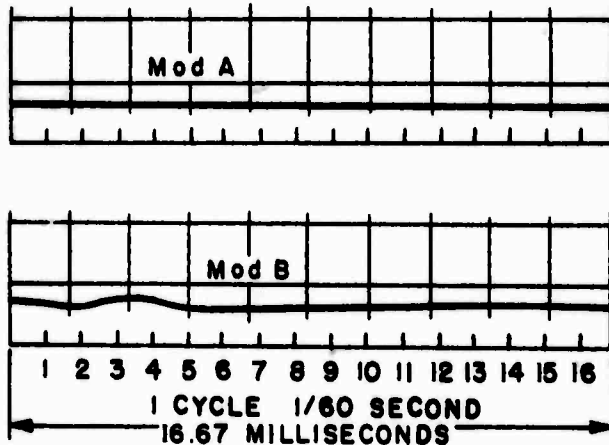
TRACES I and J: These traces show no firing pulse from Module A as well as Module B. This type of trace is associated with a series of tests of other components, see paragraphs 3.G.c., and f.
