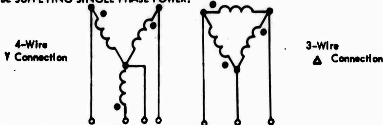
TWO STYLES OF SATISFACTORY SET-UPS - COILS SHOWN ARE SECONDARY COILS OF THREE POWER COMPANY TRANSFORMERS. PRIMARIES ARE NOT SHOWN.
