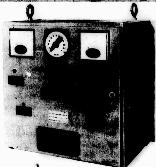
Model US-50-1-6 Charger, door closed
