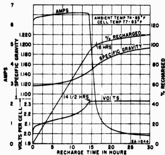
Fig. 4. Recharge characteristic of 6-ampere charger with an equalize setting of 2.33 volts per cell (100 A.H. battery discharged at 8-hour rate to 100 A.H.)
