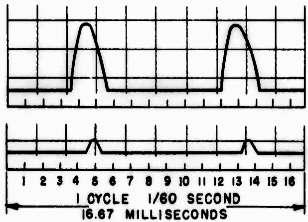
Fig. 13. Traces showing normal condition of charger output current. (Trace A is for rated charger current. Trace B is for about 10% rated charger current.)
