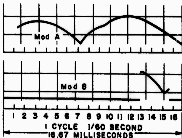
TRACES G and H: These traces show a satisfactory firing pulse from Module B, but an unsatisfactory pulse from Module A. Replace Module A, it is at fault.
