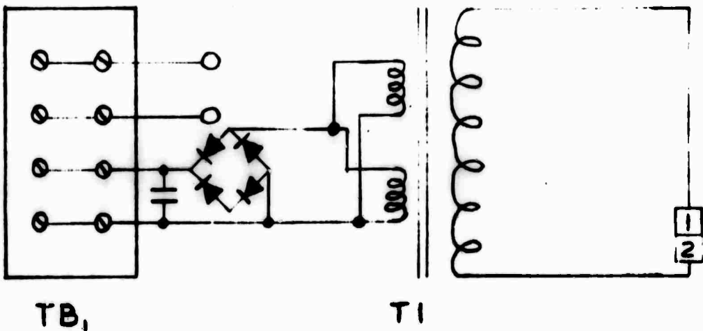
POWER SUPPLY
