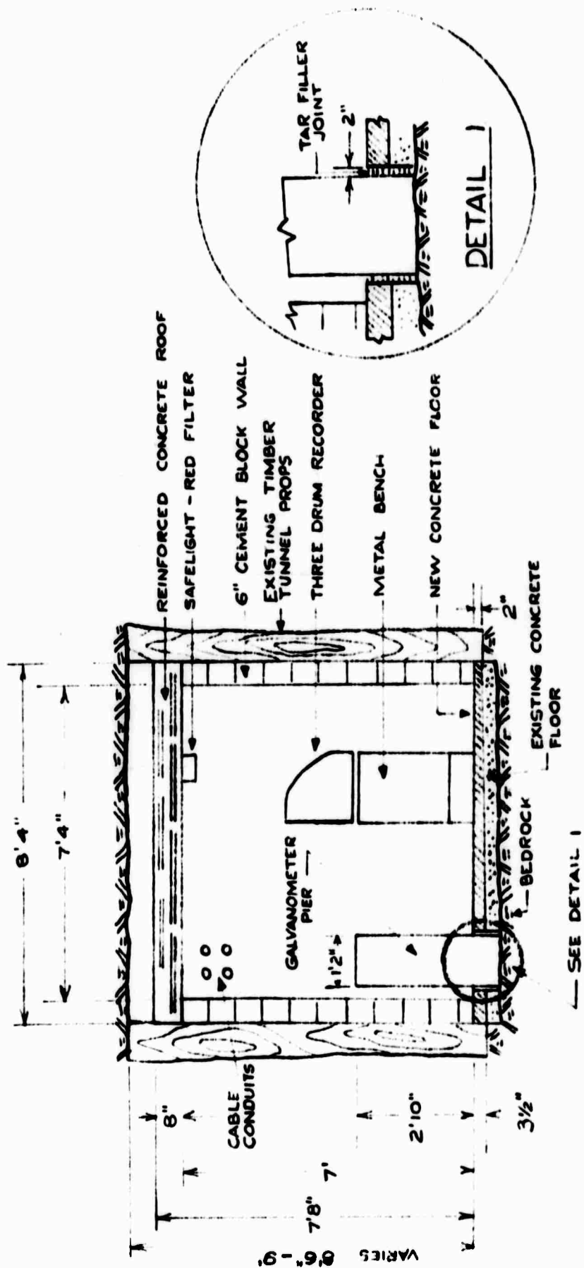
Figure II-10: Cross-sectional view of Recorder Room.
