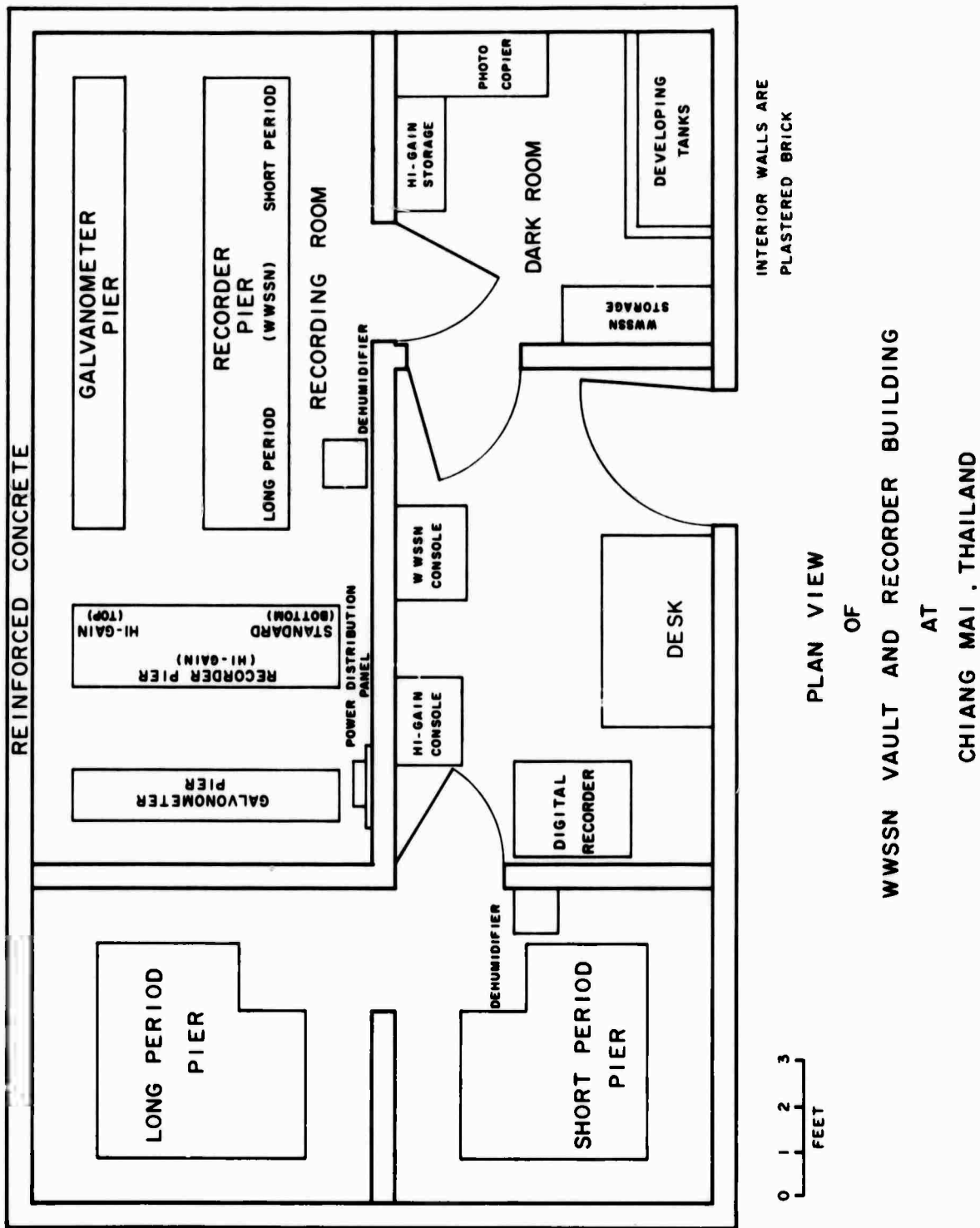
Figure II-5: Plan of existing WSSN Vault and Recording Building.
