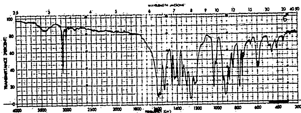
High Explosive 1 RDX (Cyclotri- methylene trinitramine)
