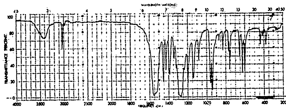
High Explosive 2 HMX (Cyclotetra- methylene trinitramine)
