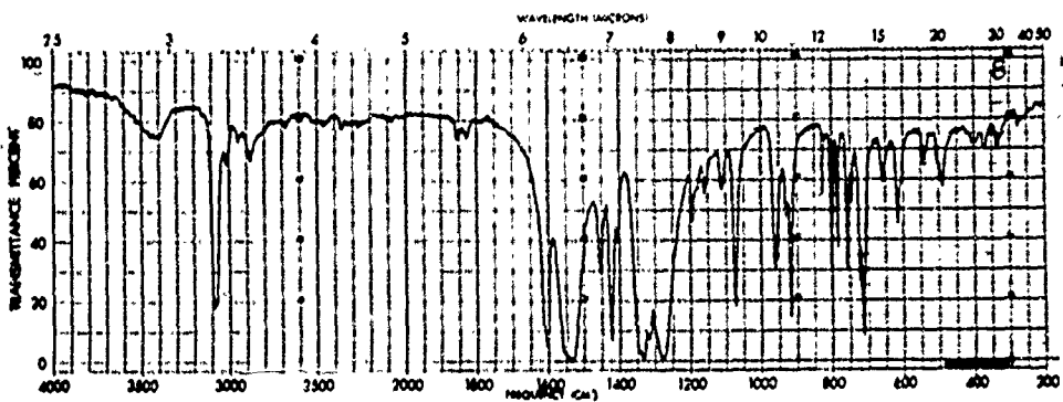
High Explosive 3 Tetryl (2,4,6-Trinitro- phenylmethyltriamine)
