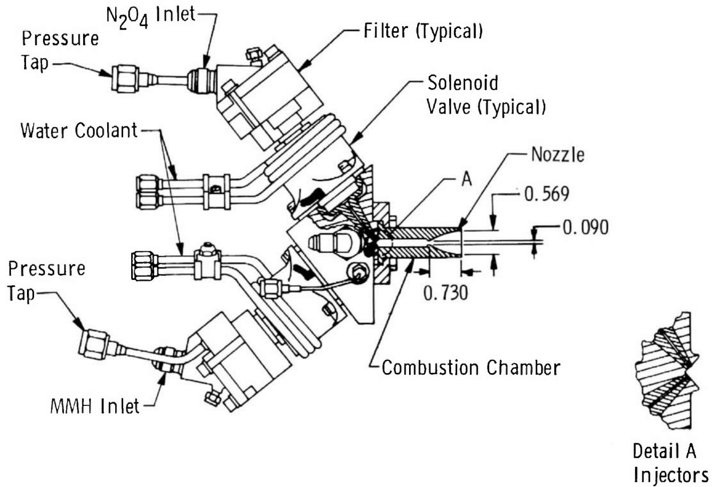
Fig. 18 One-Pound-Thrust Engine and Valves
