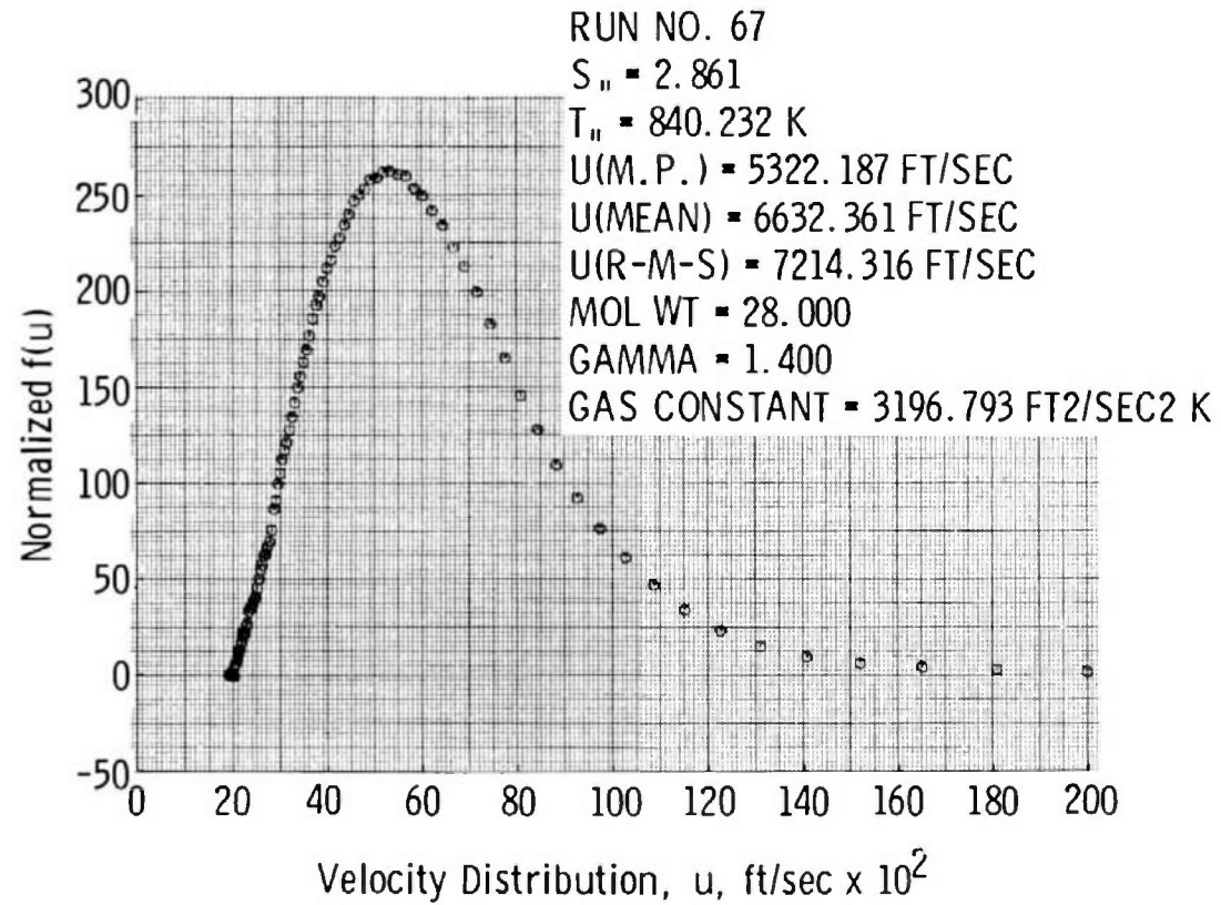
b. Velocity Distribution Fig. 34 Concluded
