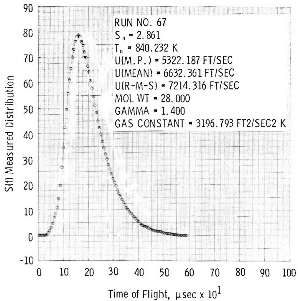
Fig. 34 Nitrogen Time-of-Flight and Velocity Measurement for Hot Thruster Firing, U_{mp} = 5322 \text{ ft/sec}
