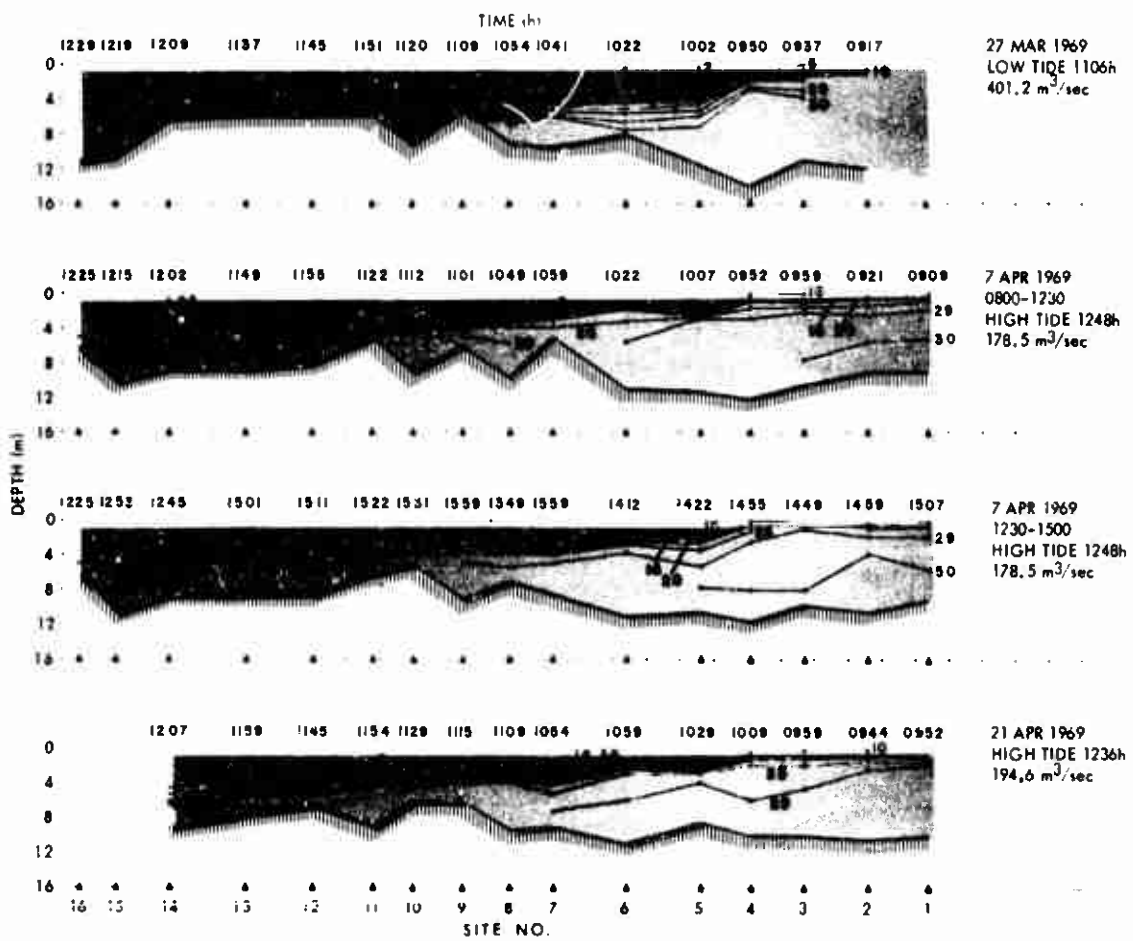
Fig. 11. Salinity Profiles of the Thames River for 27 March and 7 and 21 April 1969
