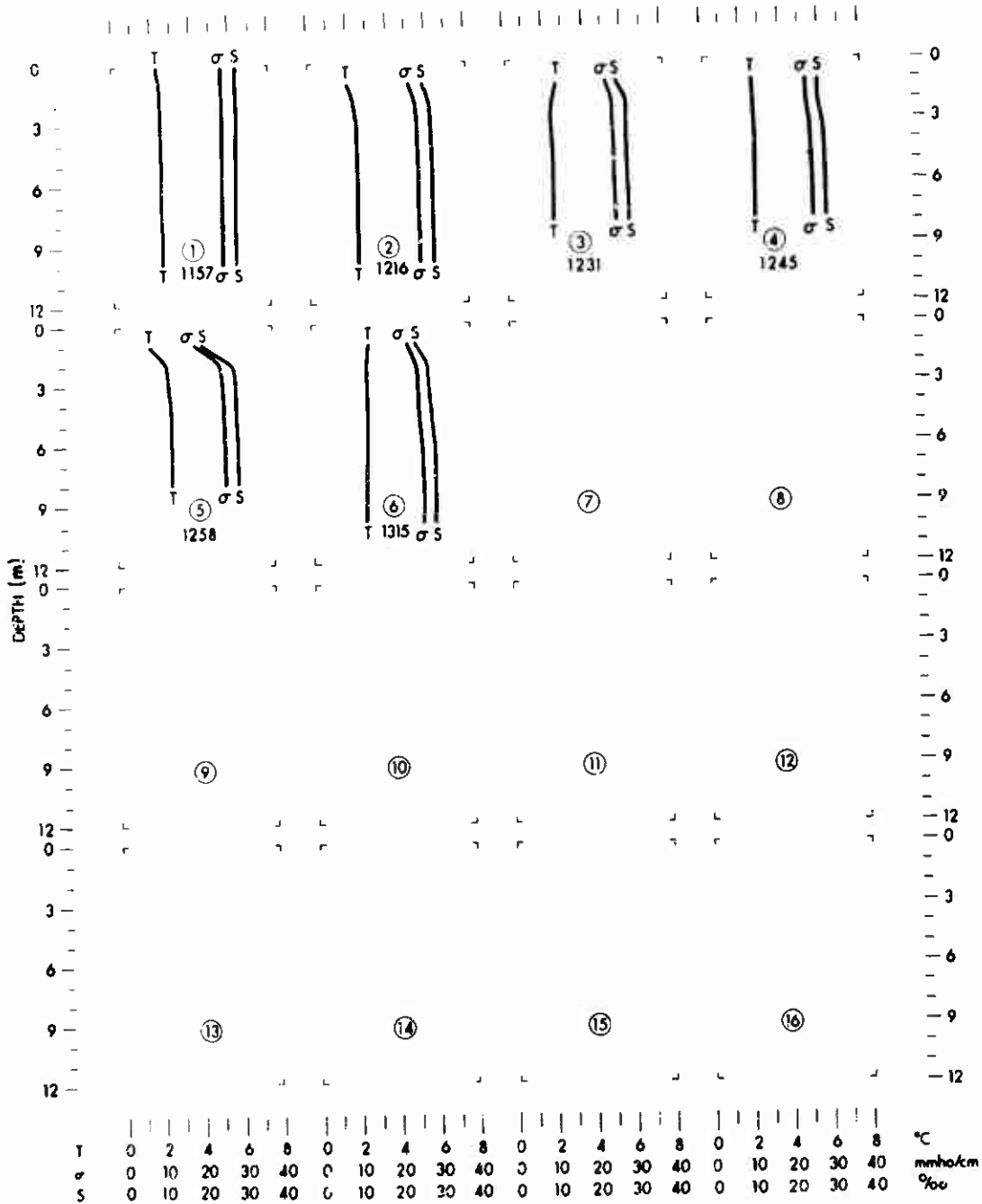
Fig. A.11. Conductivity, Temperature, and Salinity Profiles for 9 January 1969
