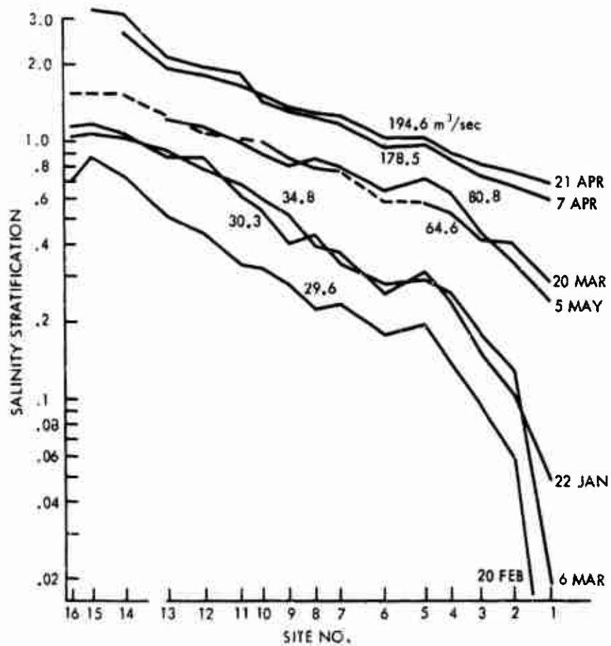
Fig. 13. Salinity Stratification as a Function of Location along the Thames River: Selected Curves of Data Taken during Periods of Flooding and High Tide. (The number beside each curve is the rate (in cubic meters per second) of freshwater discharge for the combined readings of the three stations averaged over the two days preceding the date of measurement.)
