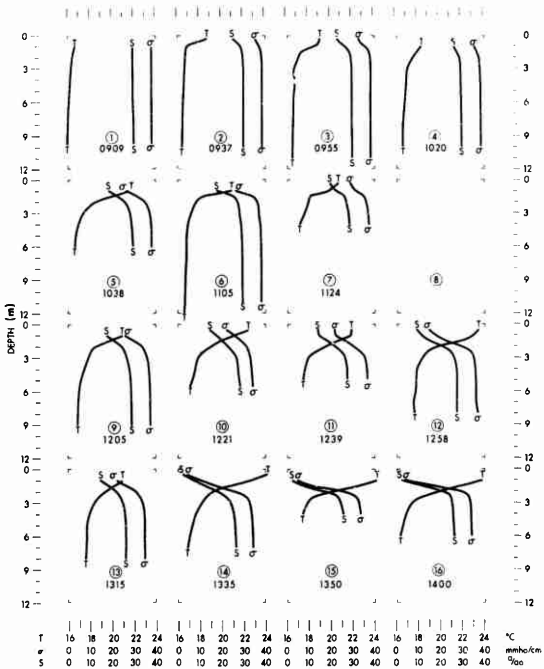
Fig. A-2. Conductivity, Temperature, and Salinity Profiles for 12 July 1968
