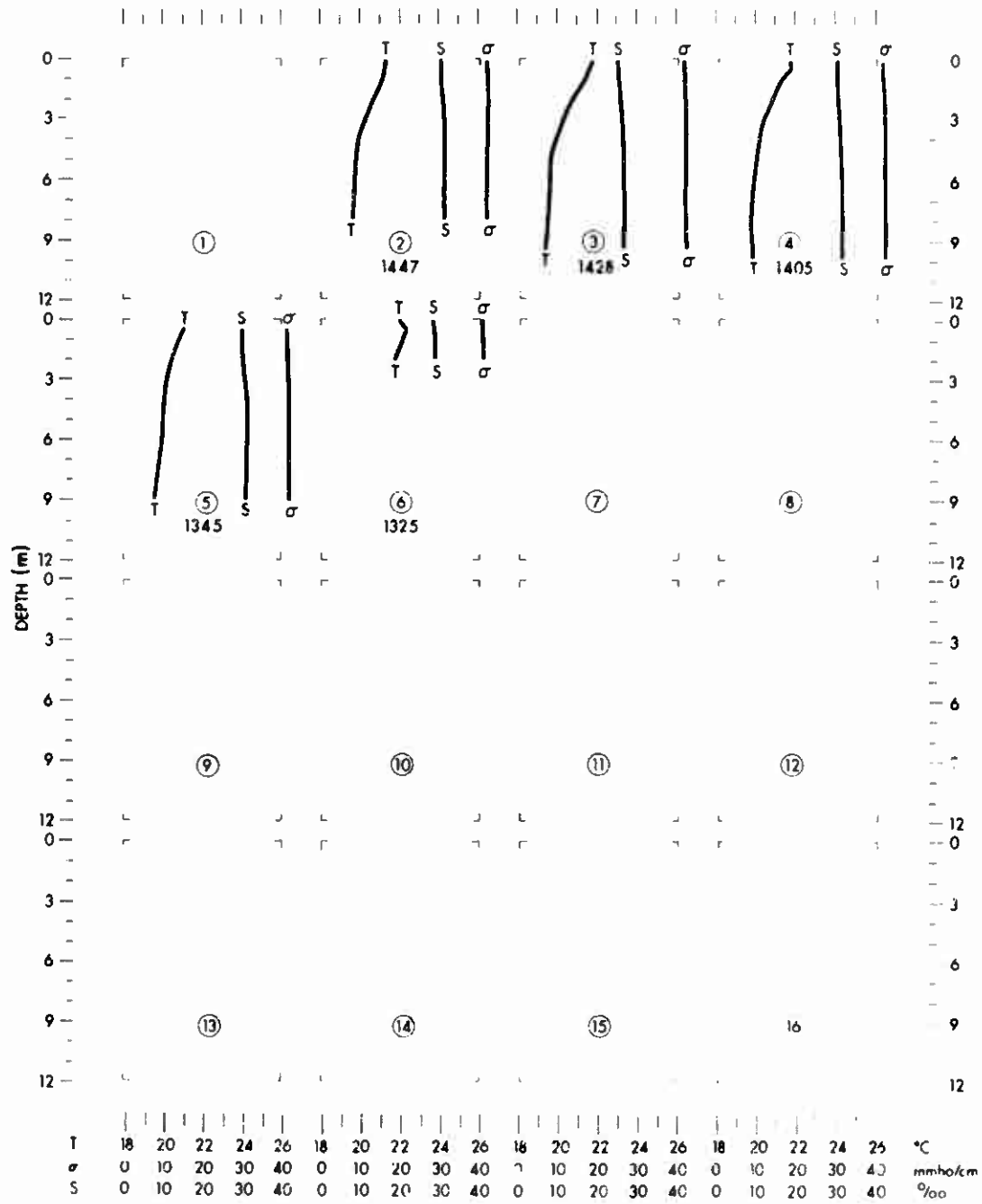
Fig. A-6 Conductivity, Temperature, and Salinity Profiles for 26 September 1968
