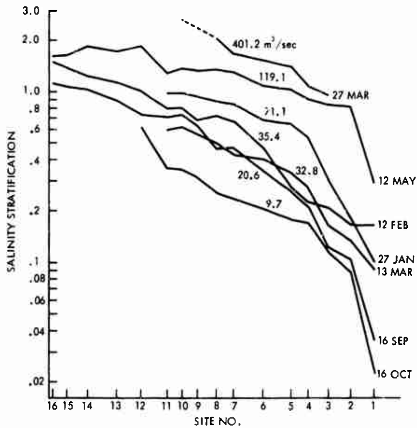
Fig. 14. Salinity Stratification as a Function of Location along the Thames River: Selected Curves of Data Taken during Periods of Ebbing and Low Tide. (The number beside each curve is the rate (in cubic meters per second) of freshwater discharge for the combined readings of the gaging stations averaged over the two days preceding the date of measurement.)
