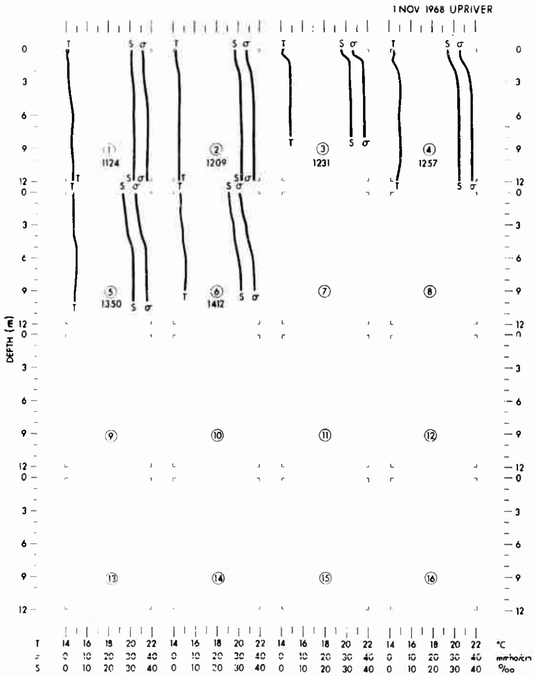
Fig. A-9. Conductivity, Temperature, and Salinity Profiles for 1 November 1968, Upriver
