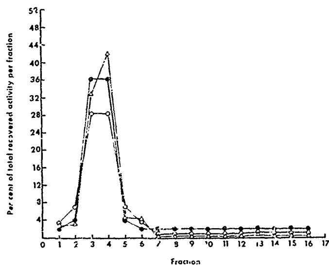
FIG. 1. Rate zonal centrifugation of VEE virus in a sucrose gradient: (Δ), infectivity; (○), hemagglutination; (◼), complement fixation.
