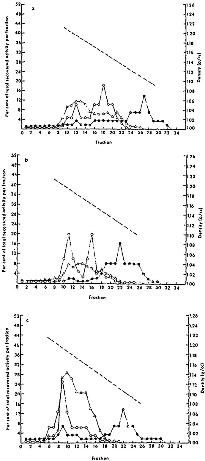
FIG. 3. Isopycnic centrifugation of WN (a), ILH (b), and RB (c) viruses in sucrose gradients: ( \Delta ), infectivity; ( \circ ), hemagglutination; ( \bullet ), complement fixation; (---), g/cc.
