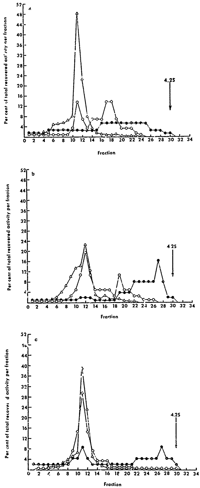
FIG. 2. Rate zonal centrifugation of WN (a), ILH (b), and RB (c) viruses in sucrose gradients: ( \Delta ), infectivity; ( \circ ), hemagglutination; ( \bullet ), complement fixation.
