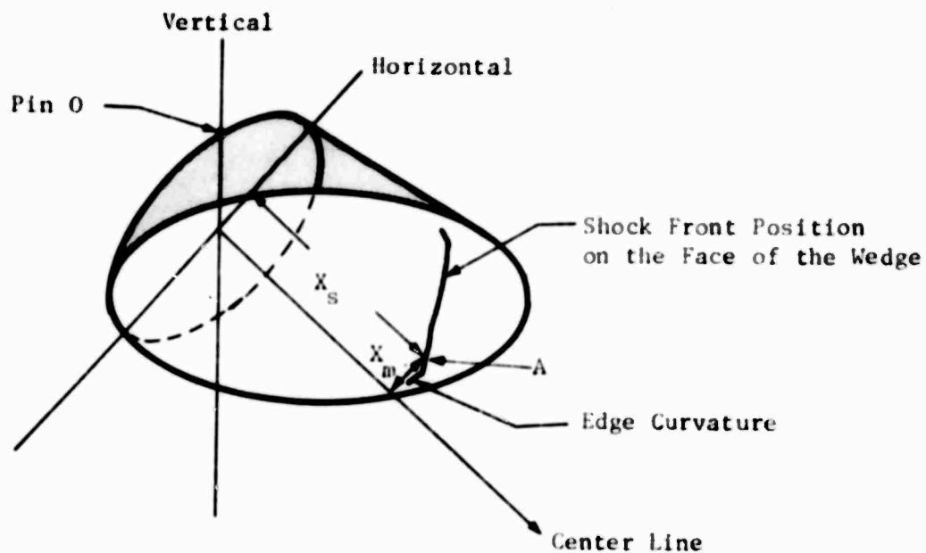
Figure 34: Wedge Geometry
