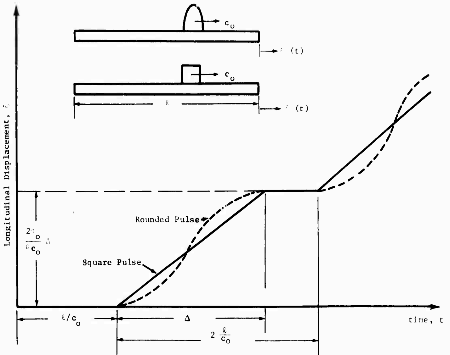
Figure 18. End Displacement, \xi , for a Rectangular Compression Pulse
